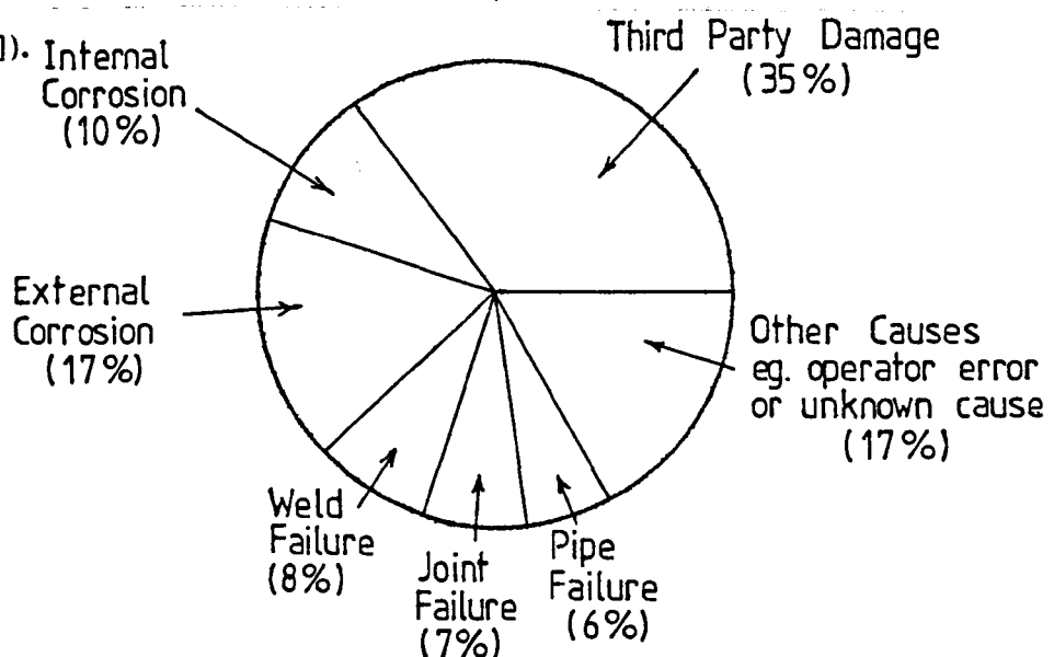
Figure 1.2. Pipe Failure Distribution for Natural Gas Lines
