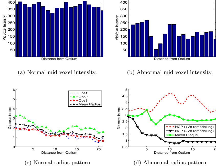
Figure 9: Graphical representation for segment representative features. (a, c) defines mid-lumen intensity and radius trend for normal segments, whereas (b, d) represents the abnormal segment. It can be observed that normal segments are characterized with high mid-lumen intensity and smooth decreasing radius, whereas abnormal segment is related with low mid-lumen intensity and often suffers with unexpected radius variations (+ve, -ve and hybrid vessel remodelling).
