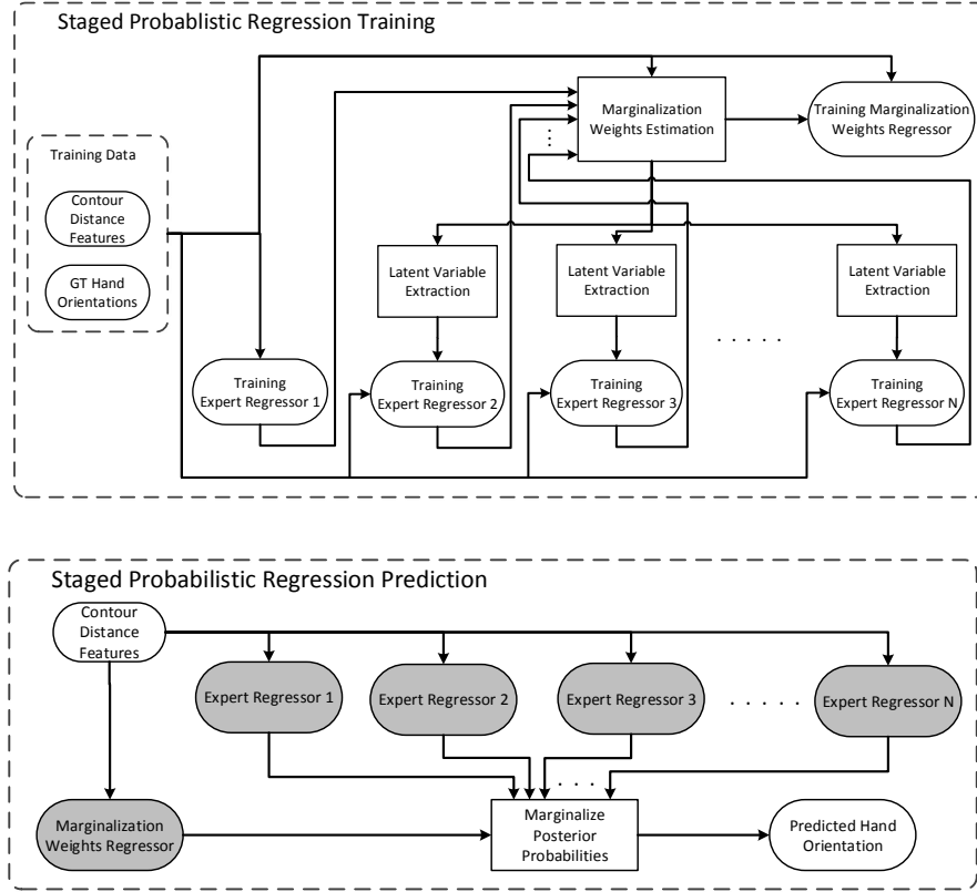
Fig. 6.1 Flowchart shows the SPOR training and prediction framework. The trained regressors are highlighted with a solid gray background.
