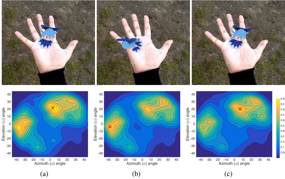
Fig. 5.13 Augmented Reality application sequence with a failure case. Top row shows the rendered augmented character on a continuous sequence of input images, whereas the bottom row shows the posterior probability p(\phi, \psi | \mathbf{d}_k) from our proposed ML-RF MtR method. The MLE prediction is shown as a red x. It can be seen in (b) that even when our method fails, the posterior probability contains information for correct orientation angles.
