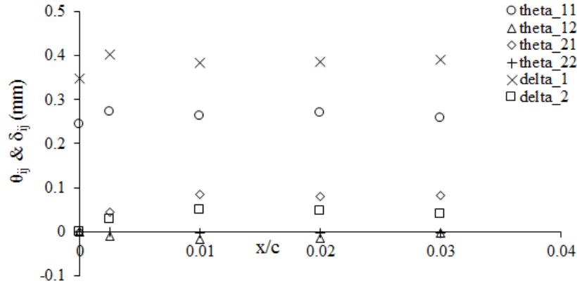
Figure 12: The port side streamwise and crossflow integral quantities in the vicinity of the AL at Re = 590 .
