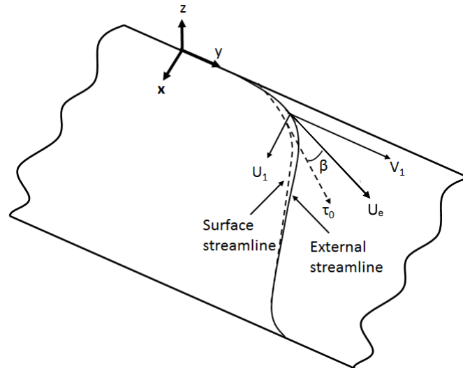
Figure 1: Schematic representation of the flow along a swept wing.
