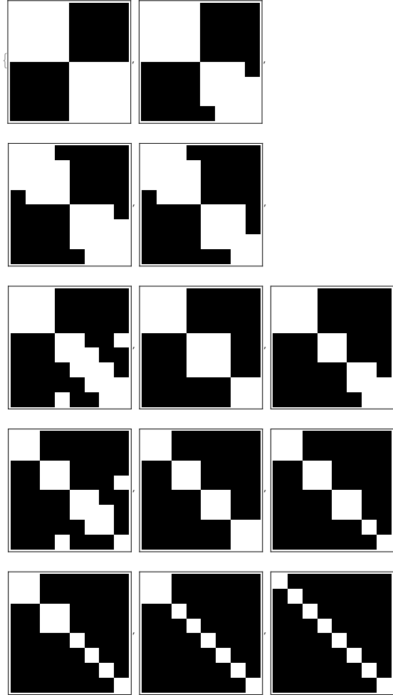
FIGURE 7.7: Analysis for maximum graphs for n = 8, m \geq 16 .
