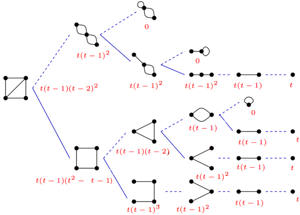
FIGURE 2.1: An example of obtaining the chromatic polynomial for K_4 - e via the deletion-contraction method. Source: Peter Kaski 2008 (with edits and corrections)
