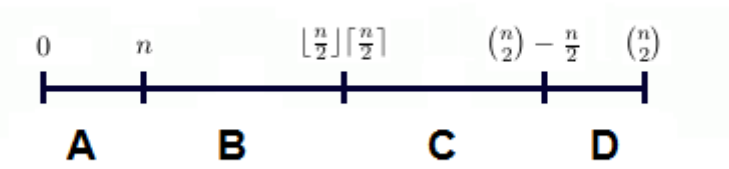
FIGURE 7.1: A summary of our knowledge on the maximum with respect to the number of edges. For sections A and D we know the maximum and have proved what it is. For C we have a good idea about the structure, and for B we have the least idea of what the graphs look like.
