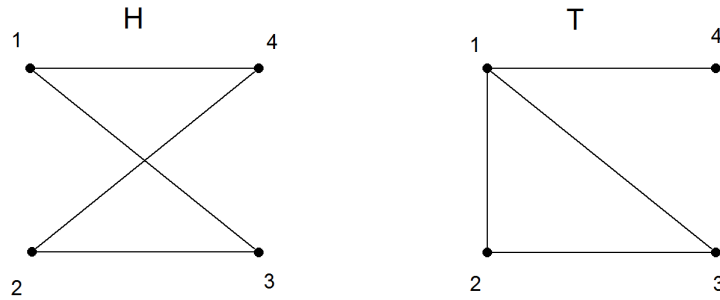
FIGURE 7.17: The labels of the graph H and T
