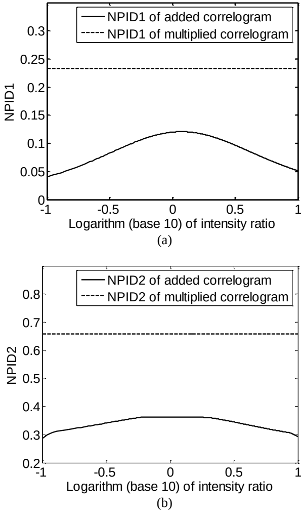
Fig. 5. (a) NPID1 varying with the logarithm of the intensity ratio (b) NPID2 varying with the logarithm of the intensity ratio. Coherence length: 7.0 \mu\text{m} ; two wavelengths: 0.78 \mu\text{m} and 0.67 \mu\text{m} .
