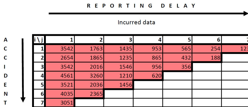
FIGURE 1.2: Example incurred triangle, aggregated by accident year and reporting delay.
