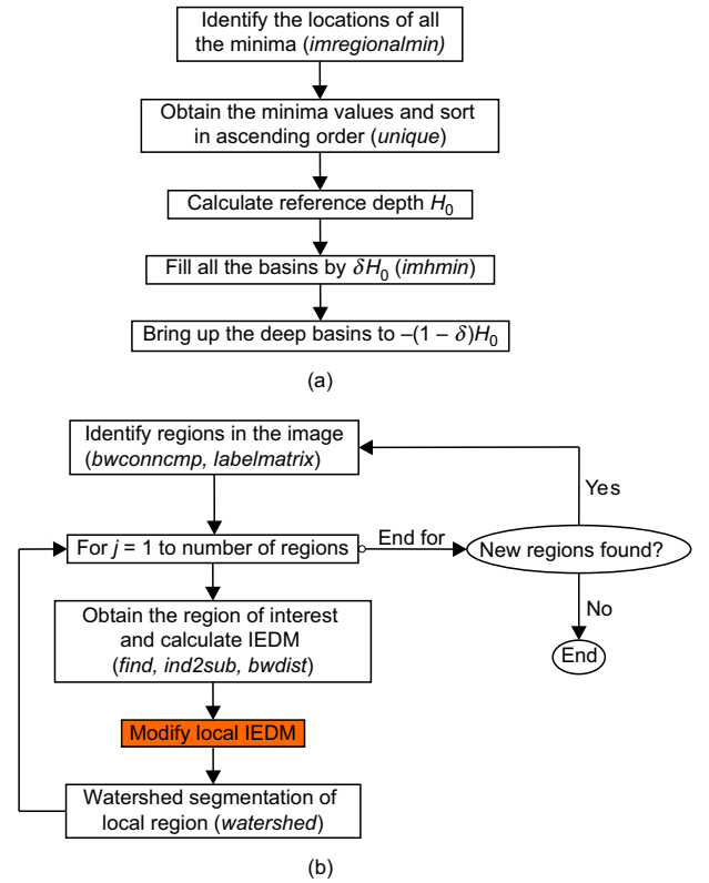
Fig. 4. Scheme of the adaptive bring-up watershed segmentation technique: (a) modification of IEDM; (b) overall process
