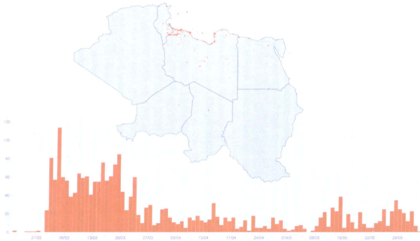
Figure 5.4: Overview of the software prototype that was developed to evaluate the suitability of D3/JavaScript. The map and the temporal histogram depict reports from the Libya crisis map (OCHA 2011). One bar on the temporal histogram represents 24 hours.
