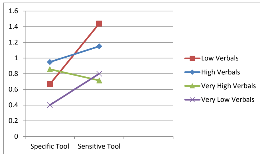
Figure 4-11: Average False Positives of User+Tool System in Easy Passages Each line represents the performance of a certain user group when using the specific versus sensitive tool. Overall, when editing easy passages, all user groups, except Very High Verbals, changed more correctly spelled words when using the sensitive tool compared to when using the specific tool.
