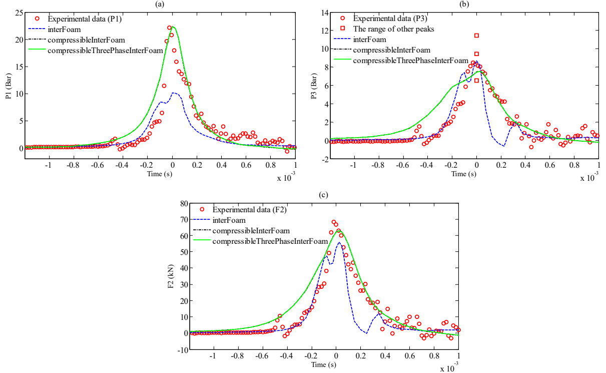
Figure 6.7 The comparison between the experimental and numerical results in terms of (a) P1, (b) P3 and (c) F2 for the case with V_{\text{impact}}=5\text{m/s} and m_{\text{plate}}=32\text{kg} .
