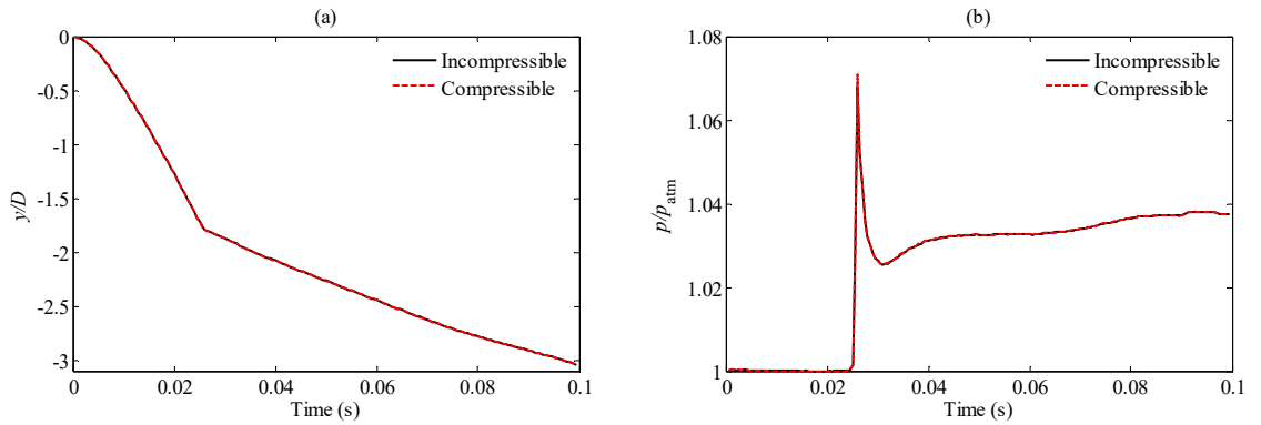
Figure 6.9 Time history of (a) the location of the tip of the oil jet and (b) the pressure on the tip in the transient stage of Case G1. ( y axis origins from the bottom of the internal hole)
