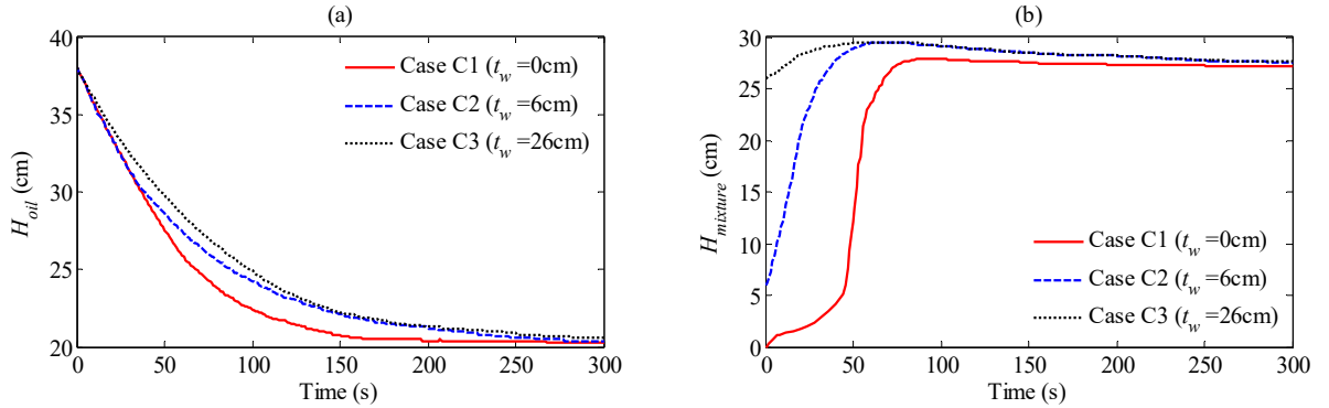
Figure 3.20 Time histories of (a) oil height in the cargo tank ( H_{oil} ) and (b) the oil-water mixture height in the ballast tank ( H_{mixture} ) for collision cases.
