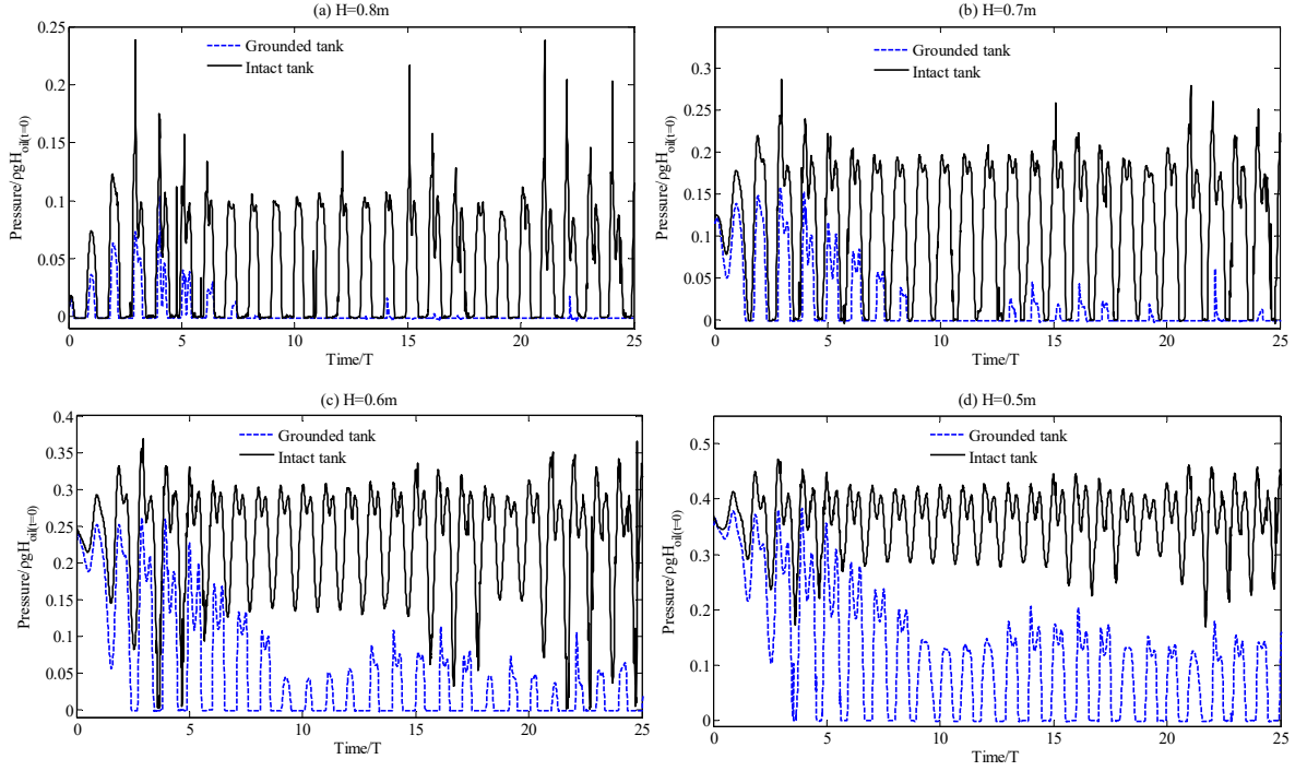
Figure 8.9 Time histories of the pressure on the left side wall at the height of (a) H=80\text{cm} , (b) H=70\text{cm} , (c) H=60\text{cm} and (d) H=50\text{cm} from the tank bottom in Case G6 and G6i. (Sway motion: \omega_1=5.5\text{ rad/s} and A=0.02\text{m} )
