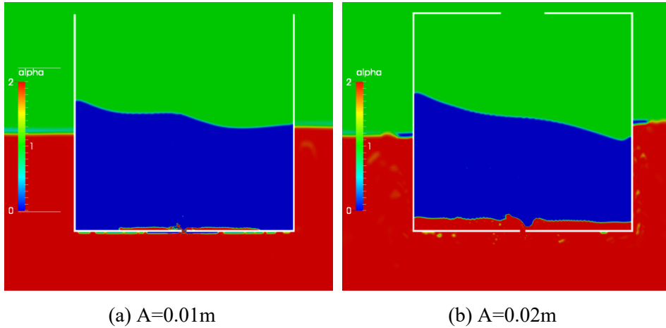
Figure 8.16 Snapshots of the spatial distributions of oil, water and air (volume of fraction \alpha ) at 175T (water: red ( \alpha=2 ); air: green ( \alpha=1 ); oil: blue ( \alpha=0 ); \omega_1=5.5 rad/s)
