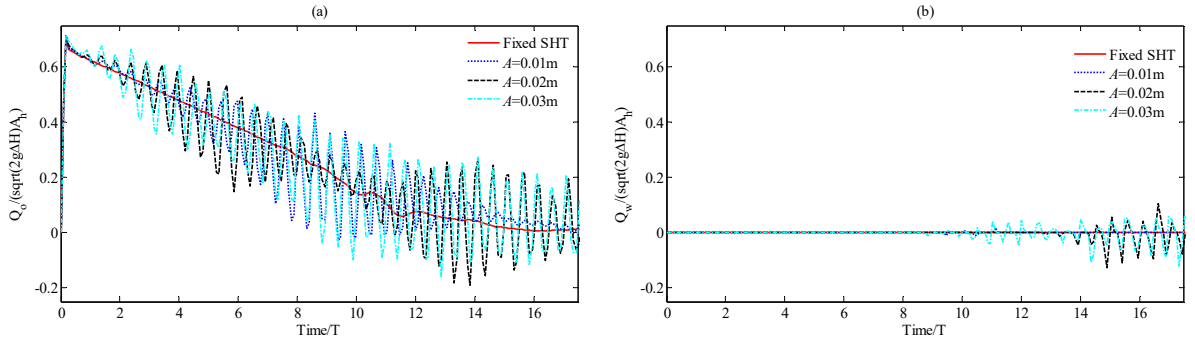
Figure 8.13 Time histories of the discharges of (a) the oil outflow ( Q_o ) and (b) the water inflow ( Q_w ) through the broken hole in the first phase. (forced sway with \omega_I=5.5 rad/s)
