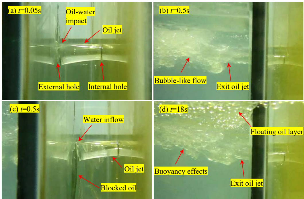
Figure 3.13 Flow states near the puncture at first stage (Case C1).
