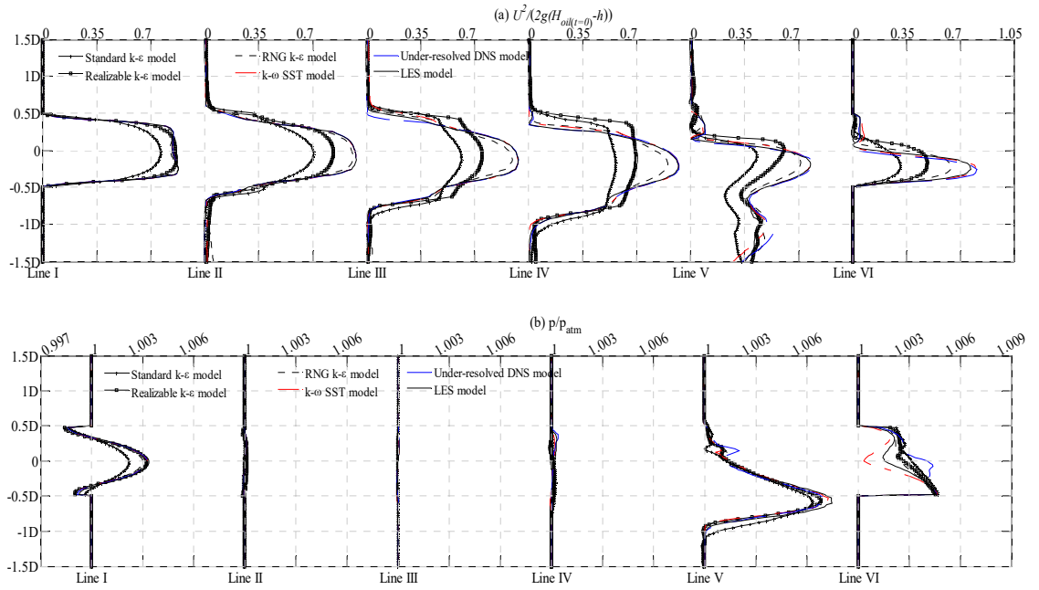
Figure 5.6 Distribution of (a) the normalized velocity head U^2/(2g(H_{oil(t=0)} - h)) and (b) the normalized pressure ( p/p_{atm} ) along the horizontal sampling lines at t/\sqrt{d/g} \approx 12 in the cases with different turbulence modelling in Case C1.
