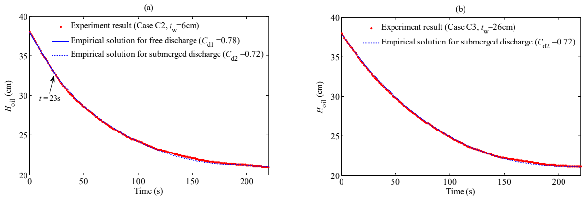
Figure 3.21 The comparison of H_{oil} between the experiment data and the empirical solution for (a) Case C2 ( t_w = 6\text{cm} ) and (b) Case C3 ( t_w = 26\text{cm} ).
