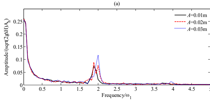
Figure 8.14 Spectrum distribution of the oil discharge ( Q_o ) in the first phase of spilling. (forced sway with \omega_I=5.5 rad/s)
