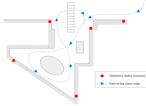
Fig. 5. The testbed plan
