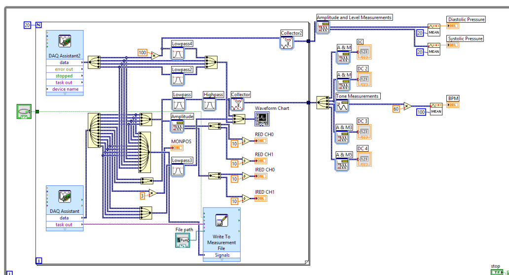
Figure 7-20 LabVIEW Virtual Instrument block diagram used for in vitro experiments.
