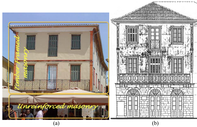
Figure 4. The 'Berykiou' building: (a) the façade and, (b) architectural survey (by Toulaitos and Gante 1995) in the central square of the Lefkas city.
