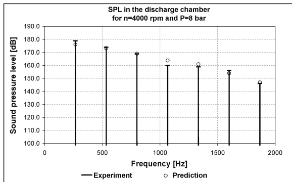
Figure 14. Gas pulsations calculated by coupled model, frequency domain.
