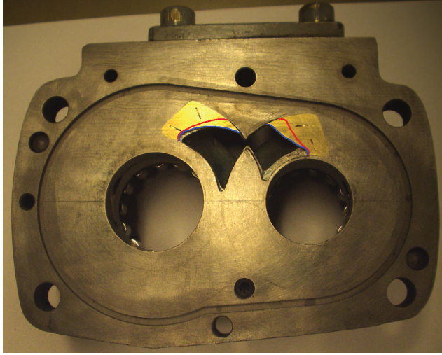
Figure 17. Modified shape of the discharge port.
