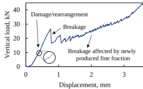
Figure 5. A typical load-displacement curve in the strain controlled test.
