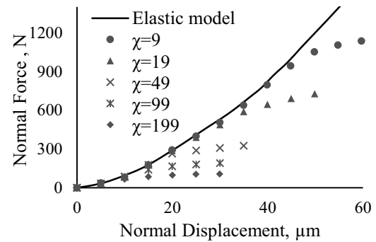
Fig. 2. Response of a spherical grain under compression for different tensile strengths.
