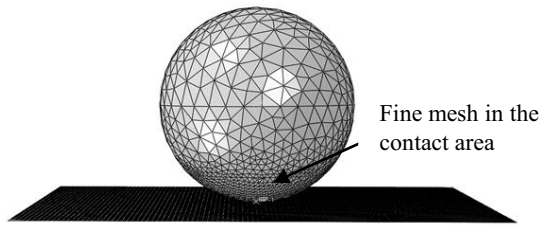
Fig. 4. Meshed sphere in contact with the rigid plate; mesh defined by smaller elements in the contact area.
