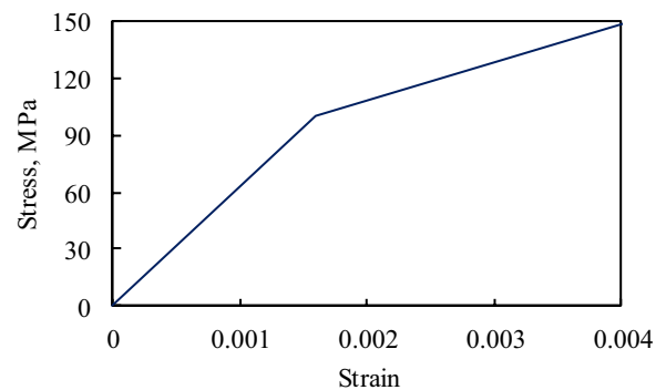
Fig. 6. Stress:strain for isotropic hardening material used in the simulation.
