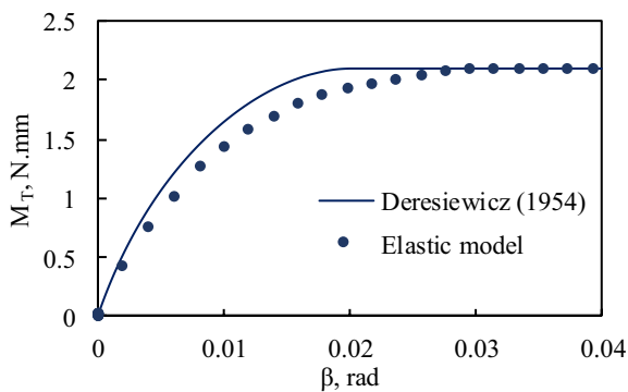
Fig. 5. Comparison between theory and numerical modelling for elastic interaction of two identical elastic spheres.
