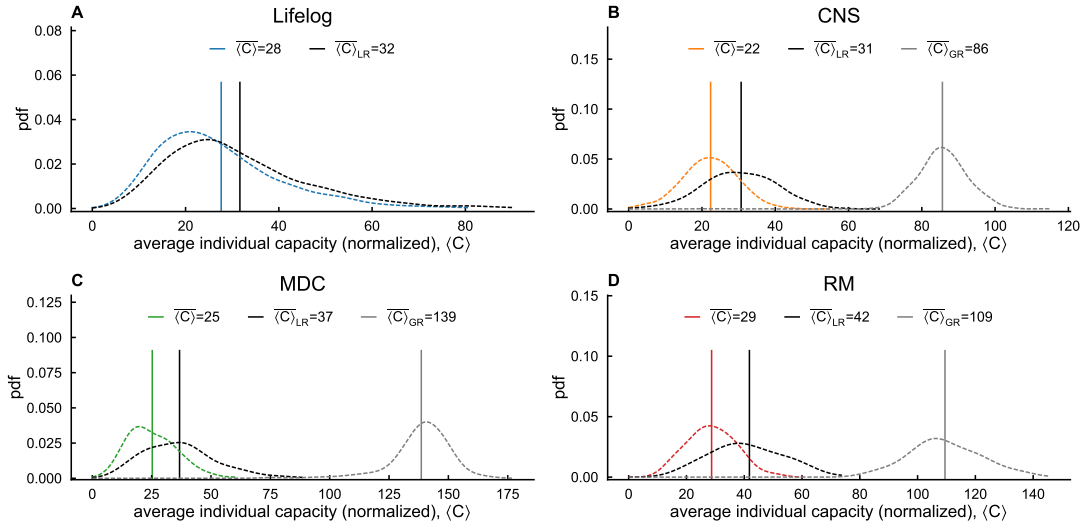
Supplementary Figure 27: Discrepancy with the randomized cases. The Kernel Density of the average individual capacity (normalized to account for the differences in time coverage) for data ( \langle C \rangle ), local ( \langle C \rangle_{LR} ) and global ( \langle C \rangle_{GR} ) randomizations (dashed lines), and the corresponding average values (full lines) computed across the population. The KolmogorovSmirnov test-statistics (Table 5) rejects the hypothesis that the three samples are extracted from the same distribution.
