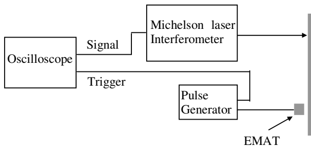
Figure 6.8 Displacement measurement set-up using Michelson laser interferometer
