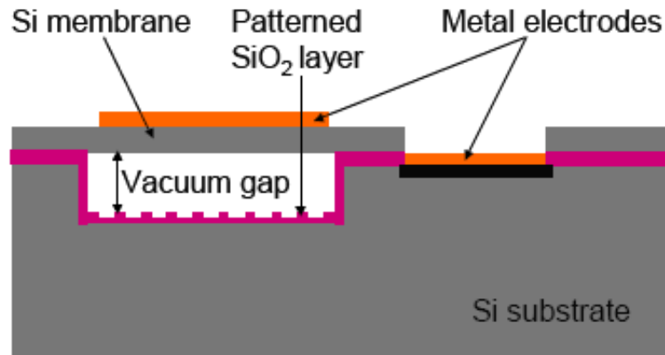
Figure 2.3 Schematic view of a captive Micro-machined ultrasonic transducer.
