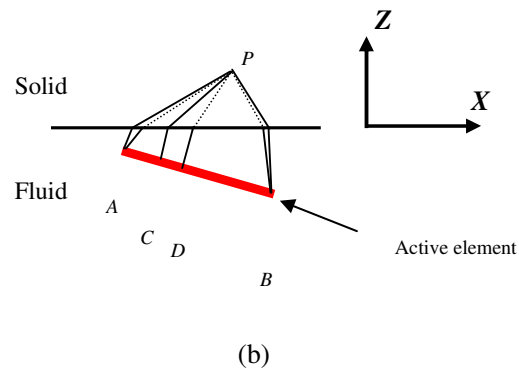
Figure 3.2 Schematic view of measurement setup (a) and ultrasound propagation paths (b) to ultrasonic field point P of plane (plane compression wave from C and plane shear wave from D) and edge waves (edge waves from A and B) generated by a circular piezoelectric transducer water coupled at oblique incidence to a solid.
