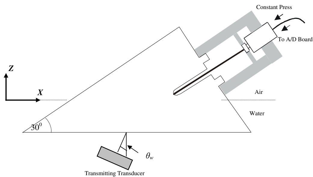
Figure 3.6 Measurement set-up with the miniature probe at 60 degrees to the water/steel interface. \theta_w is the incident angle to the water/steel interface
