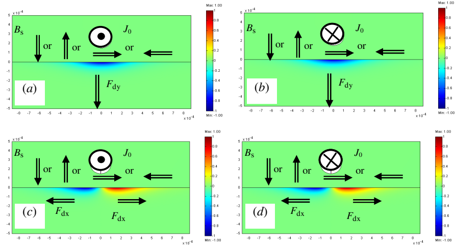
Figure 6.5 Calculated Lorentz forces of the linear coil due to dynamic magnetic field with different directions (Negative Y-, Y-, X- and negative X-direction) of static magnetic field. The direction of the Lorentz force due to dynamic magnetic field is independent of static magnetic field and the direction of the excitation current flowing in the coil. The maximum Lorentz forces in the sample are normalized.
