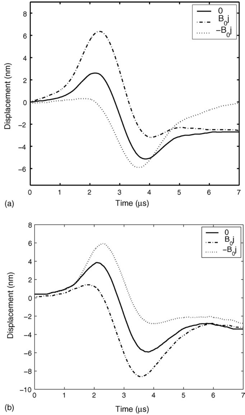
Figure 6.10 Measured Rayleigh wave at a point in X -direction (a) and at a point in negative X -direction (b) respectively, demonstrating the ultrasonic field is not of symmetry over the middle of the linear coil when static magnetic field is along the Y -direction. For clarity, each plot is to an arbitrary time origin
