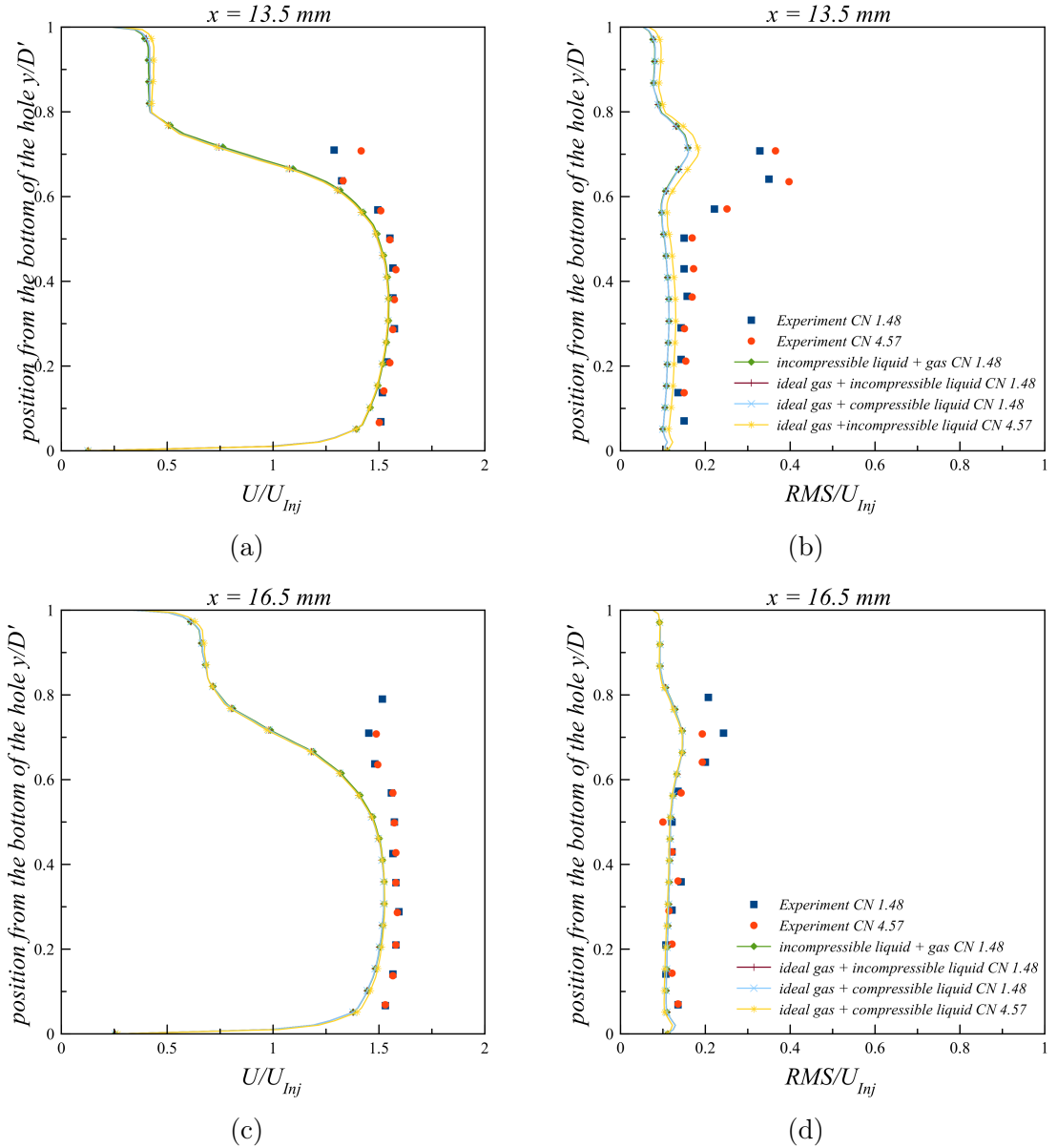
Figure 6.8: Normalized mean axial velocity and RMS comparisons at x = 13.5 \text{ mm} and x = 16.5 \text{ mm} from the origin.
