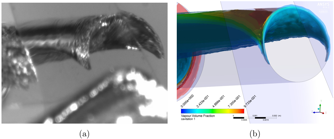
Figure 6.24: (a) Still photograph of the geometry induced cavitation formed at the upper edge of the entrance of the injector hole and travelling downstream, the image indicates cavitation remains stays in the vicinity of the injector wall, the image also indicates horseshoe appearance of cavitation source: Afzal et al. (1999) . (b) isosurface of cavitation prediction at CN = 4.57 , nominal needle lift (6.00 mm), also indicate horseshoe appearance.
