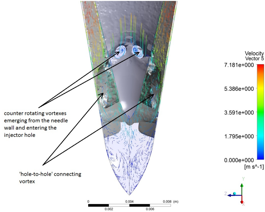
Figure 6.20: A view of the injector from the centre at CN = 4.57 . Isosurface of vorticity magnitude (0.5% of the magnitude) indicates vortices emerging from the needle wall and entering the injector hole, isosurface of vorticity magnitude also indicate the presence of 'hole-to-hole' connecting vortex. Vectors plotted on plane 4 indicate opposite direction of rotation. Vectors also plotted on the periodic boundary which also indicate the presence of 'hole-to-hole' connecting vortex.
