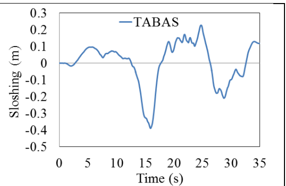
Fig. 12. Time-history of sloshing in tank No.1 (m)
