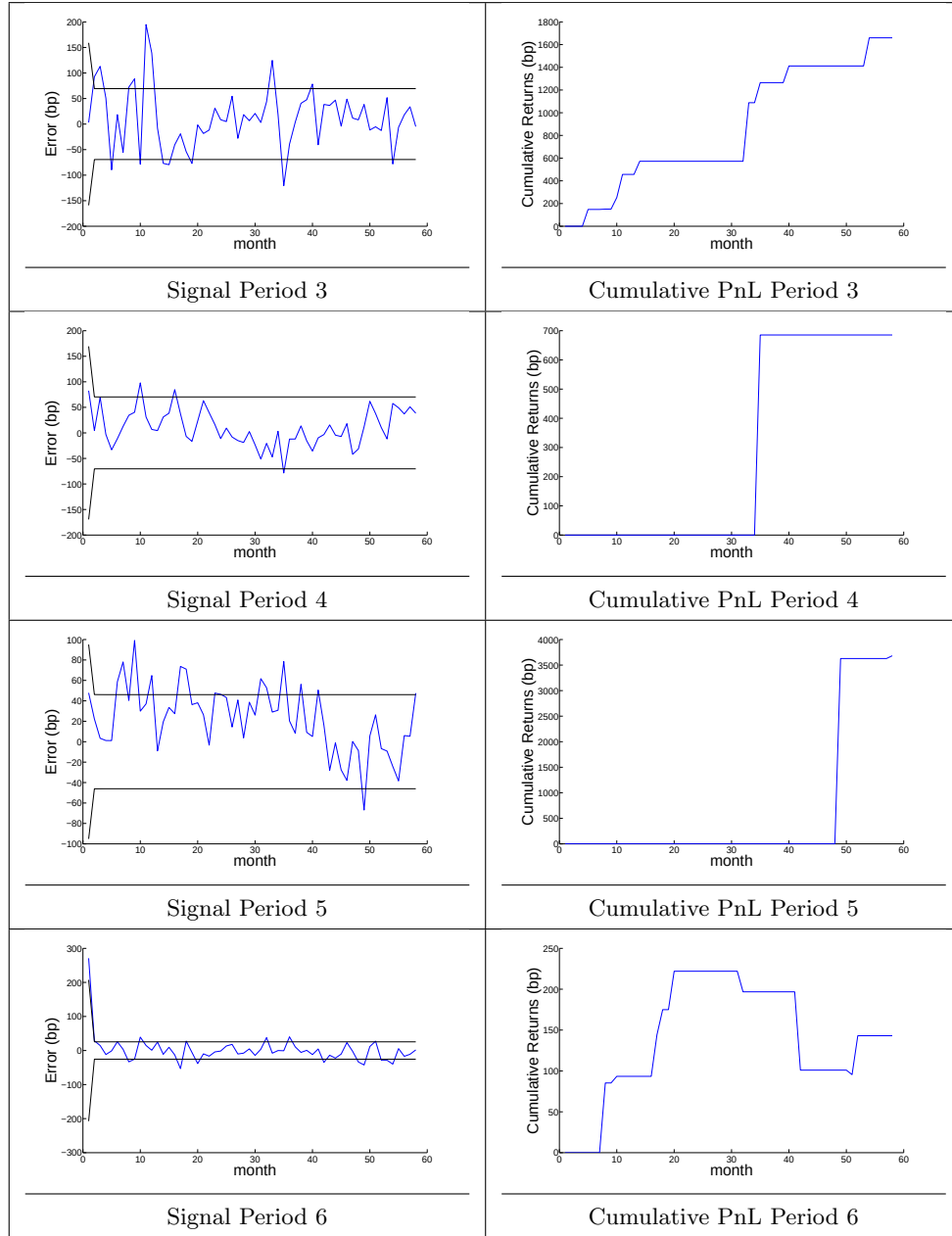
Figure 4.9.5: Steeper Signal and Cumulative PnL from application to Empirical Data
