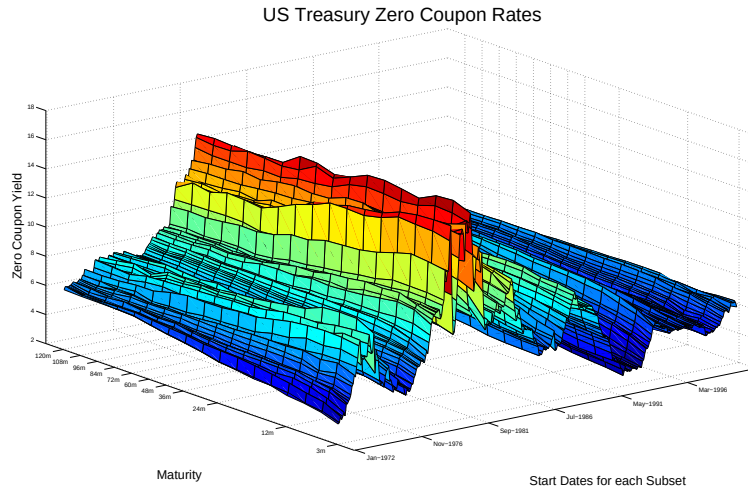
Figure 4.7.1: US Zero Coupon Curve 1972-2000
