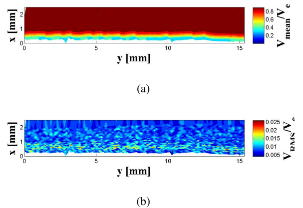
Figure 11: Horizontal string D=0.23mm L1- a)Velocity along the attachment line. b)Root Mean Square (RMS) of the velocity along the attachment line.
