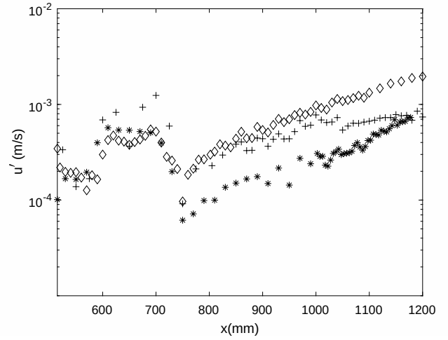
Figure 11: The amplitude of TS wave along the stream-wise direction, for the unexcited case and the excited cases where the TS mode extracted f = 120\text{Hz} , f = 172\text{Hz} and the mode of the first harmonic ( 2f ) of the excitation at f = 86\text{Hz} , represented by ‘ \circ ’, ‘ * ’, ‘ + ’ and ‘ \diamond ’.
