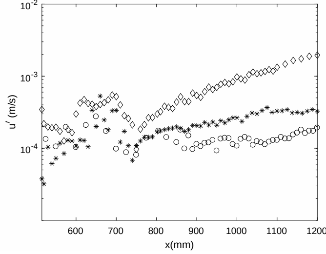
Figure 8: The amplitude of TS wave along the streamwise direction, for the unexcited case and the cases of combination of live motors excited at a frequency of 172\text{Hz} . Where ‘o’ represents the unexcited case and ‘*’ and ‘◊’ represents the case of 1 and 5 motors respectively.
