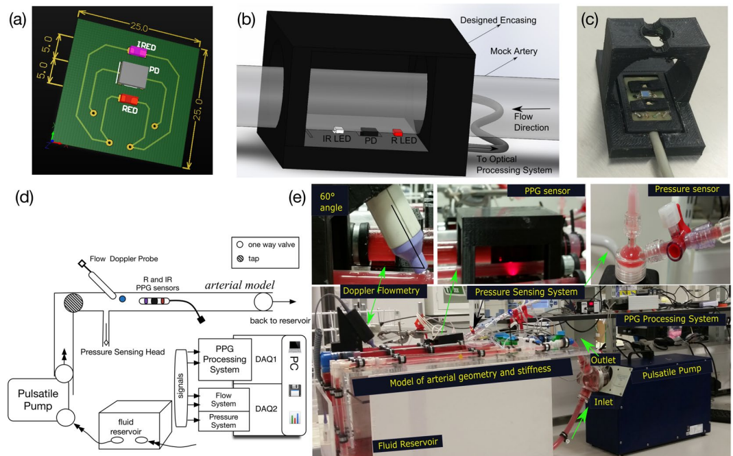
Figure 9. In vitro setup design and implementation. (a) Sensor PCB design, (b) 3D model of sensor and encasing, (c) close-up picture of inner encasing and sensor, (d) schematic of the experimental setup (e) picture of the final experimental design.
