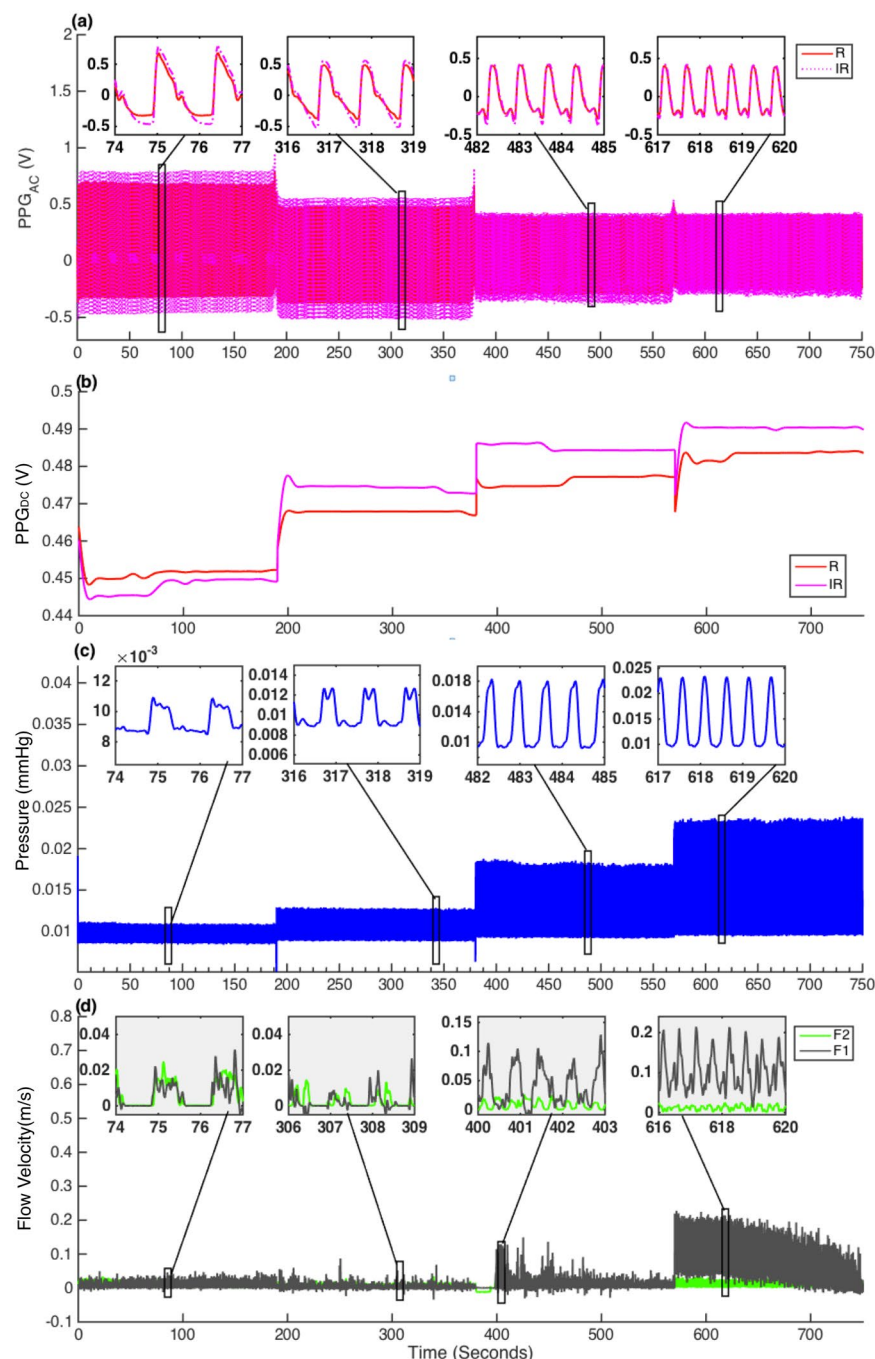
Figure 3. Signals collected during circulating whole equine blood. Data was obtained at 190 seconds for each pumping frequency (0.7, 1, 1.5 and 1.9 Hz). (a) Red (R) and Infrared (IR) PPGAC signals. (b) R and IR PPGDC levels. (c) Pressure (P) signals and (d) shows forward (F1) and backward (F2) flow velocities.
