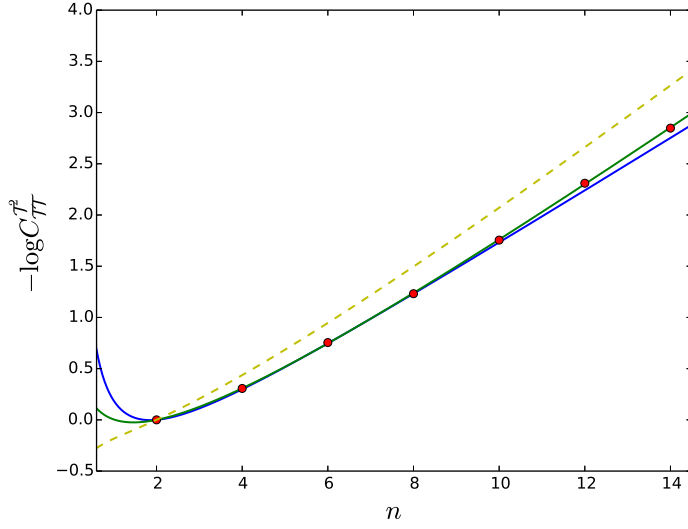
Figure 8.11: Numerical values (red dots) of the logarithm of the three-point structure constant computed using equation (8.68). The blue and green solid line the -1.0 + 0.27n + 0.9/n and -0.31 + 0.31n - 0.46 \log n fitting functions, respectively. These values are checked against \log \tilde{P}_n (yellow dashed line).
