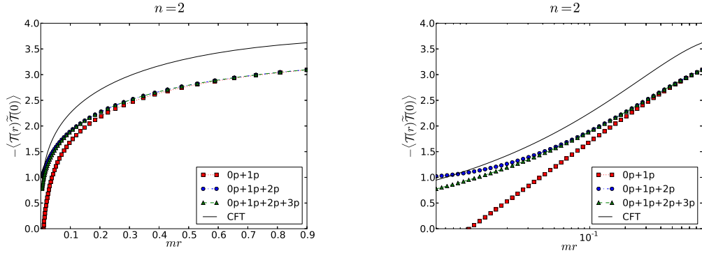
Figure 6.8: Comparison between the perturbative (solid black line) and form factor (coloured points) expansion using linear (left) and logarithmic (right) scales.
