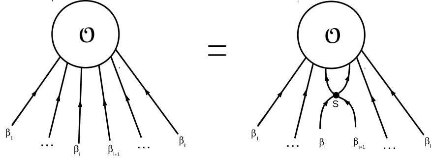
Figure 3.3: Graphical representation of the first Watson equation. In the form factor on the right the two particles i and i + 1 have been exchanged. Since these particles live in a two-dimensional space-time, the scattering is unavoidable.
