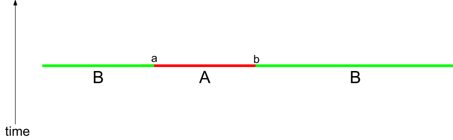
Figure 5.1: Space-time representation of the system.
