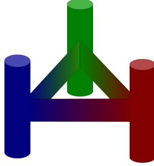
Figure 4.4: Surface \mathcal{M}_3 for n = 3 .
