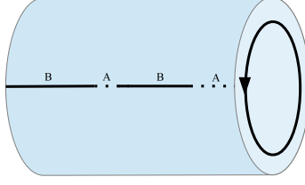
Figure 4.3: Reduced density matrix.
