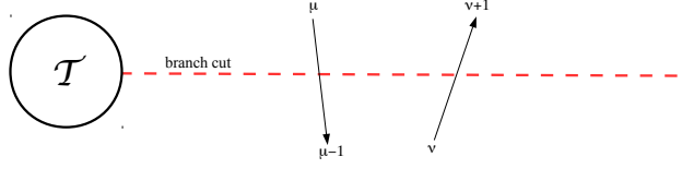
Figure 6.2: The twist field \mathcal{T} creates a branch cut (red dashed line) which moves particles between adjacent copies.
