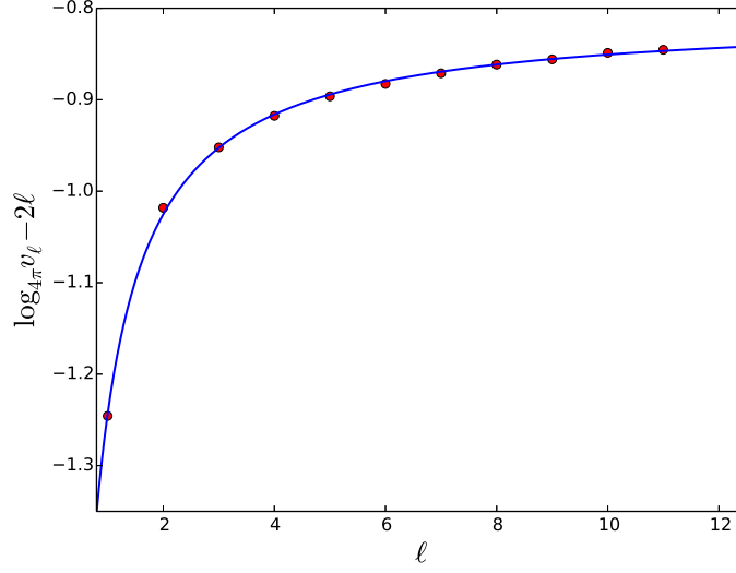
Figure 8.8: The (rescaled) values of v_\ell (red dots) checked against the interpolating function (8.63) (blue line) in linear scale.
