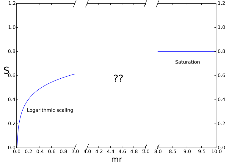
Figure 6.11: Scaling of entanglement entropy at different scales. Near the critical point ( mr \ll 1 ) it scales logarithmically according to the CFT prediction. At the other end of the scale, in the infrared regime ( mr \gg 1 ), the entropy is constant. Less is known about the behaviour of the entropy in the intermediate region. The form factor expansion can be used to estimate how the entropy tends to its saturation value.
