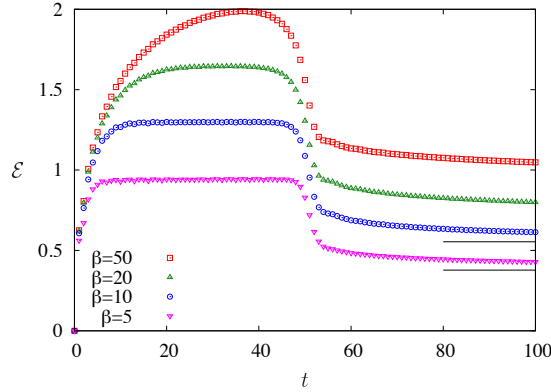
Figure 8.12: Time evolution of logarithmic negativity after a quench at equal temperature \beta^{-1} . Picture taken from [15] with permission from the authors.
