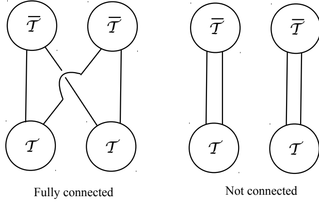
Figure 8.3: Difference between fully connected and not fully connected diagrams. The diagram on the left (right) corresponds to terms like the second (third) line of (8.18). Even though equation (8.18) refers to a \langle \mathcal{T}(0)\tilde{\mathcal{T}}(r) \rangle correlator, four operators appear in this picture instead of just two. This discrepancy is corrected by the fact that the form factors we are taking into account are normalised by the VEV of \mathcal{T} .
