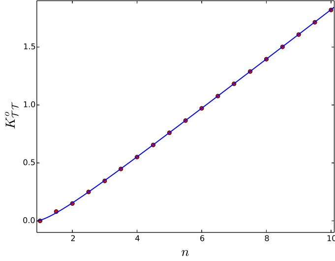
Figure 8.9: Numerical values of \kappa_{\mathcal{T}\mathcal{T}}^o (red dots) for different integer and non integer values of n . The blue line represent the best fit -0.34 + 0.215n + 0.13/n .
