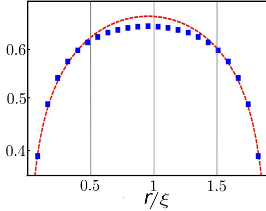
Figure 5.4: Scaling of entanglement entropy in the Lee-Yang chain with N = 24 sites against the length r of the subsystem A (normalised by the correlation length \xi - see text). The blue squares represent the numerical data, while the red dashed line corresponds to the fit (5.26).
