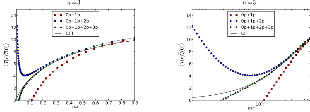
Figure 6.9: Comparison between the perturbative (solid black line) and form factor (coloured points) expansion using linear (left) and logarithmic (right) scales.
