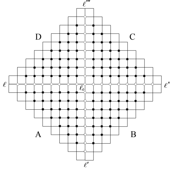
Figure 7.4: Diamond shaped lattice divided into four corners. Each Corner Transfer Matrix depends on the values of the local height on the two edges (denoted by \circ ). The internal sites ( \bullet ) should be considered already summed over all possible configurations.
