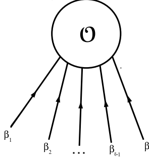
Figure 3.2: Form factors of the operator \mathcal{O} with \ell incoming particles
