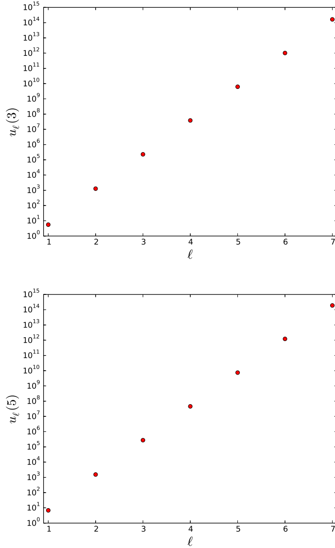
Figure 8.5: Values of u_\ell(3) and u_\ell(5) in linear-logarithmic scale.
