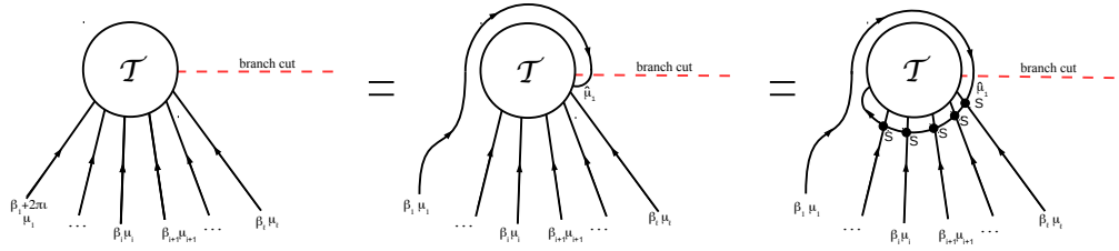
Figure 6.1: Second Watson equation for twist field. The branch cut (red dashed line) modifies particles when they cross it.
