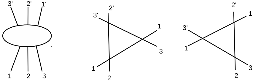
Figure 3.1: The three-particle scattering (first diagram) can be factorised into three two-particle processes (second and third diagrams). The only difference between the two factorisations is the order of the individual scattering processes.
