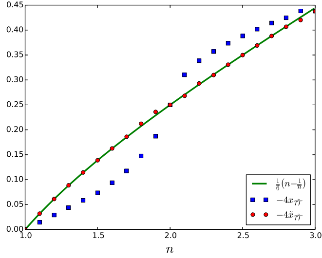
Figure 8.4: Numerical evaluation of the scaling dimension -4x_{\mathcal{T}\tilde{\mathcal{T}}} for integer and non integer values of n . In order to compute the sum (8.44) for a very high value of \ell , the actual values have been computed through a numerical fit. We computed and summed the first 150 terms of (8.44), then we completed the sum by fitting the logarithm of each term from \ell=20 to \ell=150 against \log \ell .
