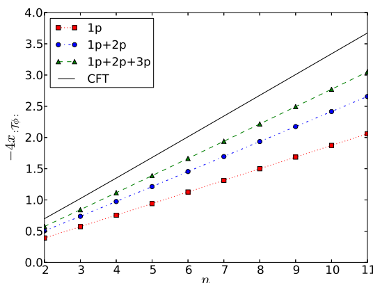
Figure 6.6: Scaling of the correlator \langle : \mathcal{T}\phi : (r) : \tilde{\mathcal{T}}\phi : (0) \rangle . The CFT prediction is given by the black solid line, while the one-, two- and three- particle form factor expansion are given respectively by the red squares, blue circles and green triangles.
