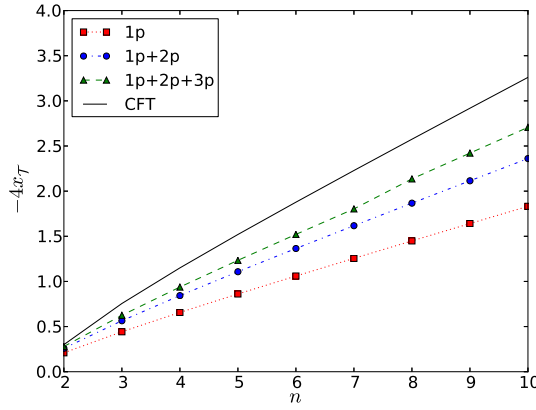
Figure 6.5: Scaling of the correlator \langle \mathcal{T}(0)\tilde{\mathcal{T}}(r) \rangle . The CFT prediction is given by the black solid line, while the one-, two- and three- particle form factor expansion are given respectively by the red squares, blue circles and green triangles.
