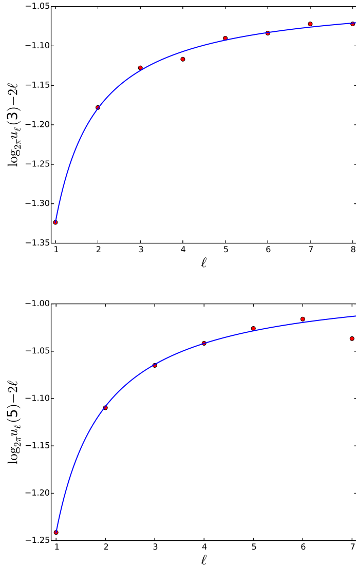
Figure 8.6: Values (rescaled) of u_\ell(3) and u_\ell(5) (red dots) in linear scale checked against the fit (8.59) (blue line).
