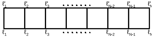
Figure 7.2: A row-to-row transfer matrix between two spin configurations.
