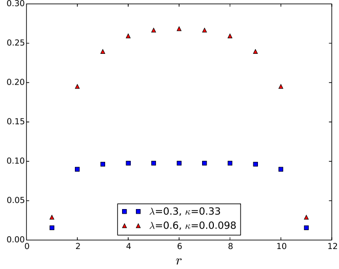
Figure 5.5: Scaling of entanglement entropy in the Lee-Yang chain with N = 12 sites against the length r of the subsystem. In this case the finite size gap is too large to extract meaningful critical information.
