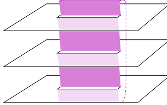
Figure 4.5: Surface \mathcal{M}_3 for n = 3 and \beta = \infty . Picture taken from [14] with permission from authors.
