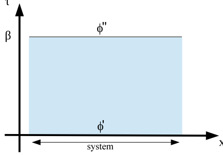
Figure 4.1: Propagator using path integrals.
