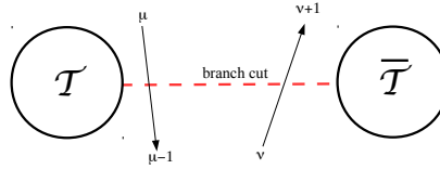
Figure 6.4: When both twist fields are present, a finite branch cut (red dashed line) is created.
