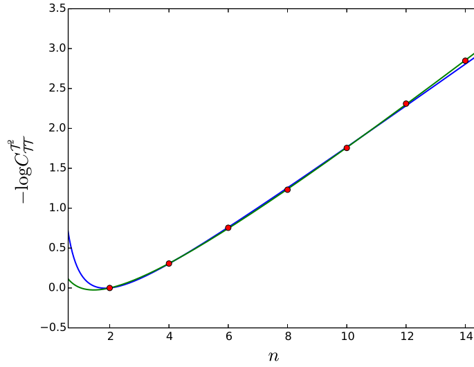
Figure 8.10: Numerical values of -\log C_{TT}^{T^2} for some even values of n (red dots). Both interpolating functions (blue and green lines) provide a very good fit of the data.
