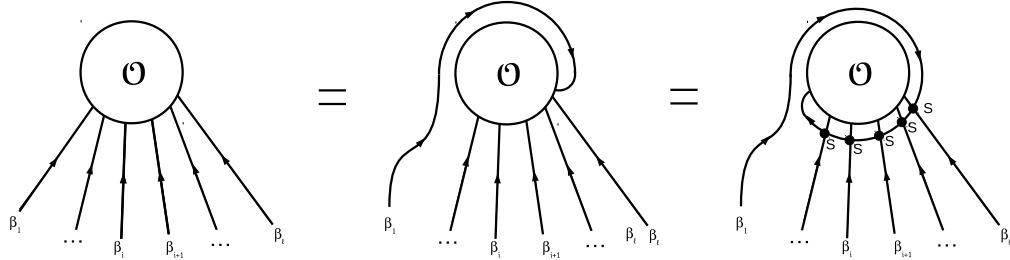
Figure 3.4: Graphical representation of the second Watson equation. A shift by 2\pi i in the first rapidity implies a complete rotation of the particle around the operator \mathcal{O} . The initial order of particles can be restored by making the first particle scatter with all others.
