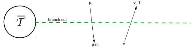
Figure 6.3: The twist field \tilde{\mathcal{T}} creates a branch cut (green dashed line) which moves particles between adjacent copies. Notice that the orientation of this branch cut is reversed compared to \mathcal{T} (Figure 6.2).
