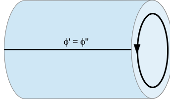
Figure 4.2: Partition function
