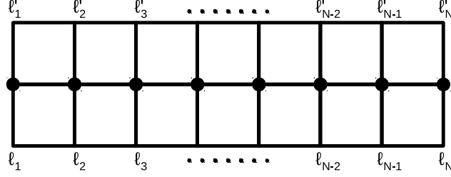
Figure 7.3: A double-row-to-row transfer matrix between two spin configurations. The intermediate spins (black dots) are summed over all possible configurations.
