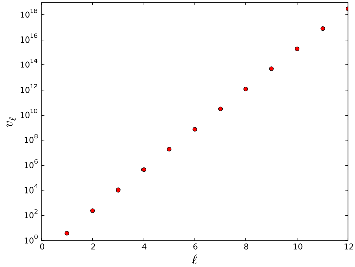
Figure 8.7: The values of the integrals v_\ell in linear-logarithmic scale.
