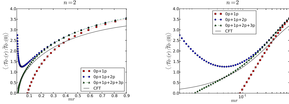
Figure 6.7: Comparison between the perturbative (solid black line) and form factor (coloured points) expansion using linear (left) and logarithmic (right) scales.
