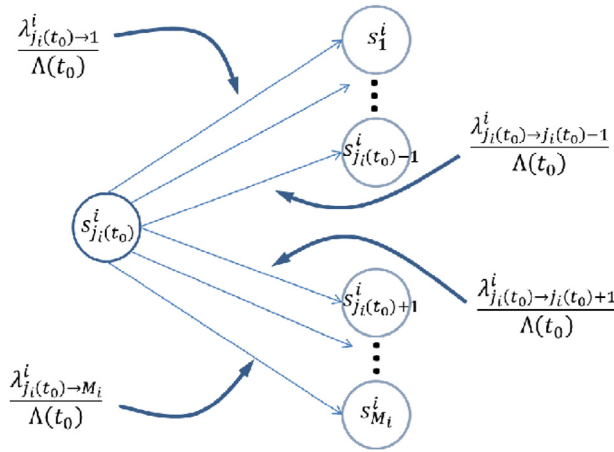
Fig. 3. Using a competing risks algorithm, an ME transits, with probability, from a state s_{ji}^i(t_0) at time t_0 to some other state at some future point in time. In this example, each transition's associated probability of occurrence is a quotient (such as \frac{\lambda_{ji}^i(t_0) \rightarrow 1}{\Lambda(t_0)} ) of transition rates for exponential distributions.
