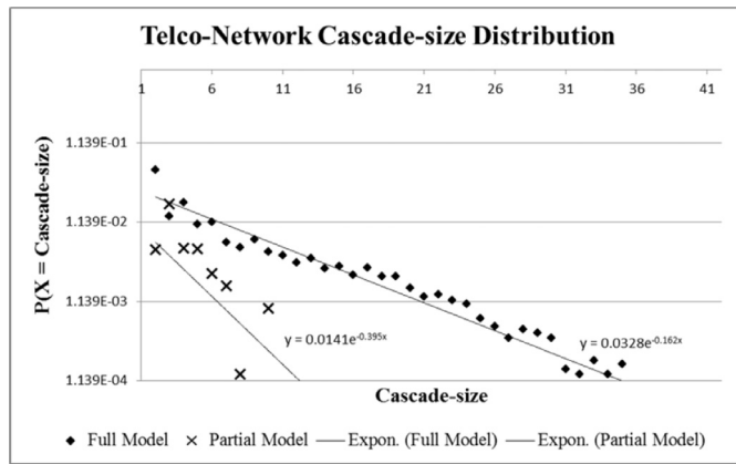
Fig. 9. A comparison of the distribution of cascade-sizes in the Telecommunications Network under two levels of abstraction: 1) when the telecommunications network is coupled with a detailed model of the power network (full model), and 2) when only a simple model of the power network is used with everything else remaining the same (partial model). The value of the scaling factor for both models is \alpha = 1 .
