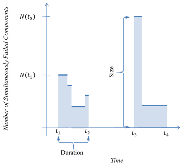
Fig. 6. This illustrates the evolution of two cascades. Each cascade has a duration and size that are random variables; only by observing a cascade to its conclusion can one know what its size and duration is. Each of these random variables can be used to define risk-measures related to cascades: that is, they define probability distributions (e.g. of cascade-size or cascade-duration) associated with the cost of a cascade's occurrence.
