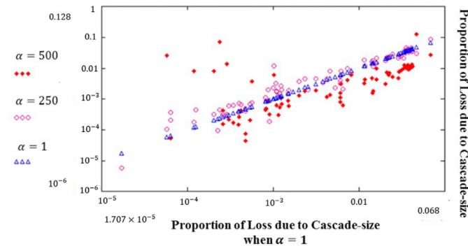
Fig. 14. The proportion of loss due to a cascade of a given size can differ with different values of \alpha .
