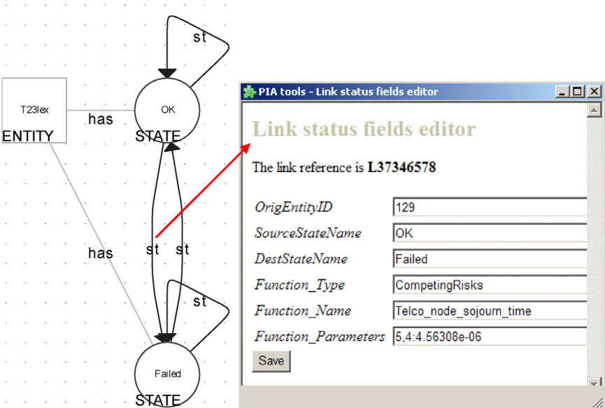
Fig. 18. A state machine diagram for an ME (a local telephone exchange) with an illustration of the parameters attached to a state transition.
