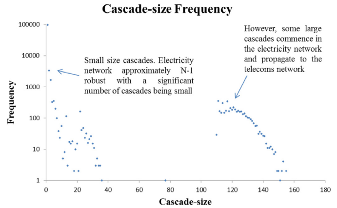
Fig. 7. This risk-measure is the distribution of cascade-sizes across the combined network consisting of both the Power Critical Infrastructure and the Telecommunications Critical Infrastructure. The value of the stochastic dependence scaling factor is \alpha = 1 .
