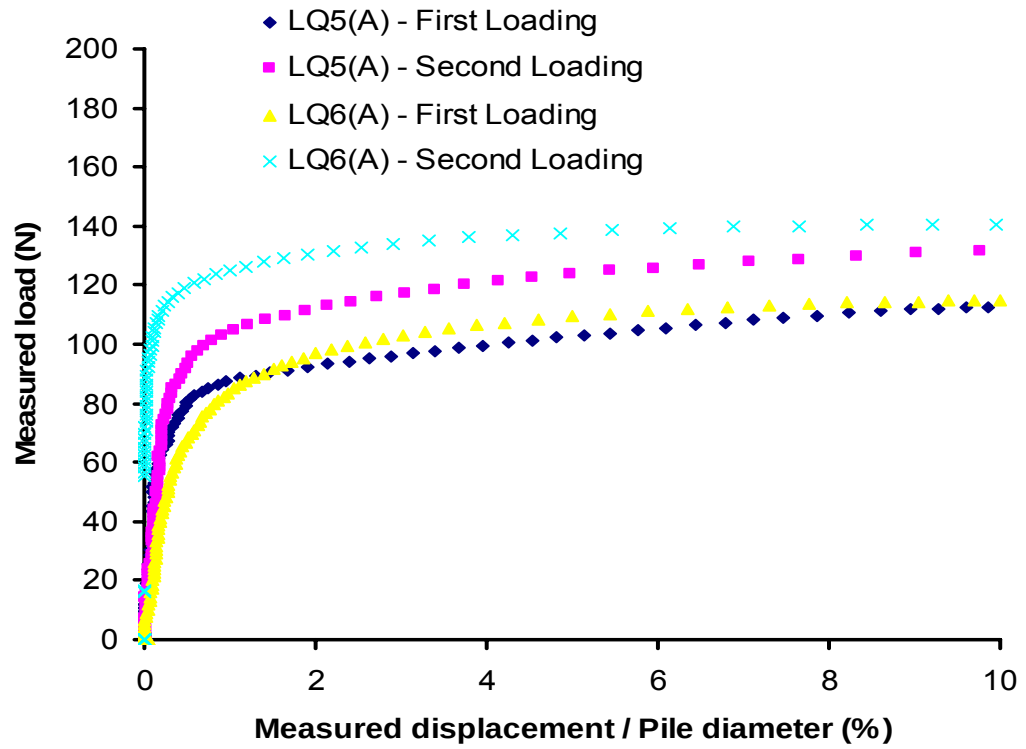
Figure 4.11 Test LQ5(A) and LQ(6) single pile foundations subjected to 1 st and 2 nd loading to failure. An increase in pile capacity of 20% was observed during 2 nd loading.
