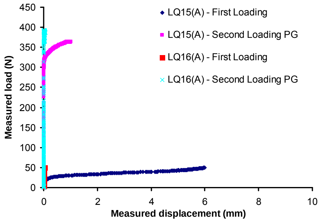
Figure 4.28 Tests LQ15(A) and LQ16(A). 1 st loading cycle – single pile foundations loaded up to working load. 2 nd loading cycle – novel pile group: Test LQ15(A) eight 200mm long mini-piles with 3D spacing; Test LQ16(A) eight 200mm long mini-piles with 2D spacing.
