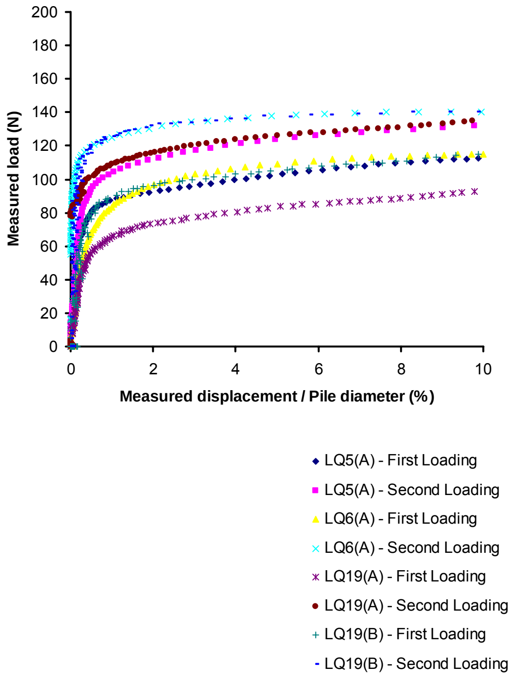
Figure 4.32 Performance of single pile foundations during 1 st and 2 nd loading. Tests LQ5(A) and LQ6(A) – centrifuge was stopped between the first and second loading. Tests LQ19(A) and LQ19(B) – centrifuge was NOT stopped between the first and second loading.
