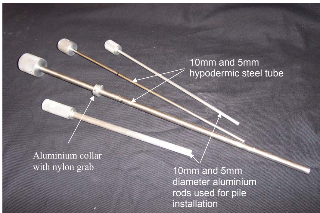
Figure 3.46 Stainless steel tubes used for model pile installation.
