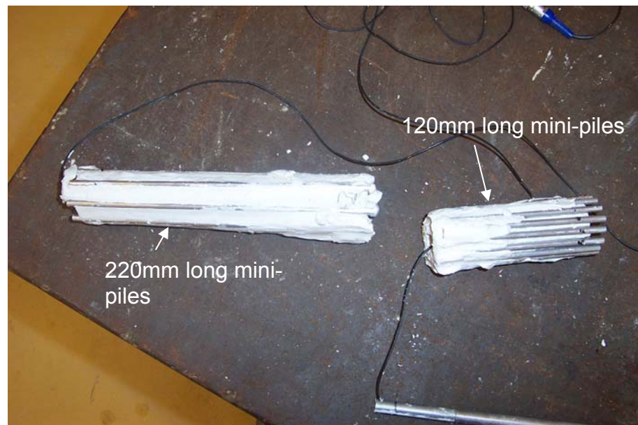
Figure 3.53 Mini-pile groups removed from the model soil after testing (Test LQ16).
