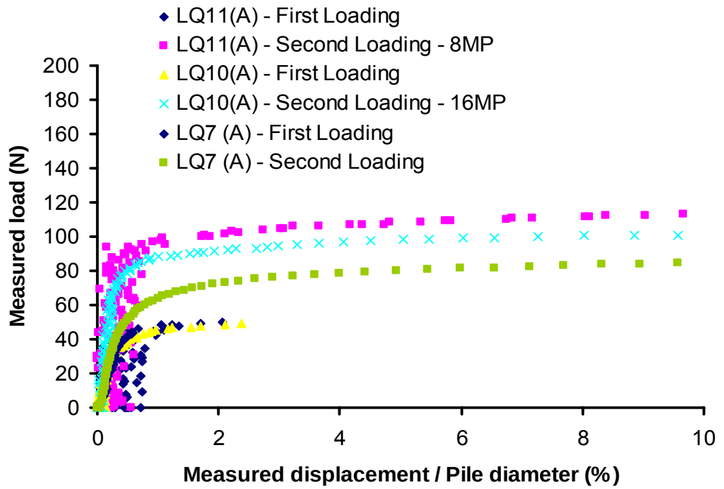
Figure 5.24 Tests LQ7(A), LQ10(A) and LQ11(A). 1 st loading cycle – single pile foundations loaded up to working load. 2 nd loading cycle – enhanced piled foundations loaded to failure: test LQ7(A) – single pile, test LQ10(A) enhanced pile foundation with sixteen 100mm long mini-piles at 3D spacing and test LQ11 enhanced pile foundation with eight 100mm long mini-piles at 3D spacing.
