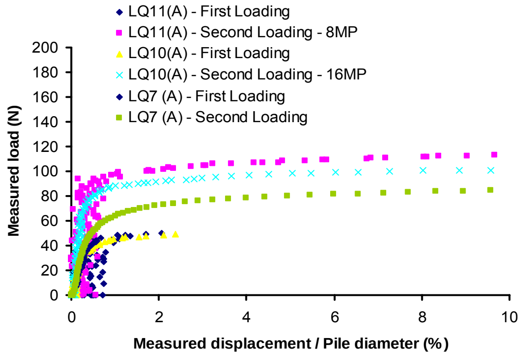
Figure 4.21 Tests LQ7(A), LQ10(A) and LQ11(A). 1 st loading cycle – single pile foundations loaded up to working load. 2 nd loading cycle – enhanced piled foundations loaded to failure: test LQ7(A) – single pile, test LQ10(A) enhanced pile foundation with sixteen 100mm long mini-piles at 3D spacing and test LQ11 enhanced pile foundation with eight 100mm long mini-piles at 3D spacing.
