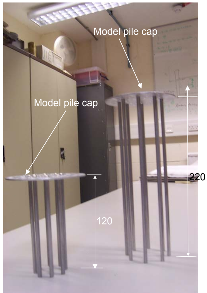
Figure 3.51 120mm and 220mm model mini-pile foundations.
