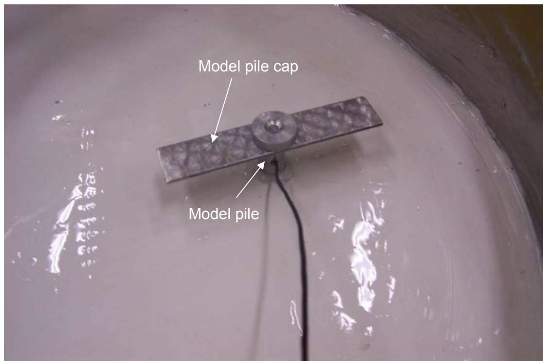
Figure 3.57 Model plate connected to the pile head 20mm above the clay surface.
