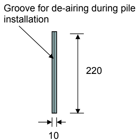
Figure 3.50 10mm diameter model pile with a groove for de-airing during installation.
