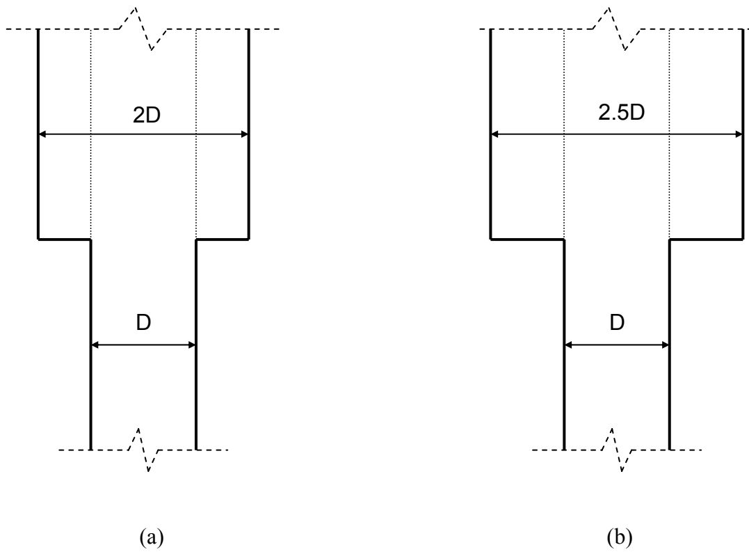
Figure 5.25 Effective geometry of the enhanced centre pile with 100mm long mini-piles installed at 2D centre to centre spacing with the existing centre pile: (a) Mini-pile group of 8 (Test LQ11(A)) (b) Mini-pile group of 16 (Test LQ10(A)).
