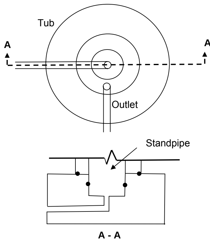
Figure 3.63 Detail of standpipe developed for centrifuge model testing.
