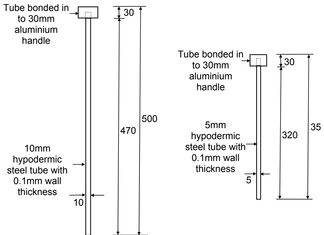
Figure 3.45 Details of tool used for installing bored model piles.
