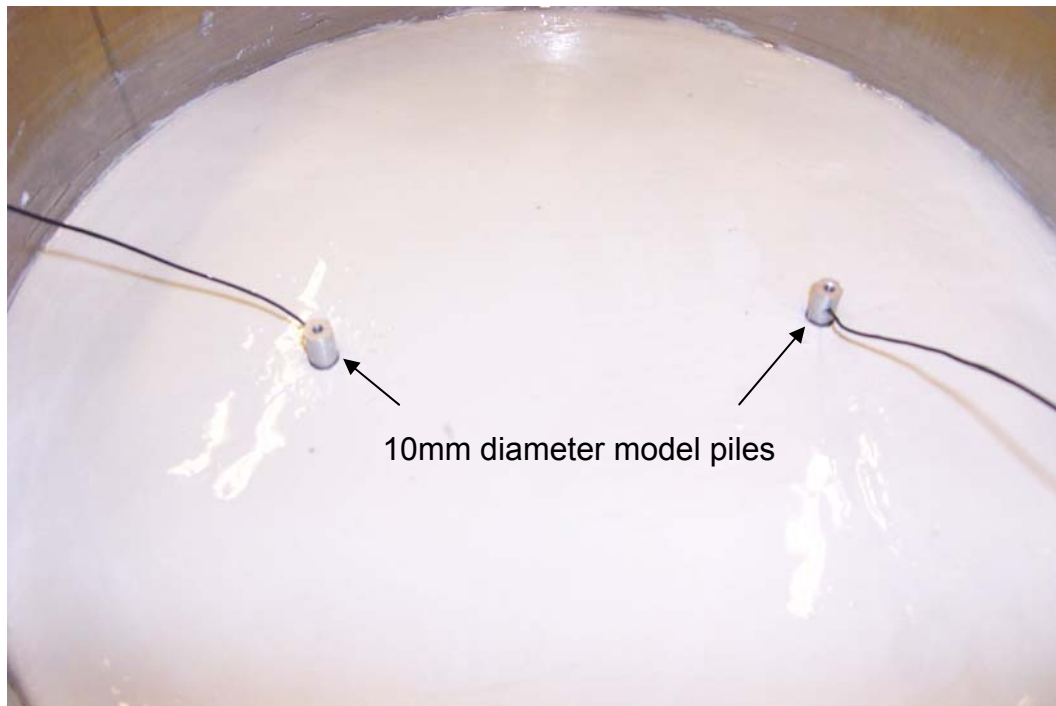
Figure 4.6 10mm diameter piles installed at 1g and embedded 200mm into the soil sample.
