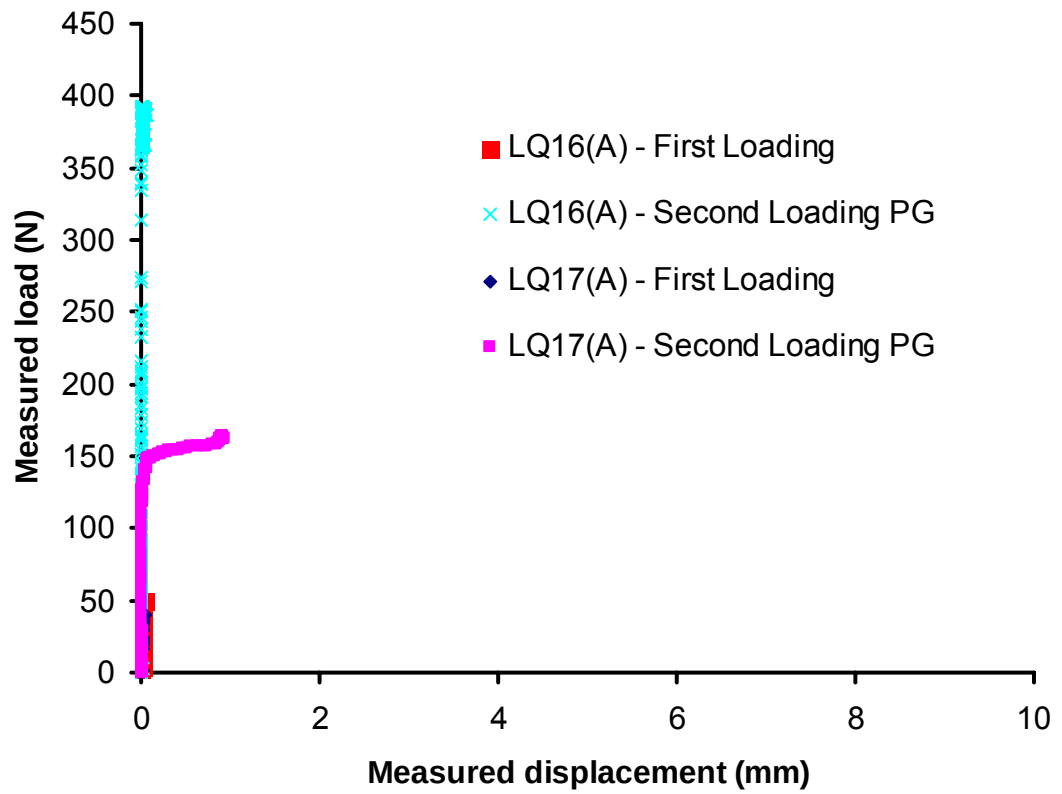
Figure 4.29 Tests LQ16(A) and LQ17(A). 1 st loading cycle – single pile foundations. 2 nd loading cycle – novel pile group: Test LQ16(A) eight 200mm long mini-piles with 2D spacing; Test LQ17(A) four 200mm long mini-piles with 2D spacing.
