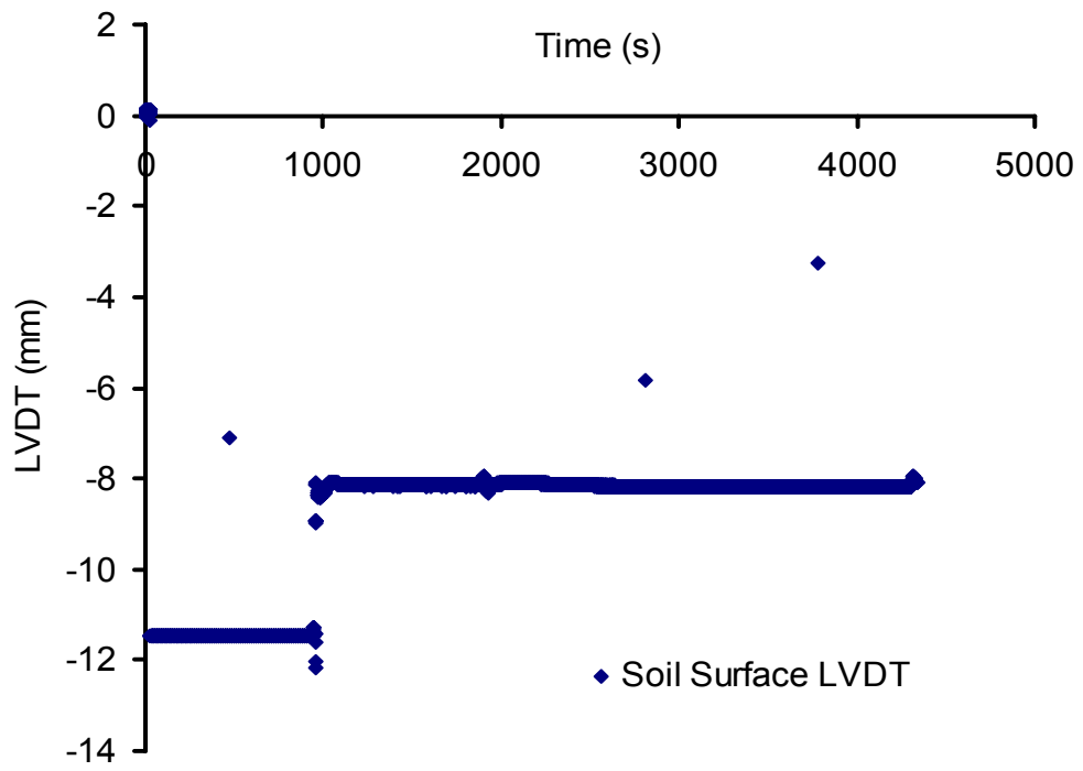
Figure 5.2 Typical soil surface compression and swelling measurements with time during centrifuge model testing (Test LQ6).
