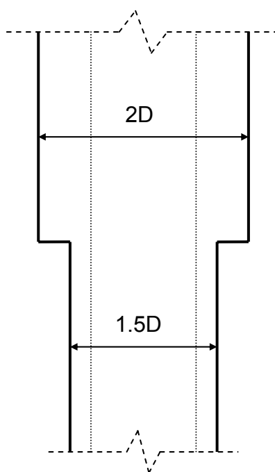
Figure 5.20 Effective geometry of the enhanced centre pile with 200mm long mini-piles installed at 1.5D centre to centre spacing with the existing centre pile.
