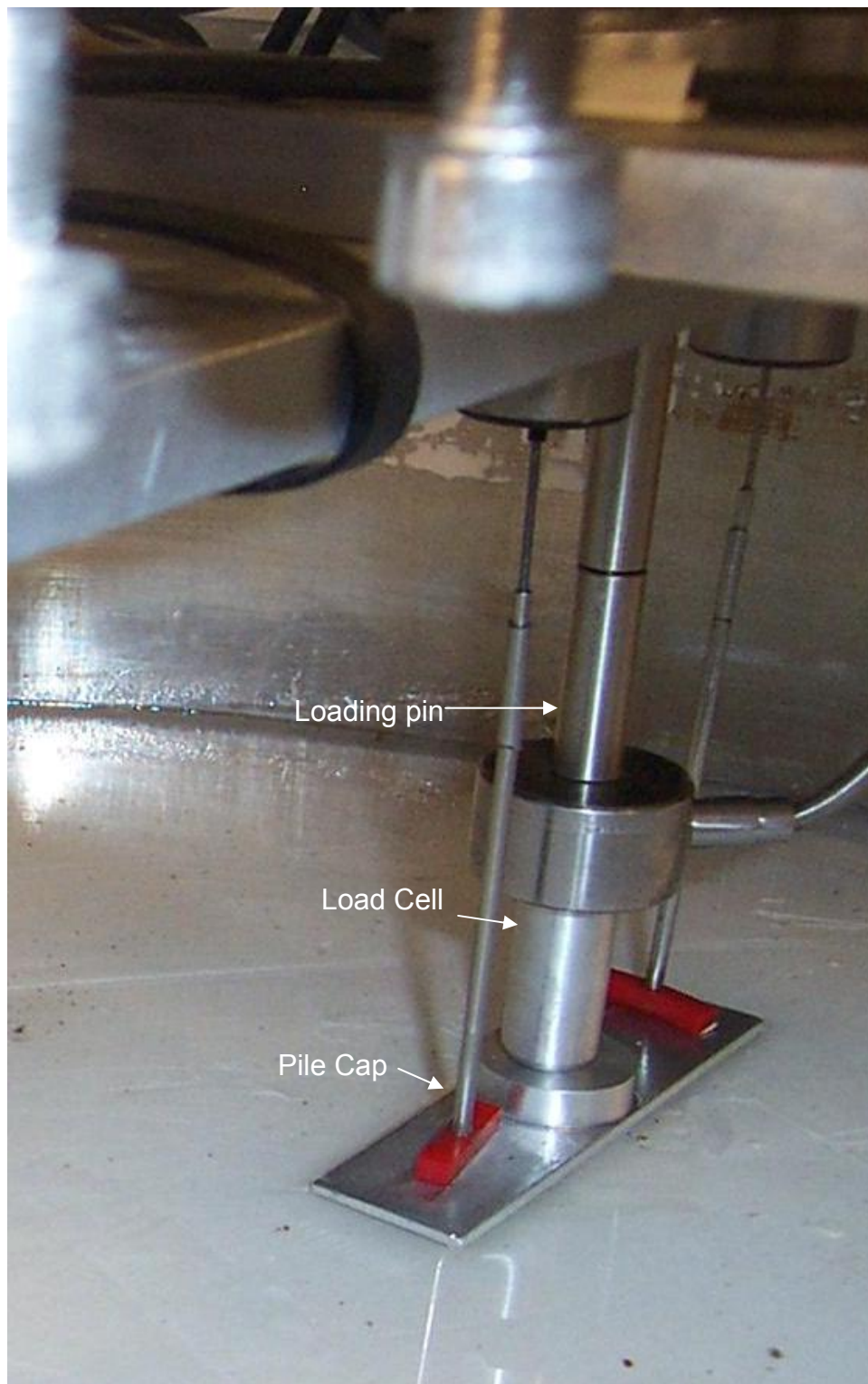
Figure 5.9 Loading pin used to axially load piles during centrifuge model testing and load cell used to measure the load applied.
