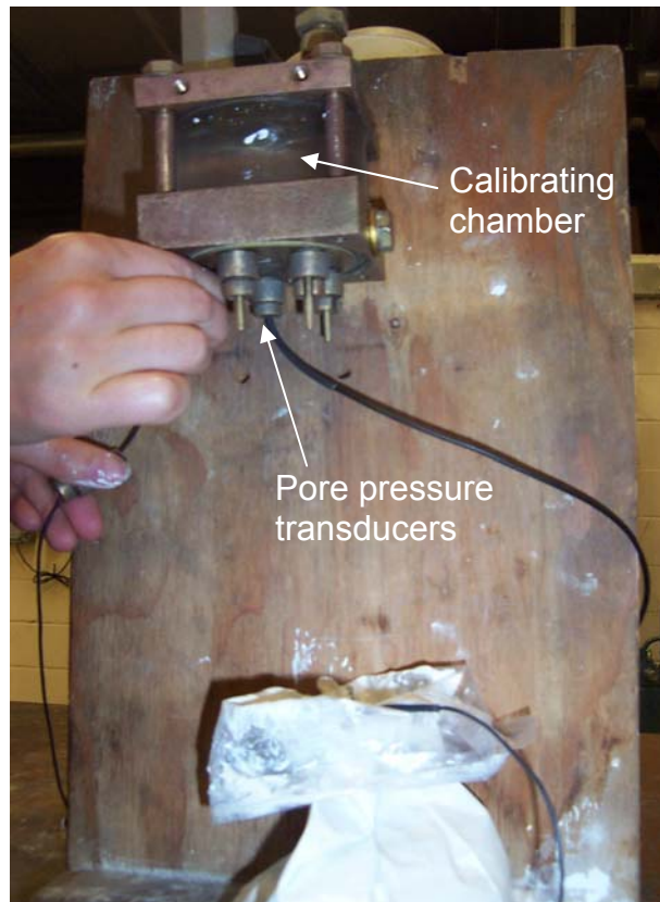
Figure 3.64 Pore pressure transducers in calibration chamber used for centrifuge model testing.
