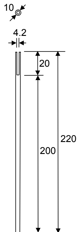
Figure 3.42 Aluminium model pile used for centrifuge model testing.
