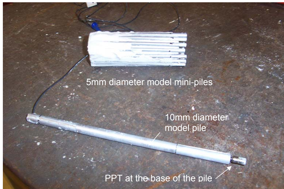
Figure 3.43 Model pile made of aluminium sections with the pore pressure transducer at the base (Test LQ10).
