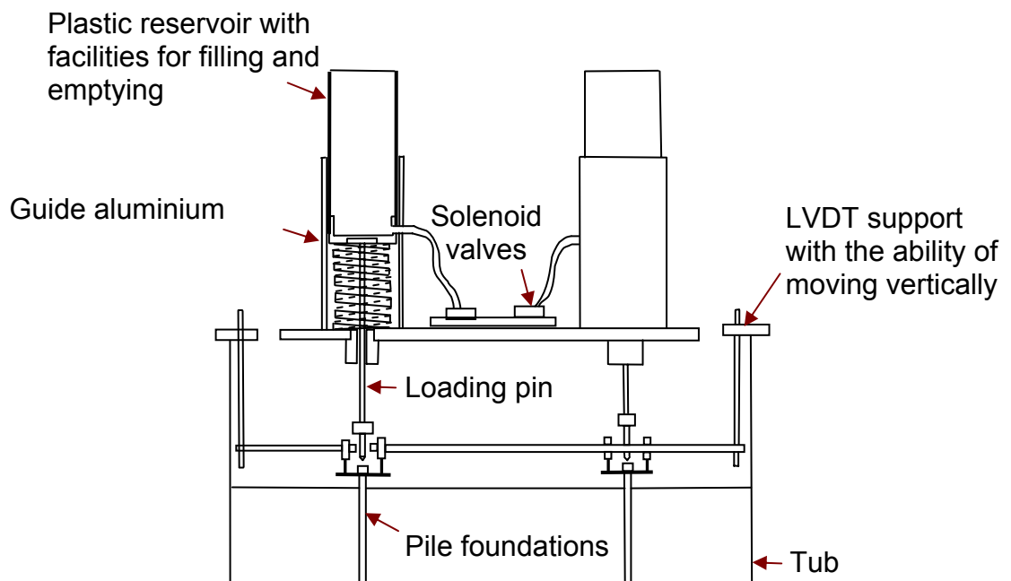
Figure 6.2 New loading apparatus developed for centrifuge model testing.
