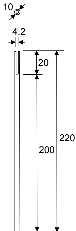
Figure 5.6 Aluminium model pile used for centrifuge model testing.
