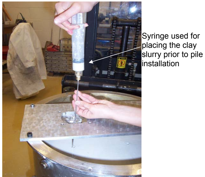
Figure 3.49 Prior to model pile installation a small amount of clay slurry is placed into the bored hole to ensure that the model pile is in good contact with clay model.
