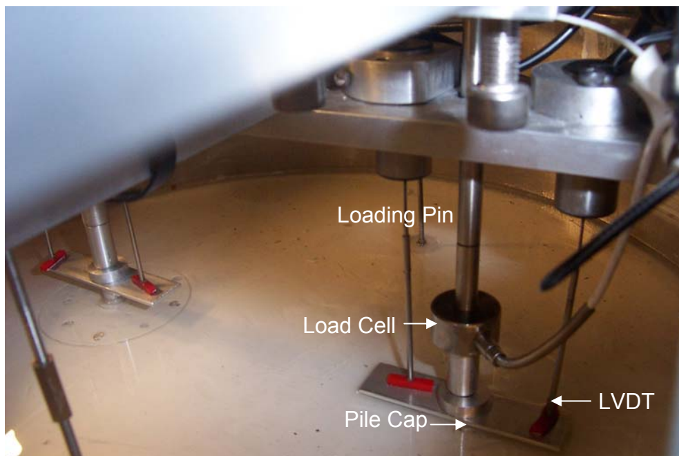
Figure 6.8 Load cell connected to a loading pin used in centrifuge model testing.
