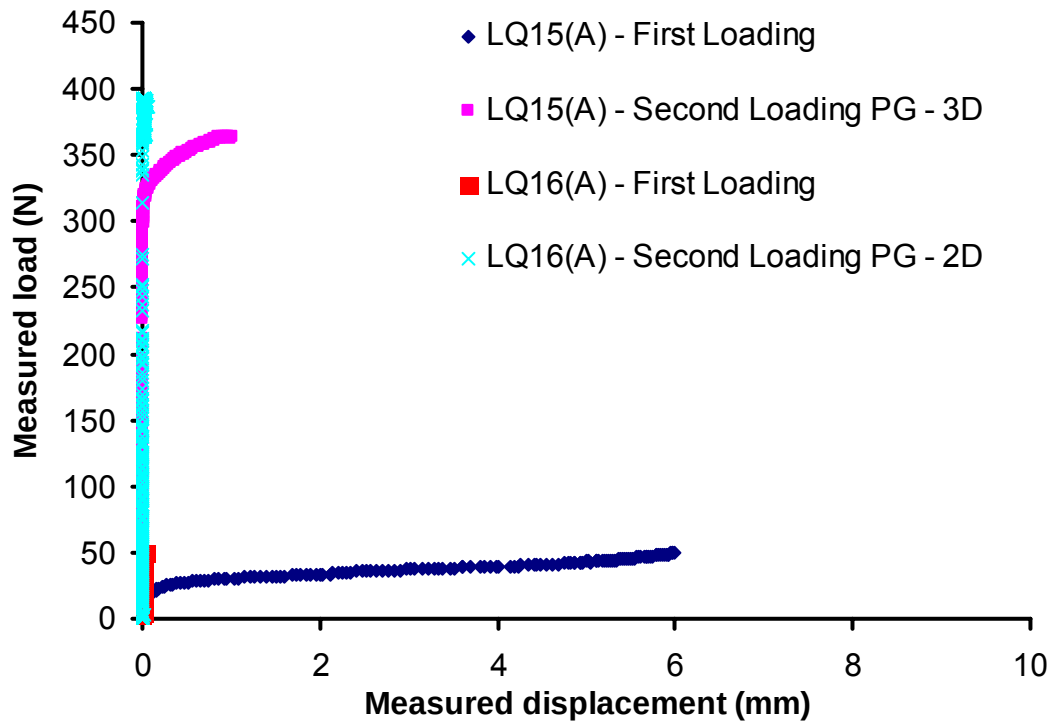
Figure 5.30 Tests LQ15(A) and LQ16(A). 1 st loading cycle – single pile foundations loaded up to working load. 2 nd loading cycle – novel pile group: Test LQ15(A) eight 200mm long mini-piles with 3D spacing; Test LQ16(A) eight 200mm long mini-piles with 2D spacing.
