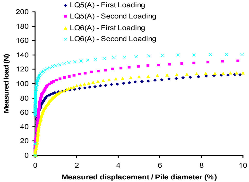
Figure 5.10 Test LQ5(A) and LQ(6) single pile foundations subjected to 1 st and 2 nd loading to failure. An increase in pile capacity of 20% was observed during 2 nd loading.
