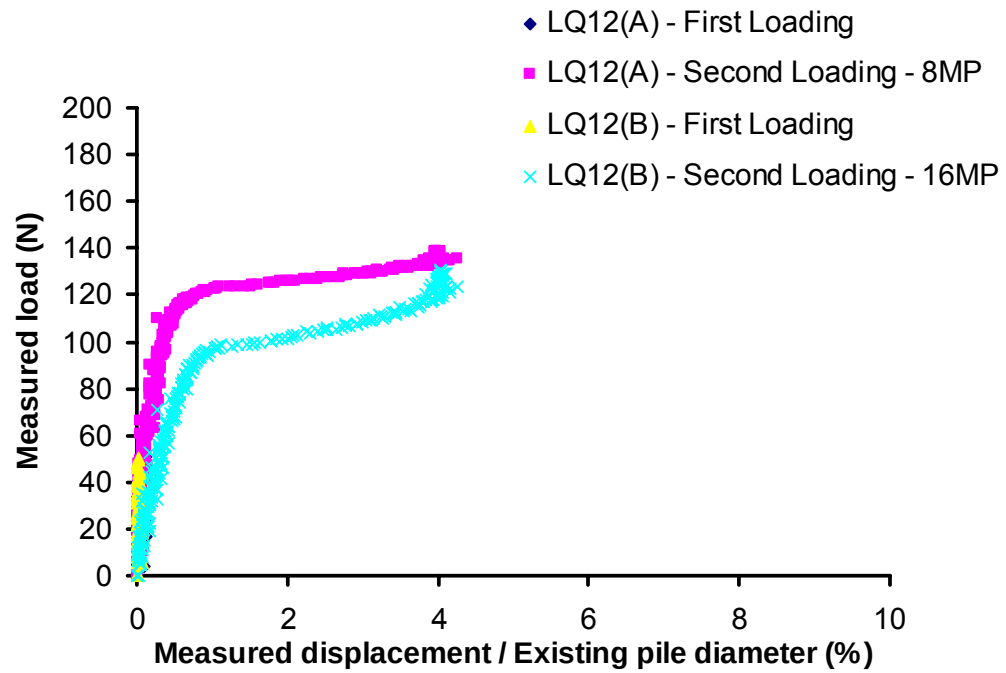
Figure 6.14 Tests LQ12(A) and LQ12(B). 1 st loading cycle – single pile foundation loaded up to working load. 2 nd loading cycle – enhanced pile foundation: Test LQ12(A) eight 200mm long mini-piles with 2D spacing; Test LQ12(B) sixteen 200mm long mini-piles with 2D spacing.
