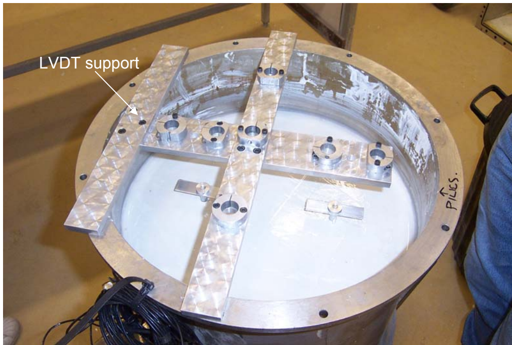
Figure 3.24 Linearly Variable Differential Transformers (LVDT) support used for the first centrifuge model testing.
