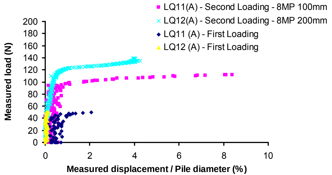
Figure 6.15 Tests LQ11(A) and LQ12(A). 1 st loading cycle – single pile foundation loaded up to working load. 2 nd loading cycle – enhanced pile foundation: Test LQ11(A) eight 100mm long mini-piles with 2D spacing; Test LQ12(A) eight 200mm long mini-piles with 2D spacing.
