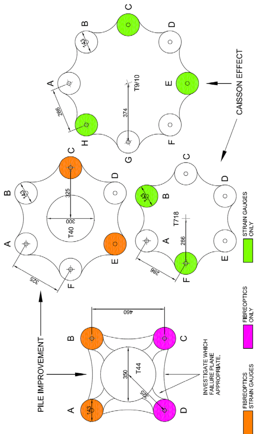
Figure 5.35 Pile improvement and caisson effect using mini-piles, trials at Chattenden, Kent, UK (Ferne et al., 2006).
