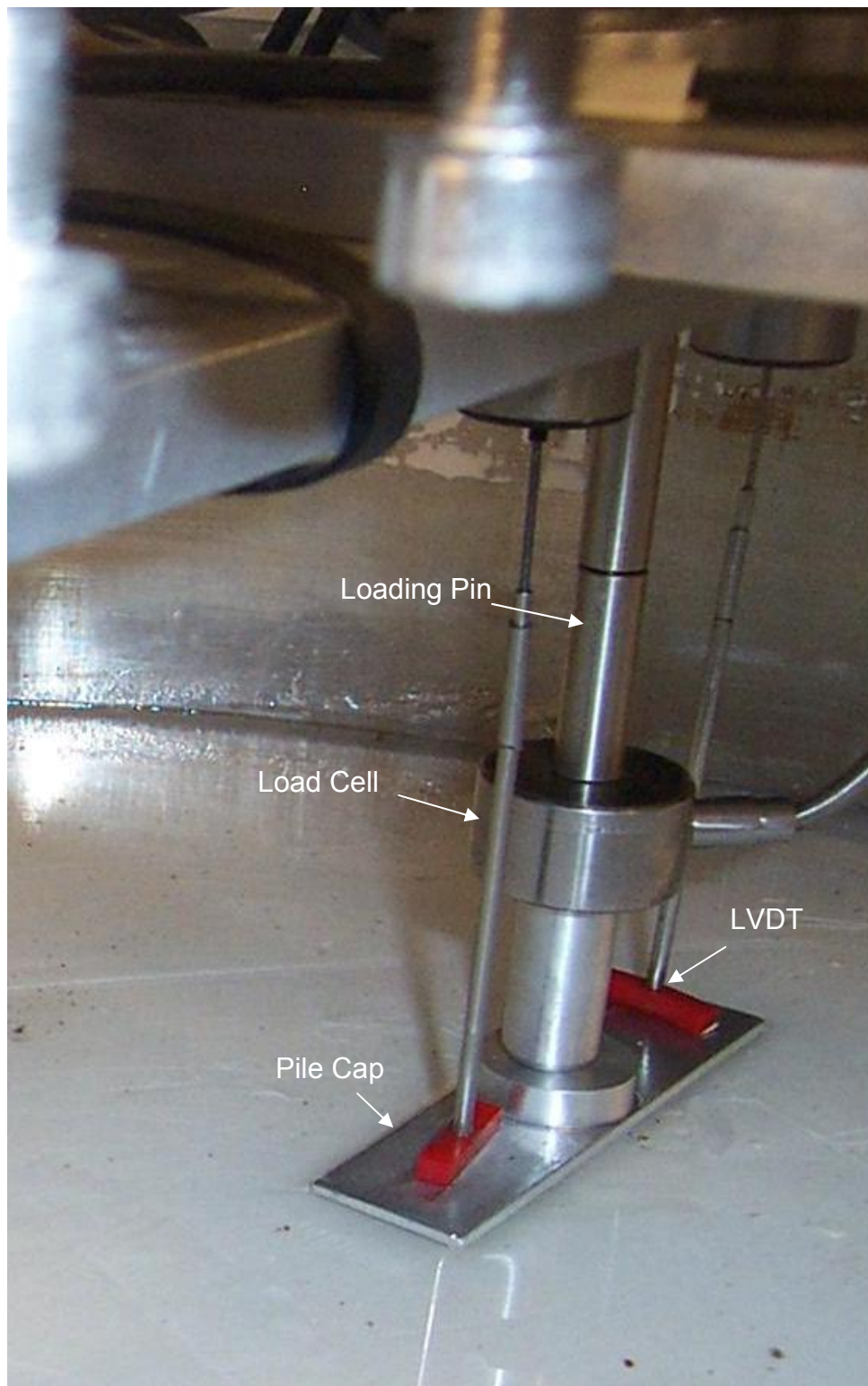
Figure 3.21 Loading pin used to axially load piles during centrifuge model testing.
