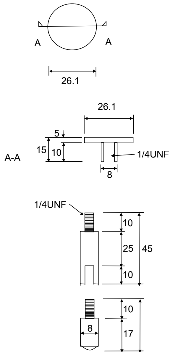
Figure 3.28 Loading pin and the loading pin base used for connecting to the base of the water reservoir.
