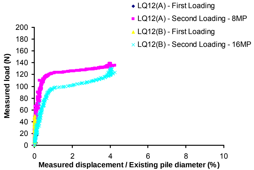
Figure 5.23 Tests LQ12(A) and LQ12(B). 1 st loading cycle – single pile foundation loaded up to working load. 2 nd loading cycle – enhanced pile foundation: Test LQ12(A) eight 200mm long mini-piles with 2D spacing; Test LQ12(B) sixteen 200mm long mini-piles with 2D spacing.
