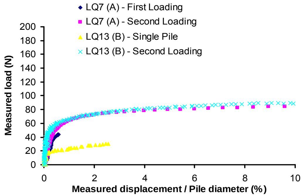
Figure 6.10 Tests LQ7(A) and LQ13(B) single pile foundations subjected to 1 st and 2 nd loading. The piles were subjected to working load during the 1 st cycle. The piles were loaded to failure during the 2 nd cycle.
