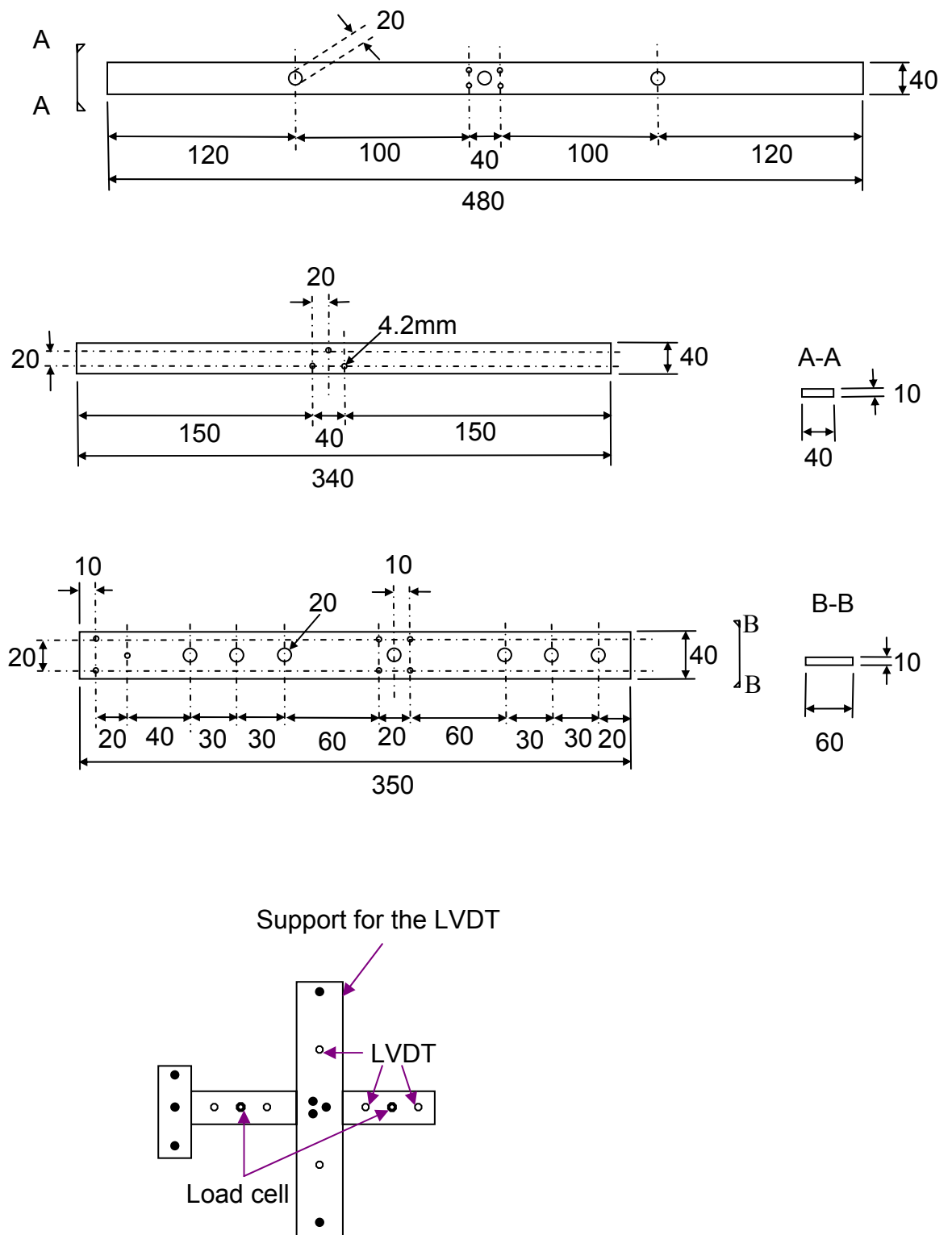
Figure 3.23 Details of aluminium beams used for supporting Linearly Variable Differential Transformers used for centrifuge model testing.
