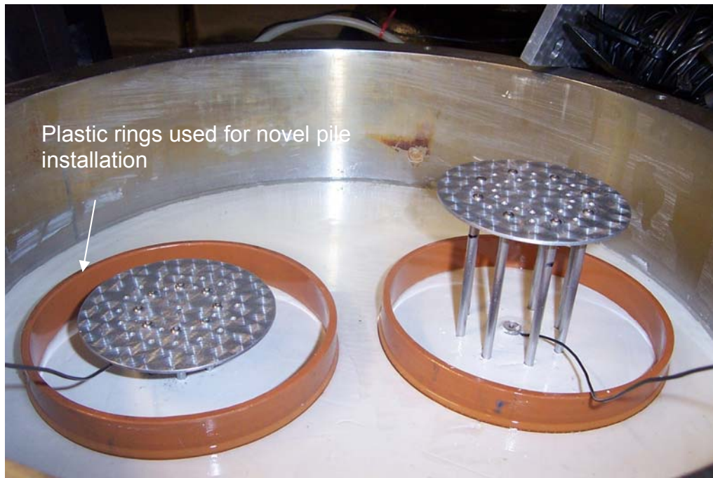
Figure 4.12 Plastic rings used to prevent the surface oil getting into bored holes during the installation of the model piles, after the model was spun up in centrifuge.
