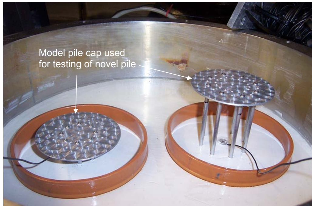
Figure 3.60 100mm diameter aluminum plate used when testing the performance of novel pile groups.
