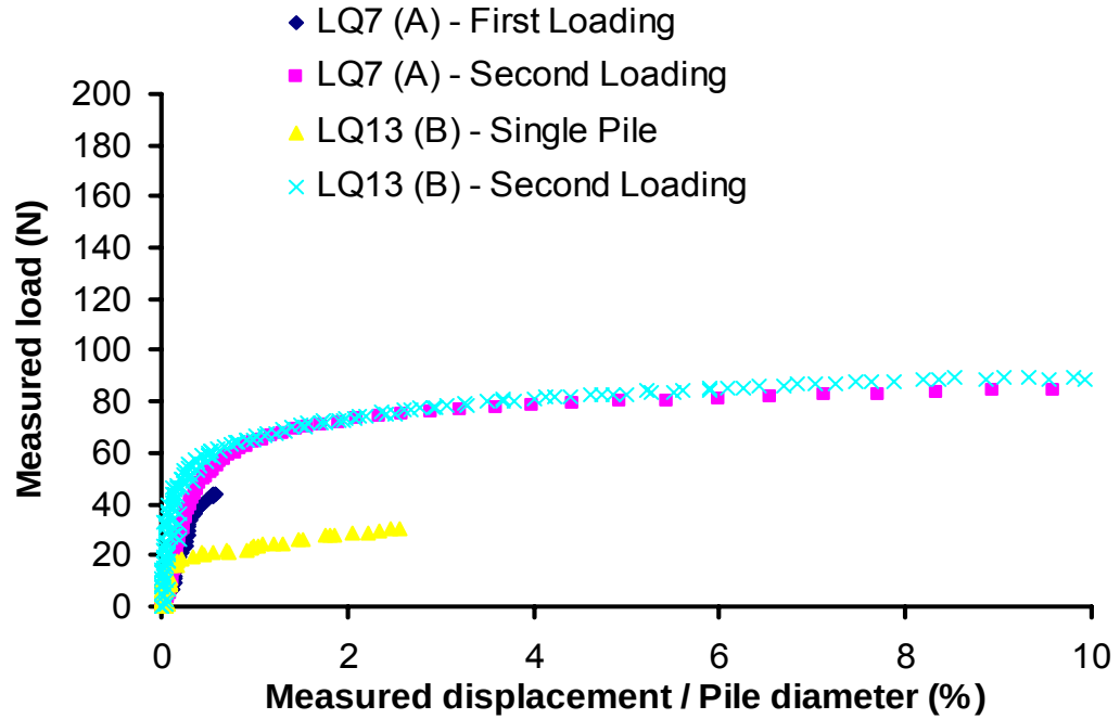
Figure 4.16 Tests LQ7(A) and LQ13(B) single pile foundations subjected to 1 st loading and 2 nd loading. The piles were subjected to working load during the 1 st cycle. The piles were loaded to failure during the 2 nd cycle.
