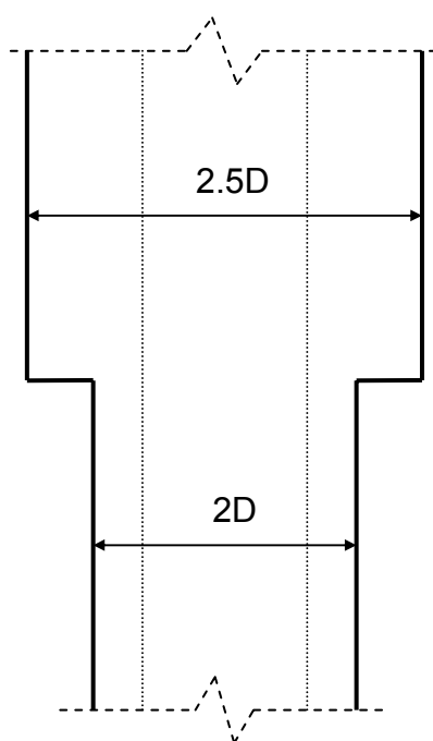
Figure 5.21 Effective geometry of the enhanced centre pile with 200mm long mini-piles installed at 2D centre to centre spacing with the existing centre pile.
