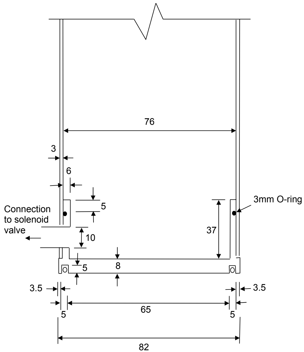
Figure 3.30 Base of the loading reservoir and details of the connection to solenoid valves.
