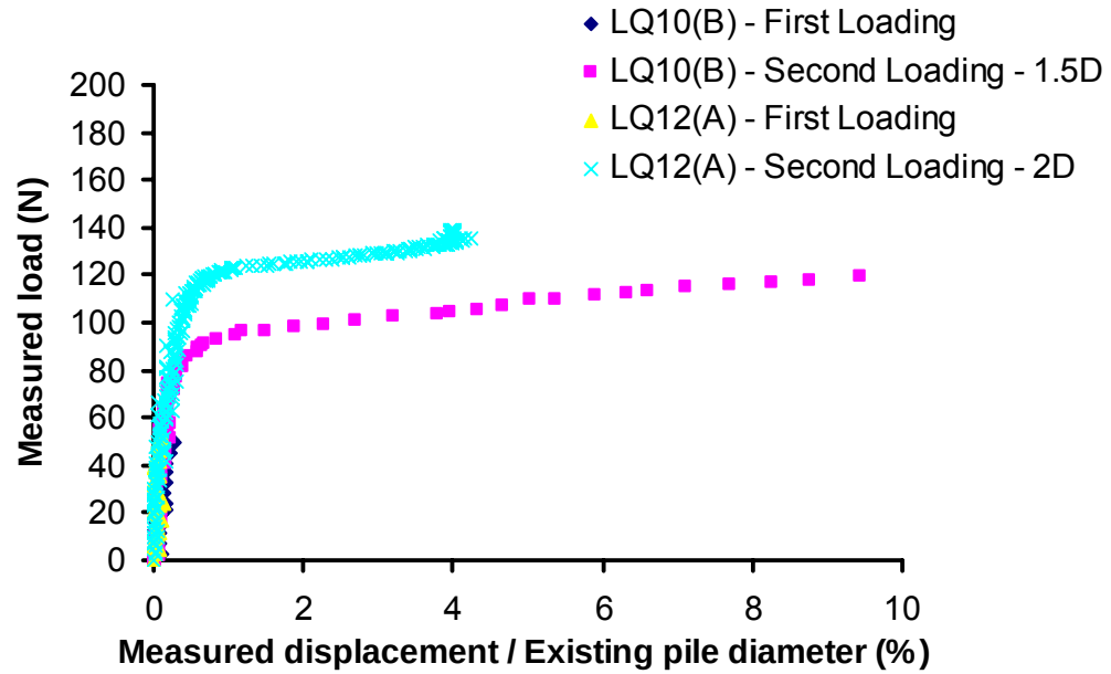
Figure 4.24 Tests LQ10(B) and LQ12(A). 1 st loading cycle – single pile foundations loaded up to working load. 2 nd loading cycle – enhanced pile foundations with eight 200mm long mini-piles. Test LQ10(B) with 1.5D pile spacing. Test LQ12(A) with 2D pile spacing.
