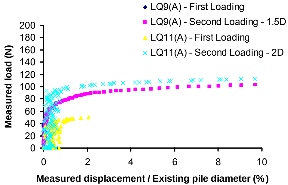
Figure 6.11 1 st loading cycle - single pile foundation loaded up to working load (FOS=2.0), tests LQ9(A) and LQ11(A). 2 nd loading cycle – enhanced pile foundations with 8 mini-piles 100mm long, test LQ9(A) with 1.5D spacing and test LQ11(A) with 2D spacing.
