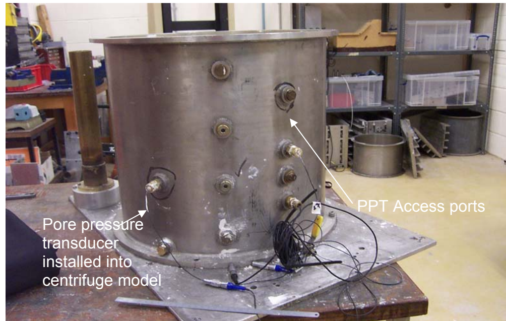
Figure 4.33 Centrifuge stainless steel tub with access ports through which the pore pressure transducers were installed.
