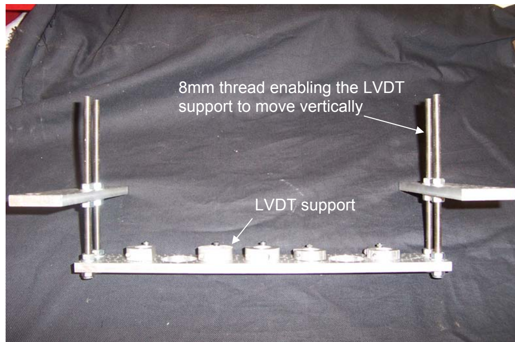
Figure 3.36 The LVDT support beam connected to 8mm threaded rod with the ability to move vertically depending on the thickness of the clay model.
