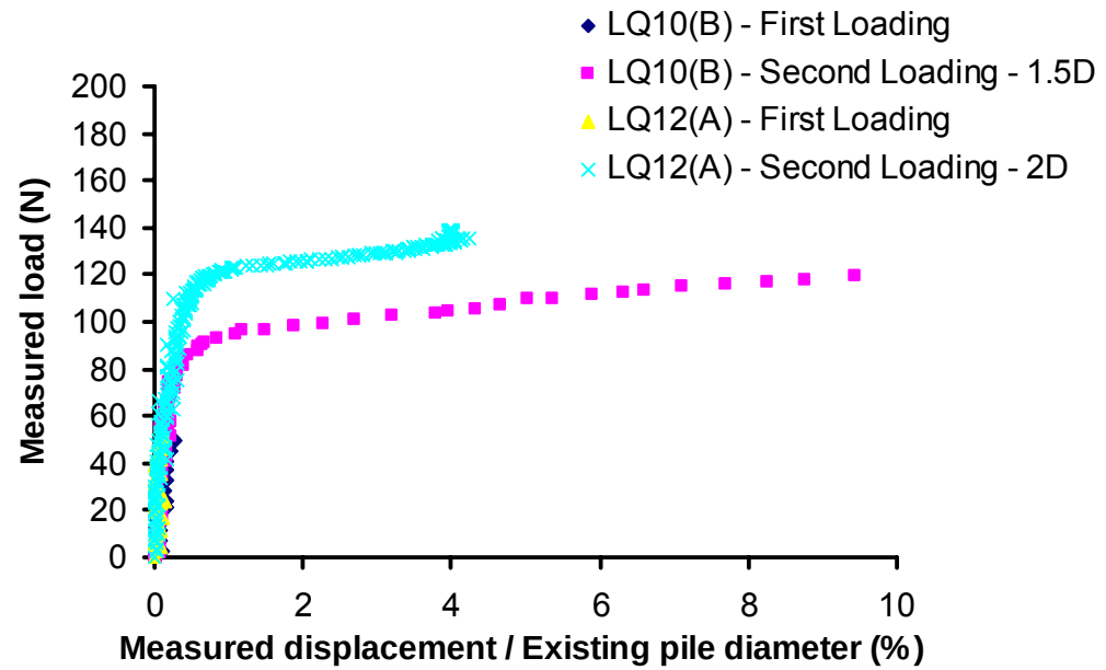
Figure 5.14 1 st loading cycle - single pile foundation loaded up to working load (FOS=2.0), tests LQ10(B) and LQ12(A). 2 nd loading cycle – enhanced pile foundations with 8 mini-piles 200mm long, test LQ10(B) with 1.5D spacing and test LQ12(A) with 2D spacing.
