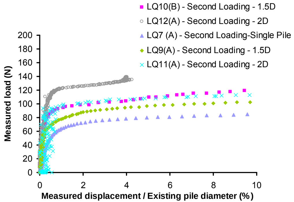
Figure 5.15 The performance of tests LQ7(A), LQ9(A), LQ10(B) and LQ12(A) during second loading cycle. During testing only the existing centre pile was loaded.
