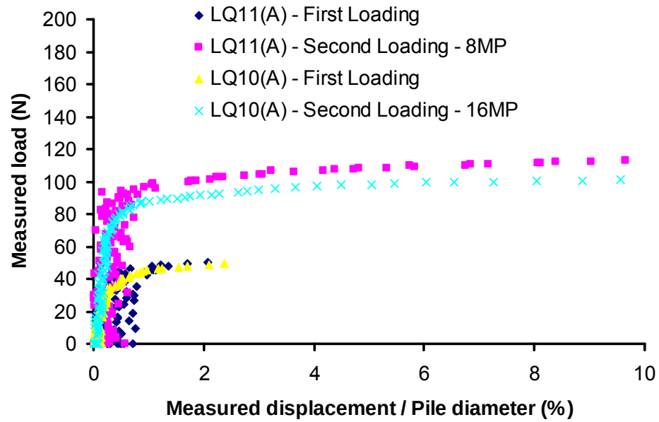
Figure 6.13 Tests LQ10(A) and LQ11(A). 1 st loading cycle – single pile foundations loaded up to working load. 2 nd loading cycle – enhanced piled foundations loaded to failure: test LQ10(A) enhanced pile foundation with sixteen 100mm long mini-piles at 3D spacing and test LQ11 enhanced pile foundation with eight 100mm long mini-piles at 3D spacing.
