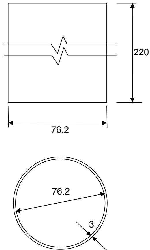
Figure 3.26 76.2 mm diameter plastic loading reservoir.
