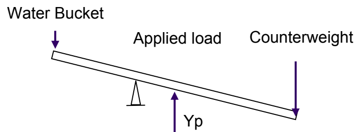
Figure 4.8 Mechanism of foundation loading device by Morrison (1994).
