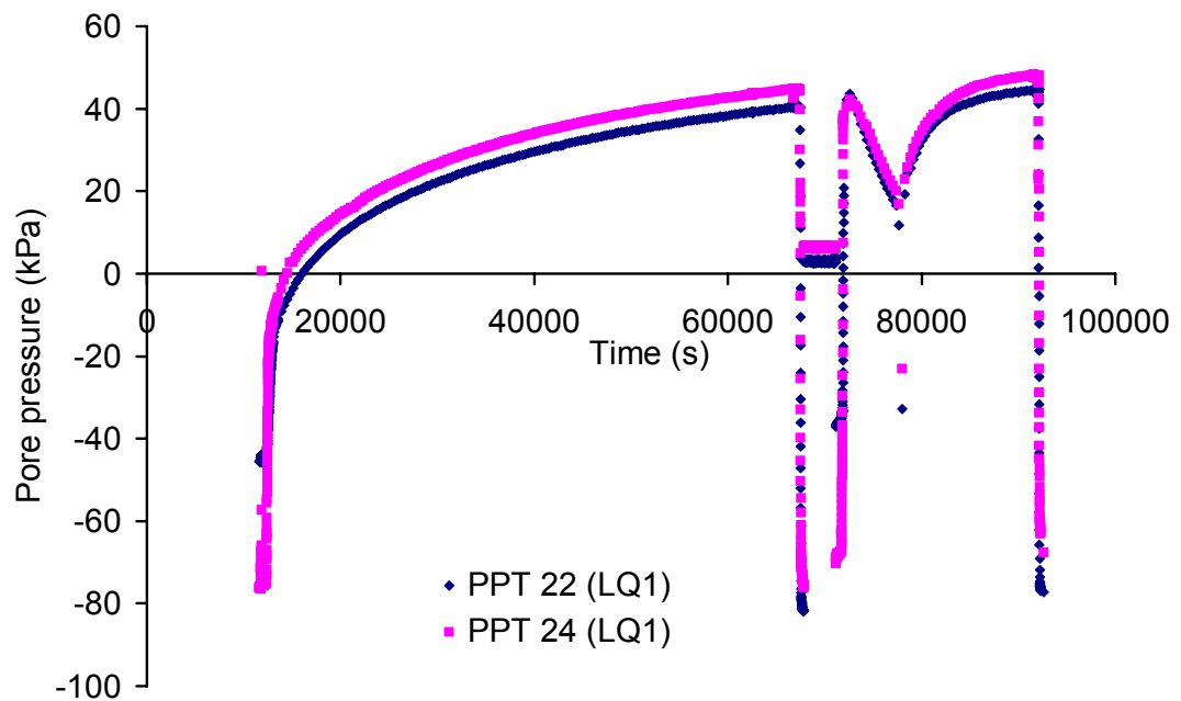
Figure 4.34 Typical pore pressure measurements with time during centrifuge model testing (Test LQ1).
