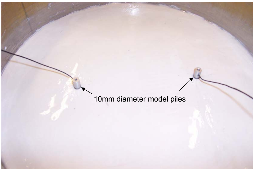
Figure 3.44 10mm diameter piles embedded 200mm into the soil sample
