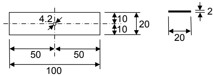
Figure 3.56 100mm by 20mm aluminium plate used when testing the performance of single model pile foundation.
