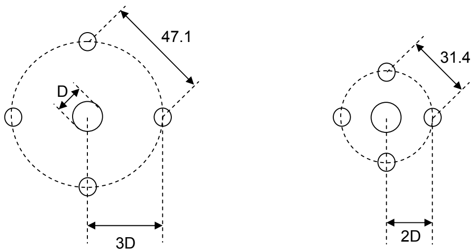
Figure 4.2 Examples of the geometry of the novel pile groups tested.
