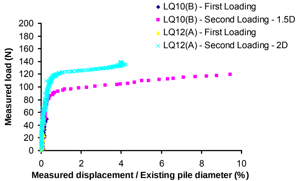
Figure 6.12 1 st loading cycle - single pile foundation loaded up to working load (FOS=2.0), tests LQ10(B) and LQ12(A). 2 nd loading cycle – enhanced pile foundations with 8 mini-piles 200mm long, test LQ10(B) with 1.5D spacing and test LQ12(A) with 2D spacing.
