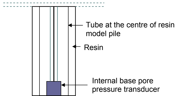
Figure 3.41 Proposed design for resin model piles to be used for centrifuge model testing.
