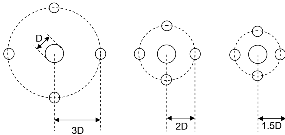
Figure 4.17 Details of the geometry of the novel pile groups used to investigate the influence of centre to centre spacing between the centre pile and the mini-pile group.
