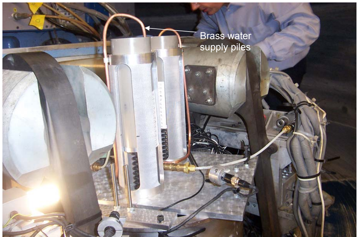
Figure 3.29 Brass pipes, connected to centrifuge slip rings, used to fill the loading reservoirs with water during centrifuge model testing.
