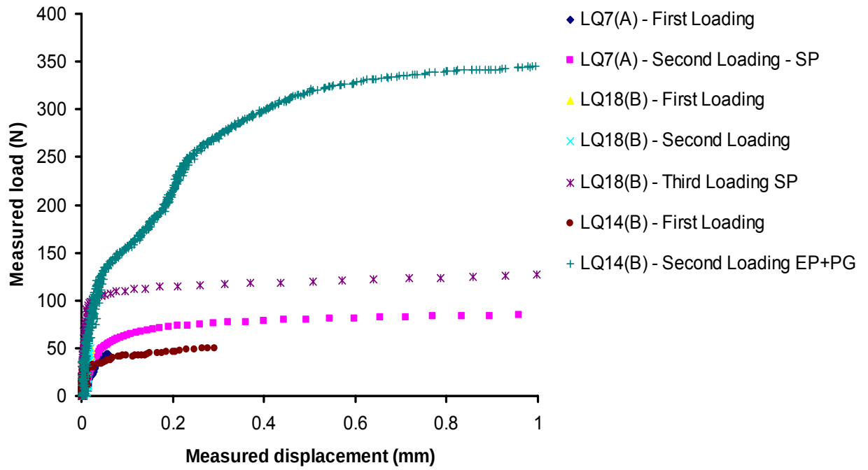
Figure 6.20 Tests LQ7(A), LQ14(B) and LQ18(B). 1 st loading cycle – single pile foundation. 2 nd loading cycle – Test LQ7(A) single pile foundation; Test LQ14(B) novel pile group (centre pile enhanced with eight 100mm long mini-piles with 3D spacing; Test LQ18(B) single pile foundation (centrifuge was not stopped between the first and second loading cycle). 3 rd loading cycle – test LQ18(B) centre pile enhanced with eight 100mm long mini-piles with 3D spacing.
