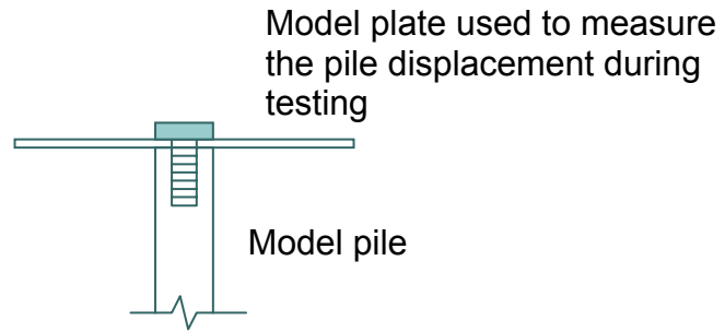
Figure 3.58 Details of connection of the model plate and aluminium model pile.
