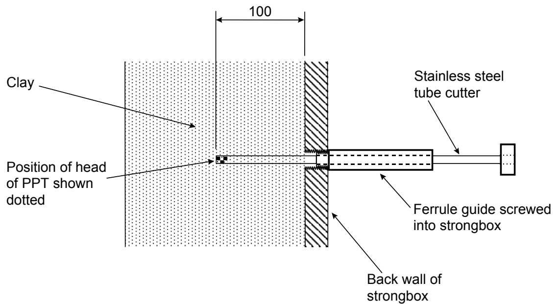
Figure 3.67 Method of ensuring correct positioning of pore pressure transducers within model (McNamara, 2001).
