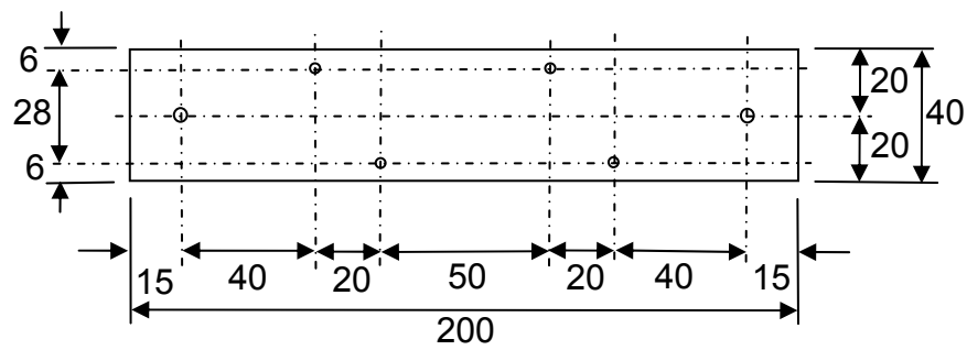
Figure 3.32 Aluminium plate used to connect the solenoid valves to the loading apparatus.
