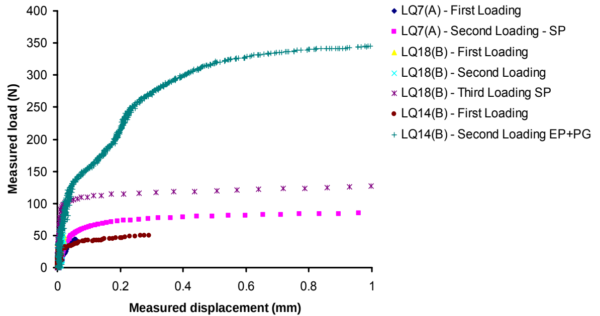
Figure 4.30 Tests LQ7(A), LQ14(B) and LQ18(B). 1 st loading cycle – single pile foundation. 2 nd loading cycle – Test LQ7(A) single pile foundation; Test LQ14(B) novel pile group (centre pile enhanced with eight 100mm long mini-piles with 3D spacing; Test LQ18(B) single pile foundation (centrifuge was not stopped between the first and second loading cycle). 3 rd loading cycle – test LQ18(B) centre pile enhanced with eight 100mm long mini-piles with 3D spacing.
