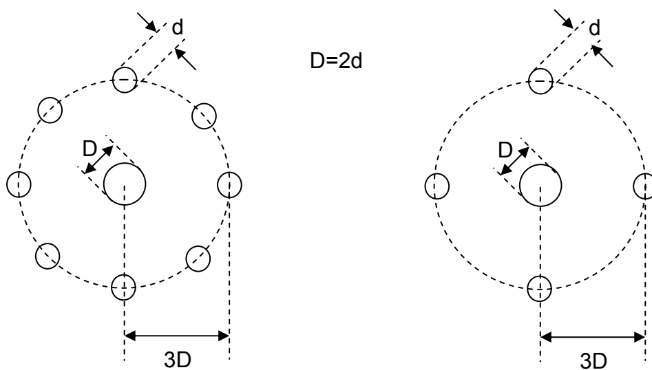
Figure 5.29 Examples of geometry of centrifuge model used to investigate caisson effect.
