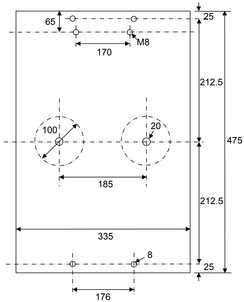
Figure 3.33 12mm thick aluminium plate used to support the loading apparatus and solenoid valves.
