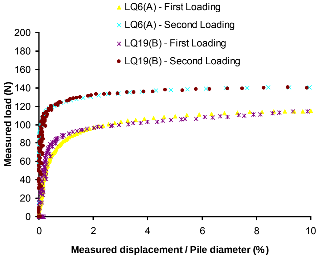
Figure 6.21 Performance of single pile foundations during 1 st and 2 nd loading. Test LQ6(A) – centrifuge was stopped between the first and second loading. Test LQ19(B) – centrifuge was NOT stopped between the first and second loading.
