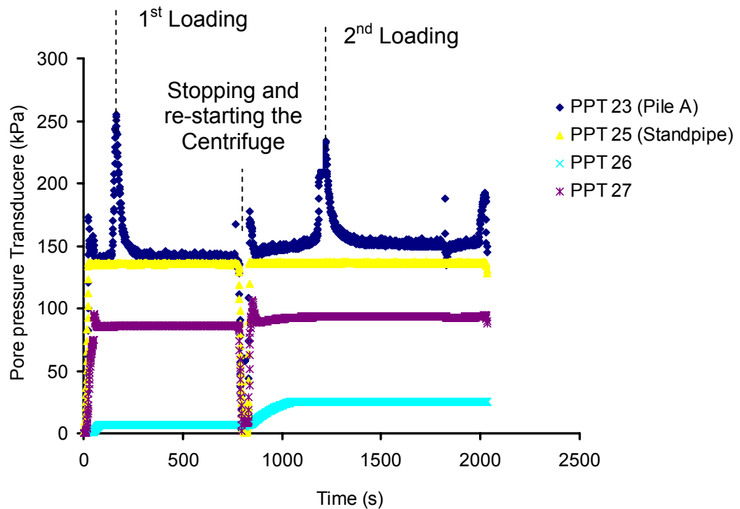
Figure 5.4 Pore pressure transducer response during centrifuge model testing.
