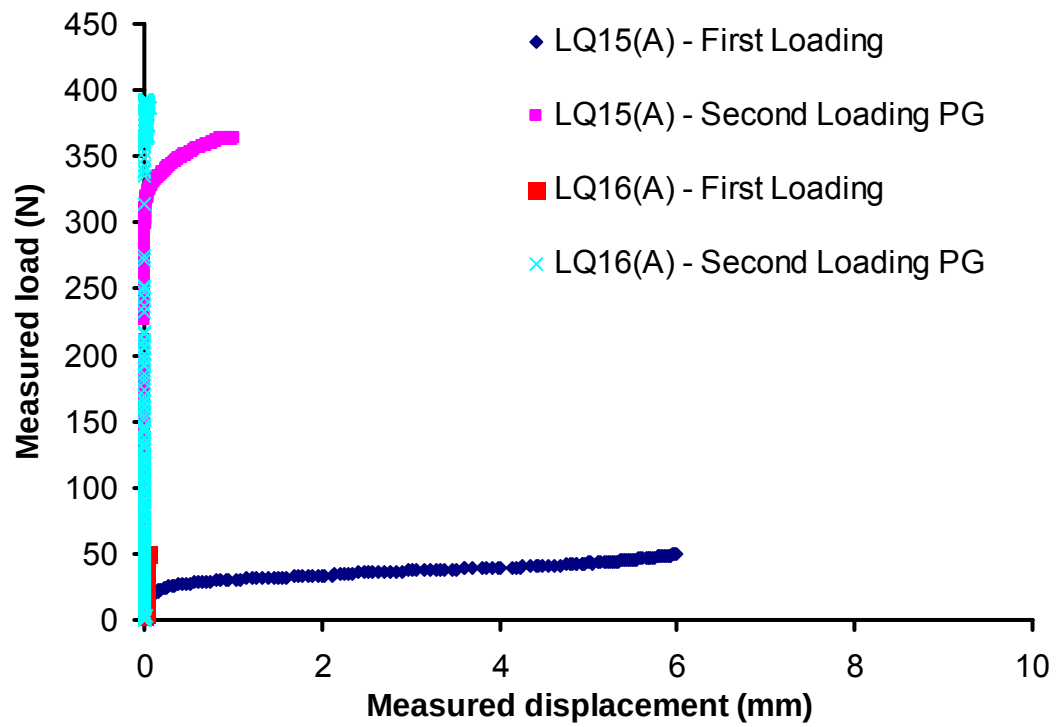
Figure 6.17 Tests LQ15(A) and LQ16(A). 1 st loading cycle – single pile foundations loaded up to working load. 2 nd loading cycle – novel pile group: Test LQ15(A) eight 200mm long mini-piles with 3D spacing; Test LQ16(A) four 200mm long mini-piles with 3D spacing.
