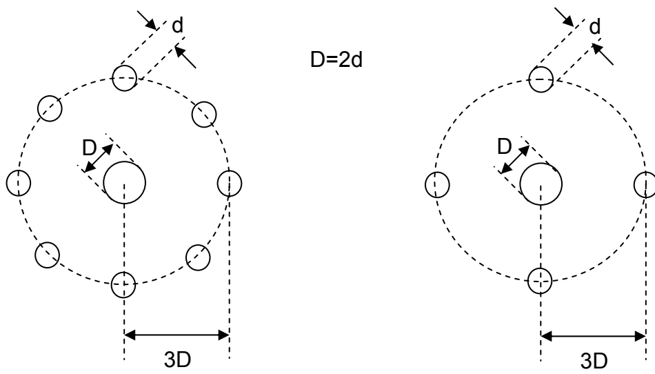
Figure 4.1 Geometry of the centrifuge model; groups of eight and four mini-piles.
