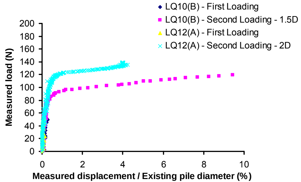
Figure 4.19 1 st loading cycle - single pile foundation loaded up to working load (FOS=2.0), tests LQ10(B) and LQ12(A). 2 nd loading cycle – enhanced pile foundations with 8 mini-piles 200mm long, test LQ10(B) with 1.5D spacing and test LQ12(A) with 2D spacing.
