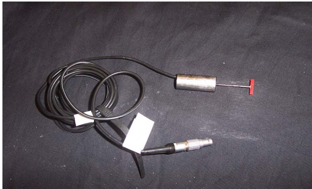
Figure 3.65 LVDT used for centrifuge model testing.
