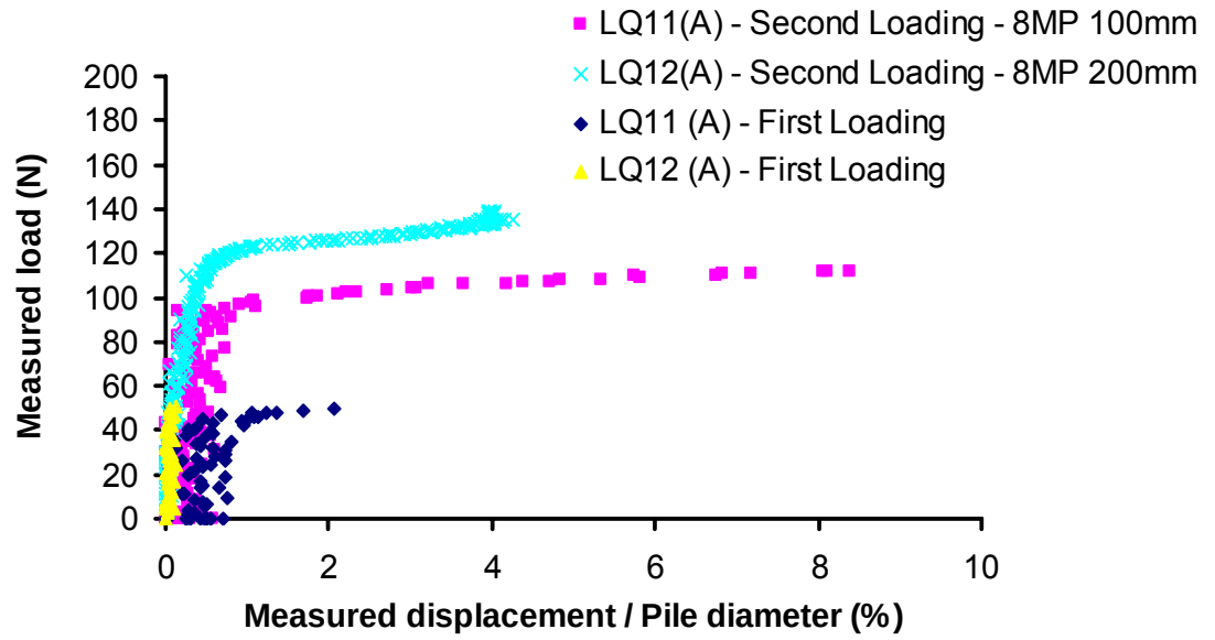
Figure 5.27 Tests LQ11(A) and LQ12(A). 1 st loading cycle – single pile foundation loaded up to working load. 2 nd loading cycle – enhanced pile foundation: Test LQ11(A) eight 100mm long mini-piles with 2D spacing; Test LQ12(A) eight 200mm long mini-piles with 2D spacing.
