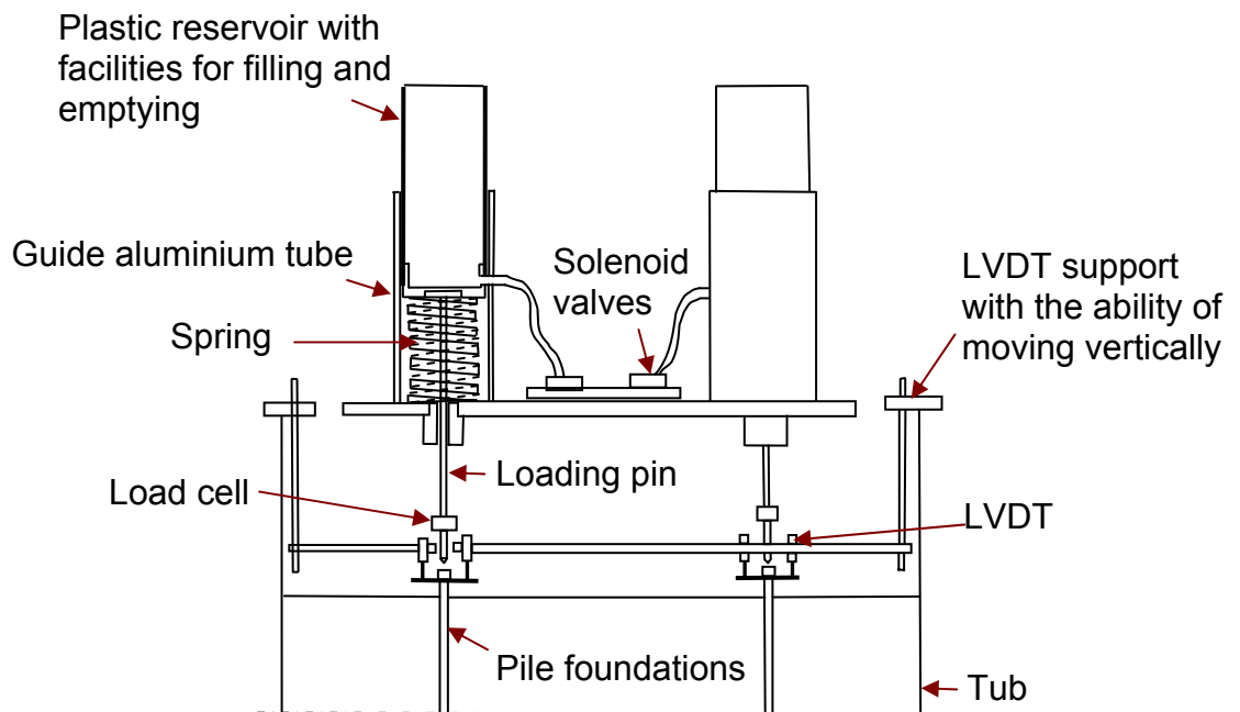
Figure 4.10 New loading apparatus developed for centrifuge model testing.
