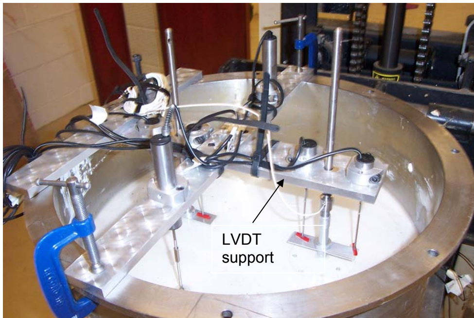
Figure 3.22 Linearly Variable Differential Transformers (LVDT) support clamped at the flange of the tub used for the first centrifuge model test.
