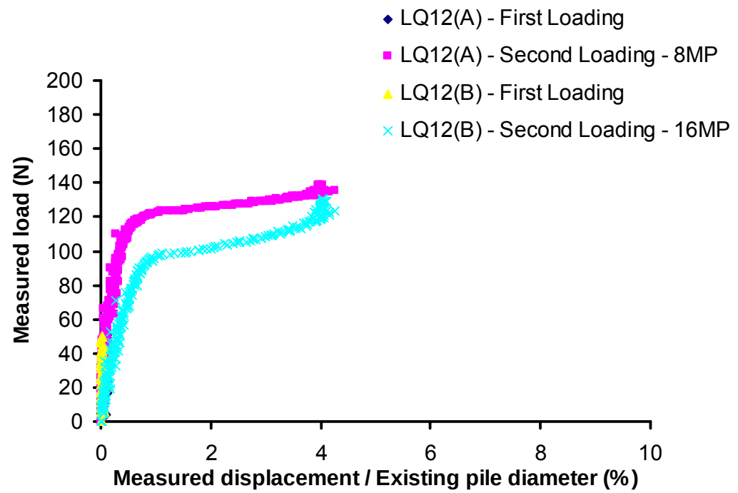
Figure 4.22 Tests LQ12(A) and LQ12(B). 1 st loading cycle – single pile foundation loaded up to working load. 2 nd loading cycle – enhanced pile foundation: Test LQ12(A) eight 200mm long mini-piles with 2D spacing; Test LQ12(B) sixteen 200mm long mini-piles with 2D spacing.
