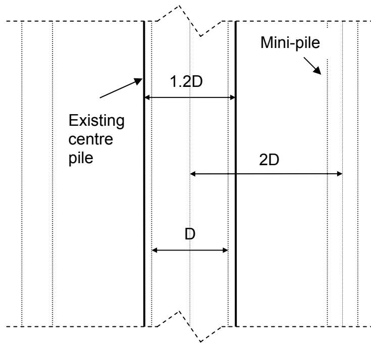
Figure 5.31 Test LQ17(A). Novel pile group with four 200mm mini-piles at 2D centre to centre spacing with the existing centre pile.
