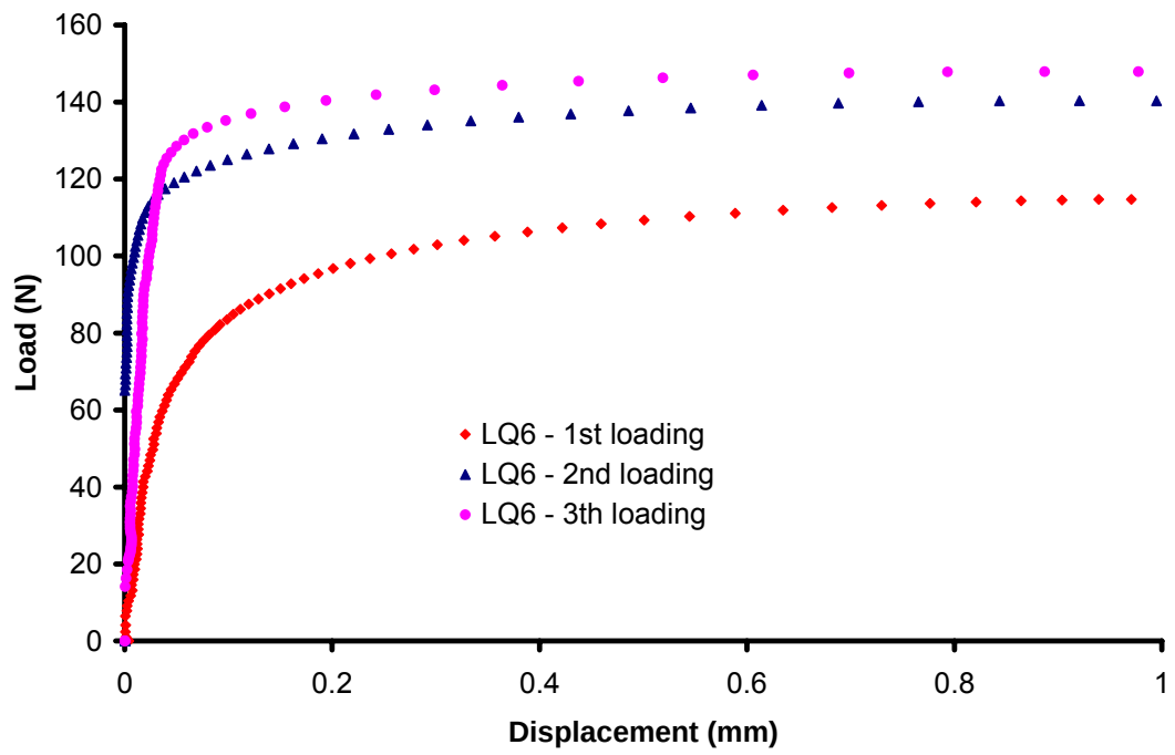
Figure 5.12 Tests LQ6 – Single pile foundations subjected to three loading cycles.
