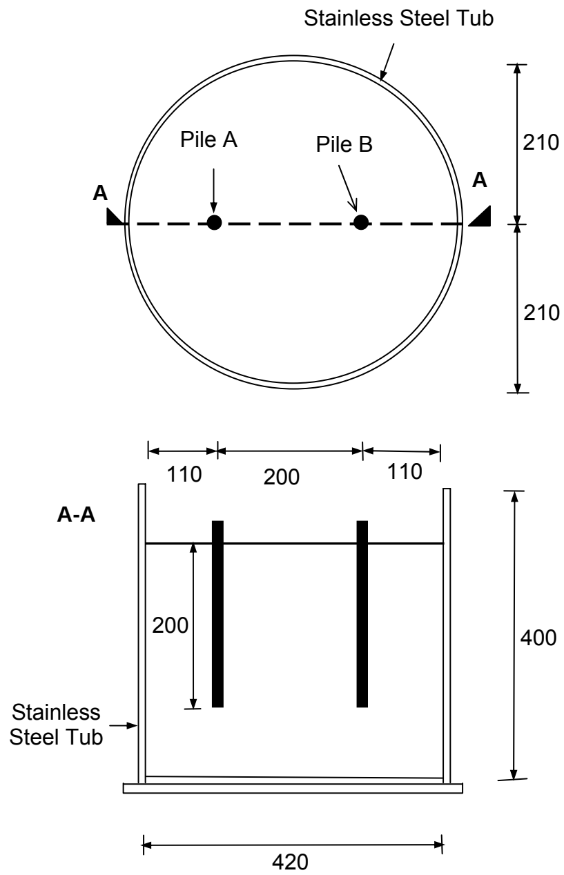
Figure 5.1 Geometry of a typical model used for centrifuge testing.
