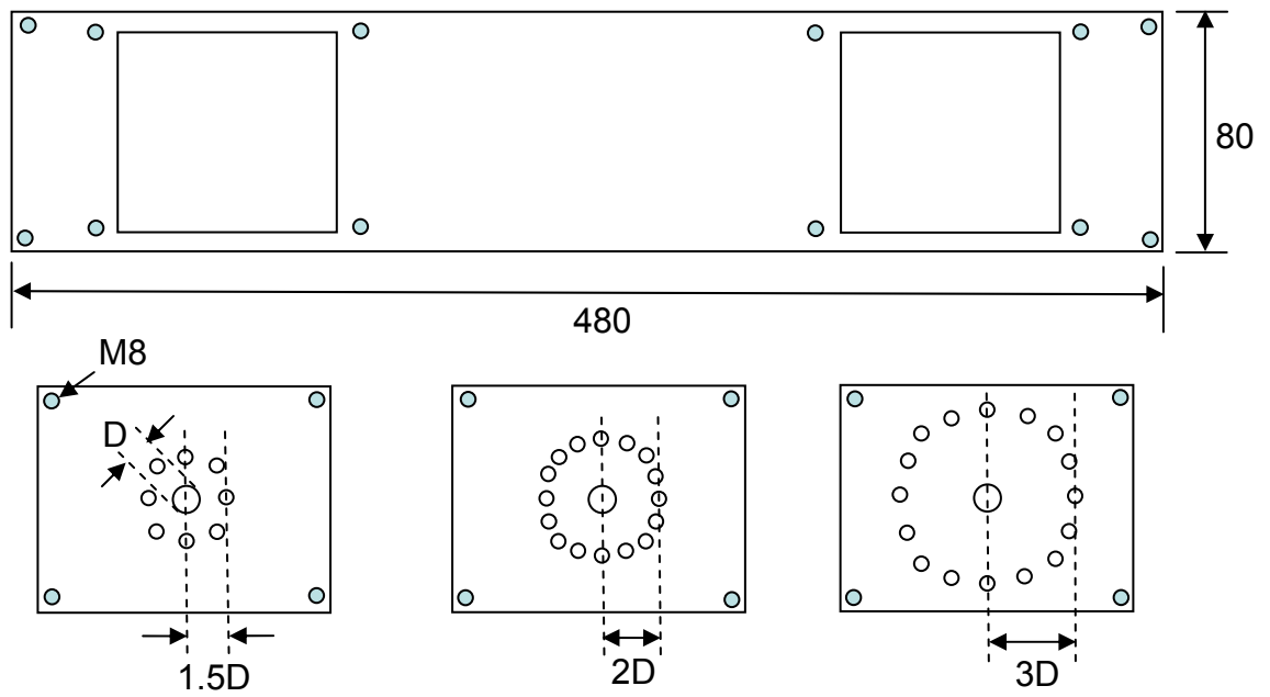
Figure 3.47 Detail of jig used for model pile installation.
