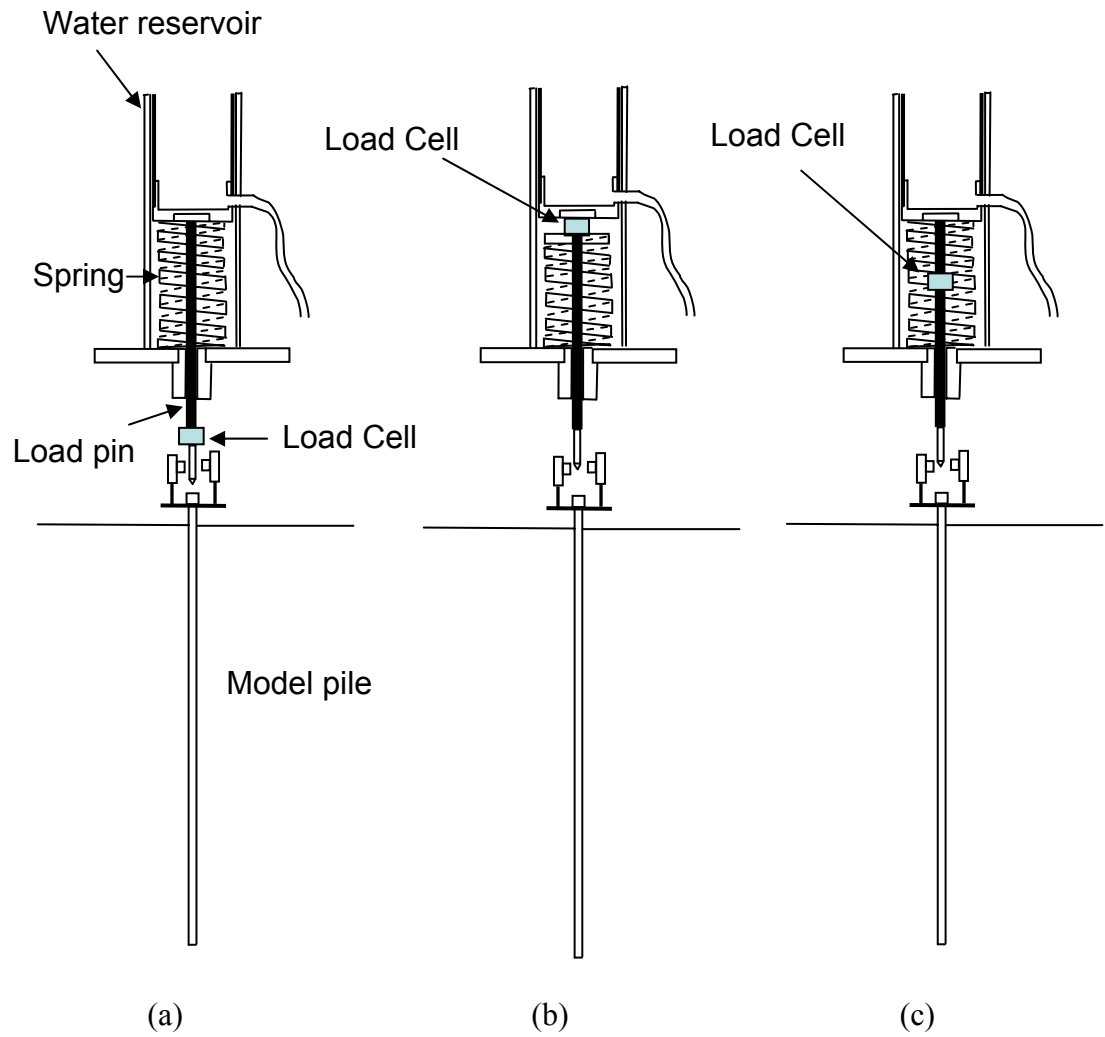
Figure 4.15 Details of the geometry of the loading apparatus for tests: (a) LQ1 to LQ19, (b) LQ20 and (c) LQ21.
