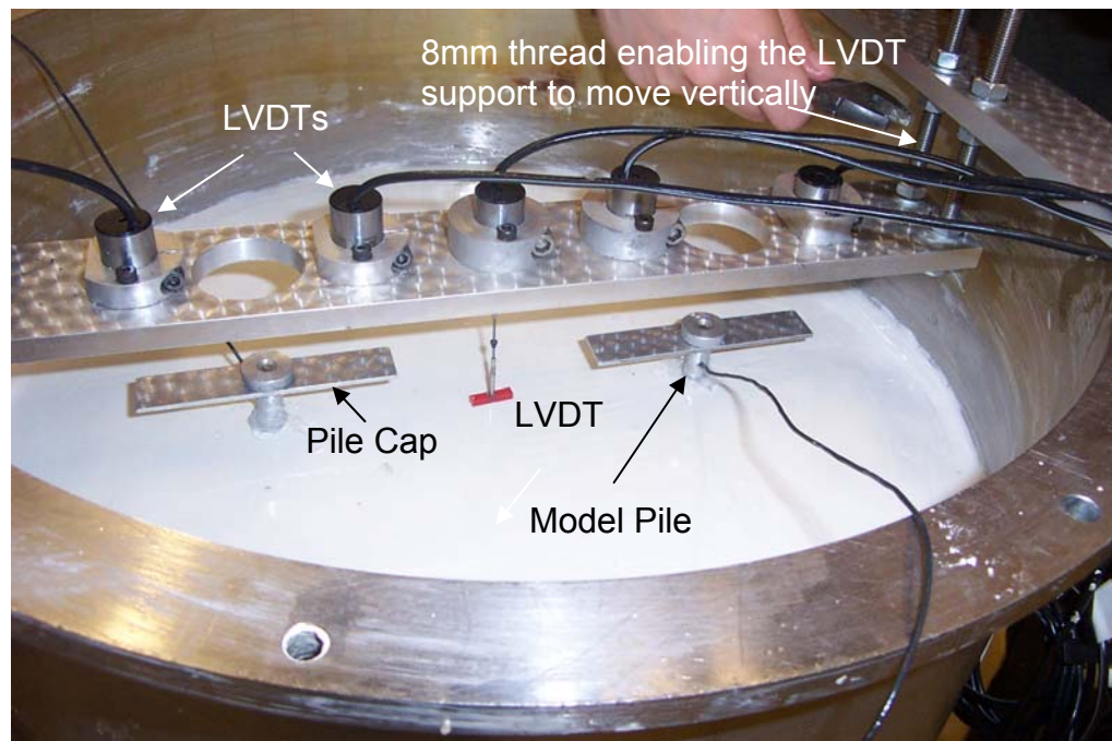
Figure 5.3 The LVDTs used to measure pile settlements during loading and changes in the model soil surface during testing.
