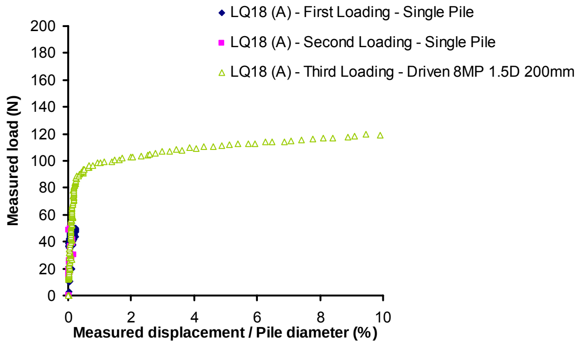
Figure 4.13 Test LQ18(A). Pile foundations subjected to three loading cycles. The centrifuge was not stopped between the first and second loading cycle.
