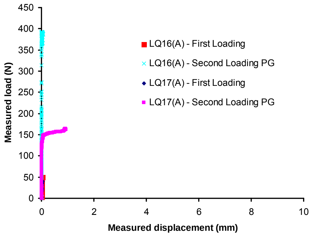
Figure 6.18 Tests LQ16(A) and LQ17(A). 1 st loading cycle – single pile foundations. 2 nd loading cycle – novel pile group: Test LQ16(A) eight 200mm long mini-piles with 3D spacing; Test LQ17(A) four 200mm long mini-piles with 3D spacing.
