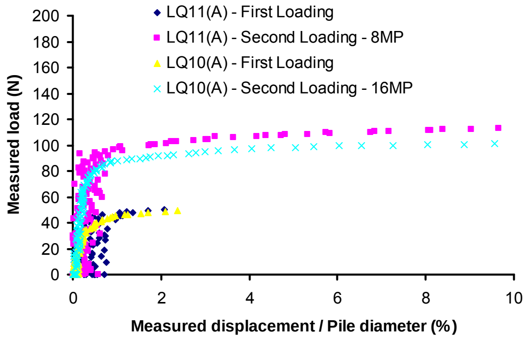
Figure 5.22 Tests LQ11(A) and LQ10(A). 1 st loading cycle – single pile foundation loaded up to working load. 2 nd loading cycle – enhanced pile foundation: Test LQ11(A) eight 100mm long mini-piles with 2D spacing; Test LQ10(A) sixteen 100mm long mini-piles with 2D spacing.
