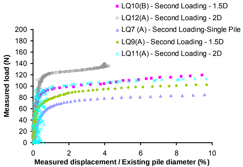
Figure 4.20 The performance of tests LQ7(A), LQ9(A), LQ10(B) and LQ12(A) during second loading cycle. During testing only the existing centre pile was loaded.
