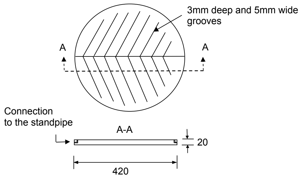
Figure 3.40 Drainage base plate.
