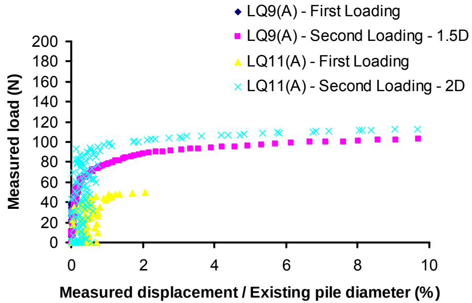
Figure 5.13 1 st loading cycle - single pile foundation loaded up to working load (FOS=2.0), tests LQ9(A) and LQ11(A). 2 nd loading cycle – enhanced pile foundations with 8 mini-piles 100mm long, test LQ9(A) with 1.5D spacing and test LQ11(A) with 2D spacing.
