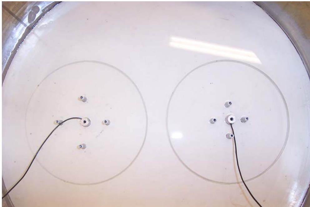
Figure 6.5 Enhanced existing model pile foundations, after initial loading, with mini-pile groups.
