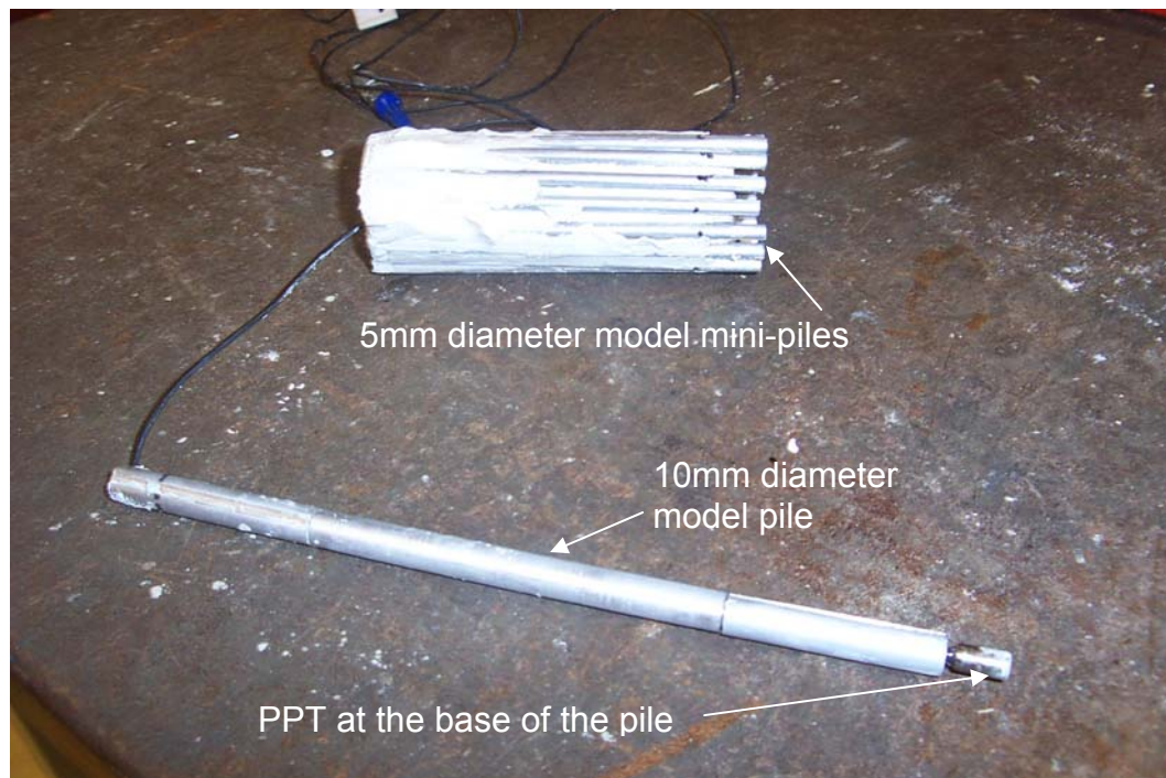
Figure 4.5 Model pile made of aluminium sections with the pore pressure transducer at the base.
