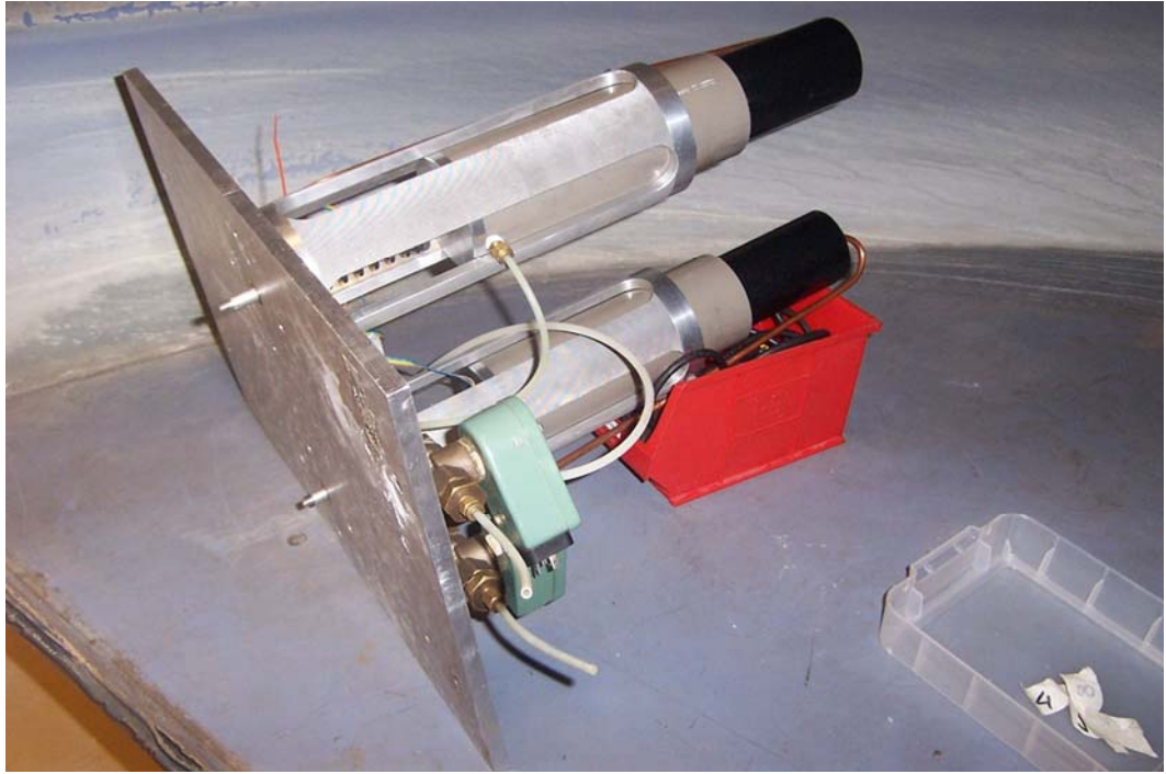
Figure 3.34 Loading reservoirs, guide tubes, springs and solenoid valves put together prior to mounting on the centrifuge tub.
