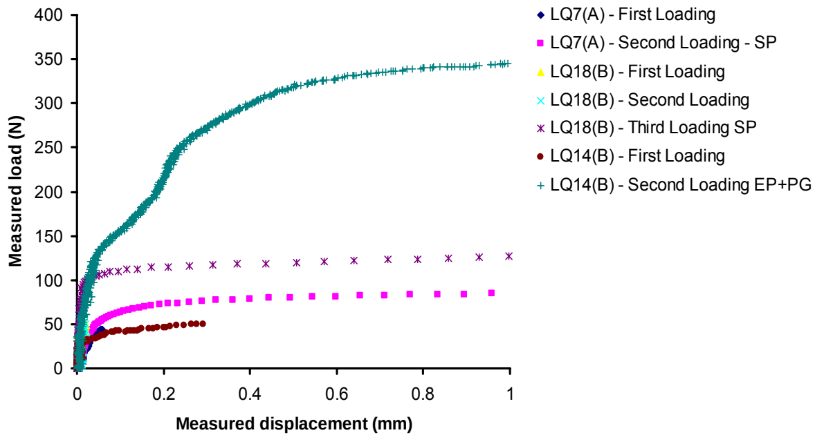
Figure 5.34 Tests LQ7(A), LQ14(B) and LQ18(B). 1 st loading cycle – single pile foundation. 2 nd loading cycle – Test LQ7(A) single pile foundation; Test LQ14(B) novel pile group (centre pile enhanced with eight 100mm long mini-piles with 3D spacing; Test LQ18(B) single pile foundation (centrifuge was not stopped between the first and second loading cycle). 3 rd loading cycle – test LQ18(B) centre pile enhanced with eight 100mm long mini-piles with 3D spacing.
