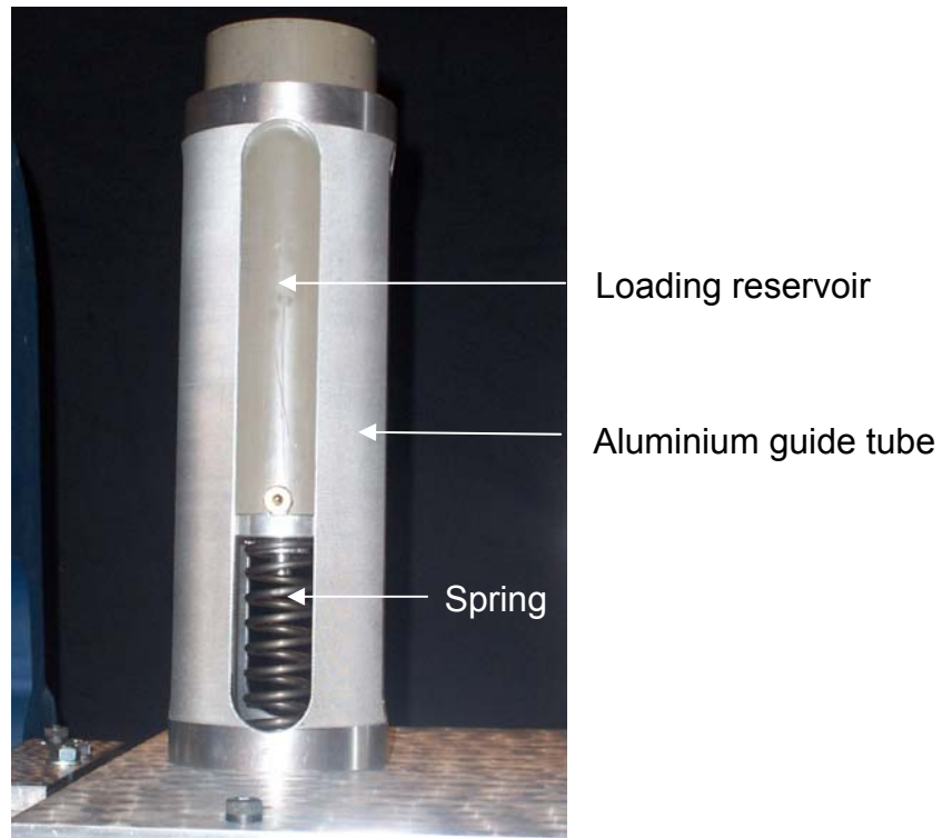
Figure 3.27 Plastic loading reservoir supported by a spring while empty.
