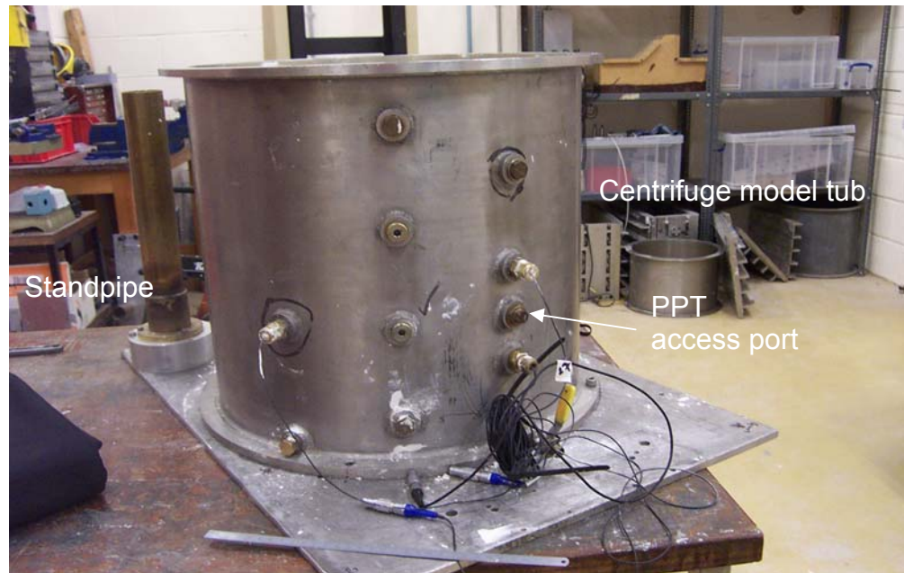
Figure 3.38 Centrifuge stainless steel tub with access ports through which the pore pressure transducers were installed.
