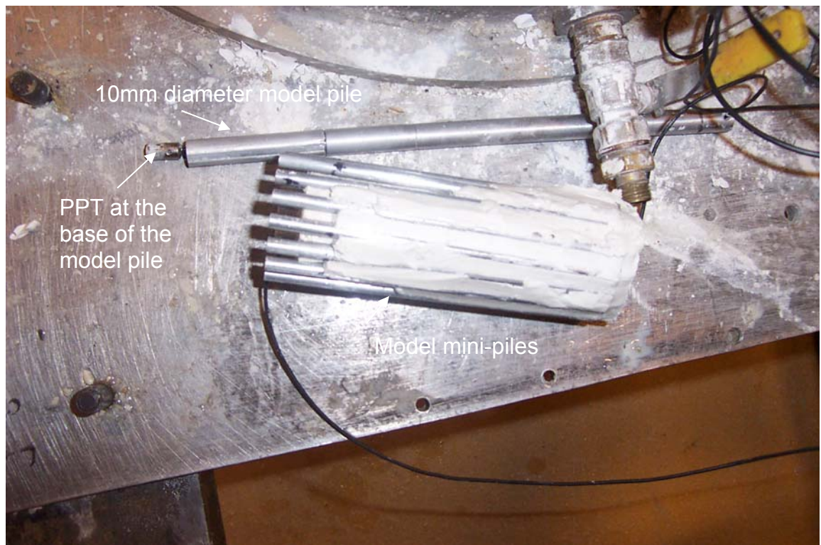
Figure 3.54 10mm diameter model with a pore pressure transducer at the base.
