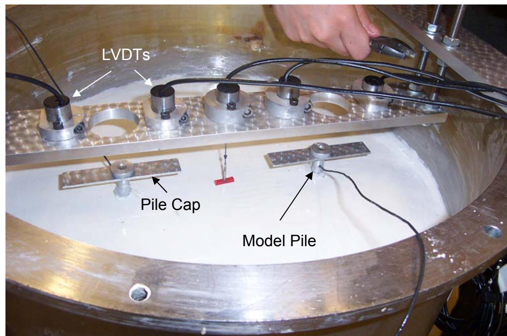
Figure 3.37 The LVDT support mounted and connected to the flange of the tub.
