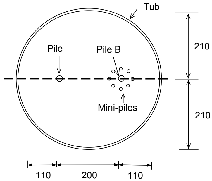
Figure 5.5 Typical geometry of model used to investigate the performance of enhanced pile foundation.
