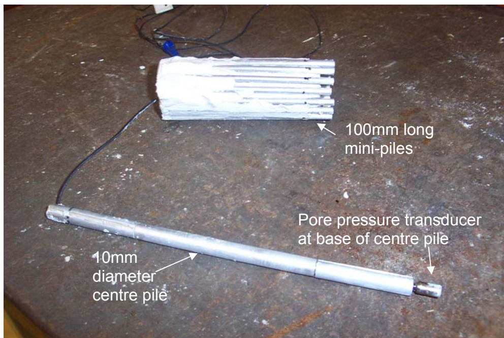
Figure 6.6 Pore pressure transducer at the tip of the model pile used in centrifuge model testing (Test LQ19).
