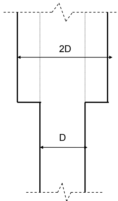
Figure 5.18 Effective geometry of the enhanced centre pile with 100mm long mini-piles installed at 1.5D centre to centre spacing with the existing centre pile.
