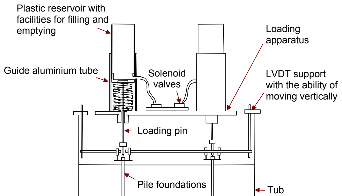
Figure 3.25 New loading apparatus developed for centrifuge model testing.
