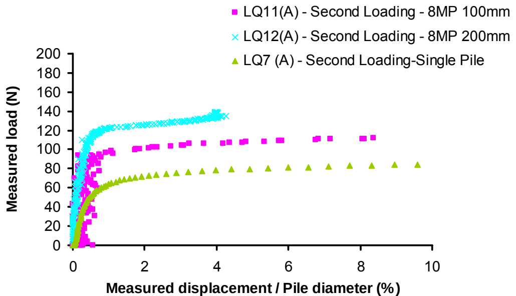
Figure 4.25 The performance of tests LQ7(A), LQ11(A) and LQ12(A) during 2 nd loading cycle. In all tests only the centre pile was loaded.
