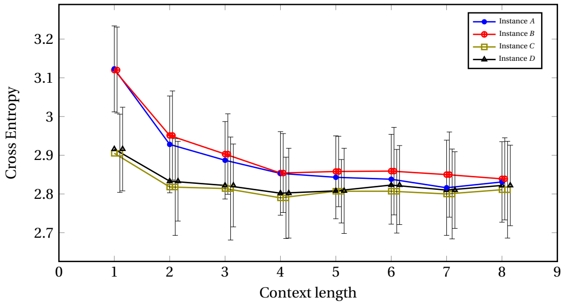
Fig. 6.2 Comparison between the predictive performances, on the Chinese folk melody dataset, of the pitch-only NPM (Instance A), its extensions which use the intfref type (Instance B) and ioi type (Instance C) as additional input, and both these types together in a single model (Instance D).
