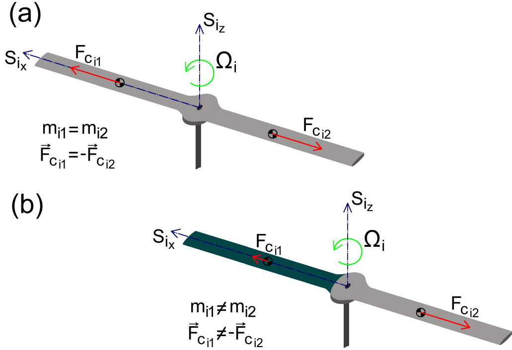
Figure 5.12: (a) Centrifugal forces acting on the two rotating blades of a compensated rotor. (b) Centrifugal force decompensation appearing in the rotor when a rotating blade with different mass is considered.
