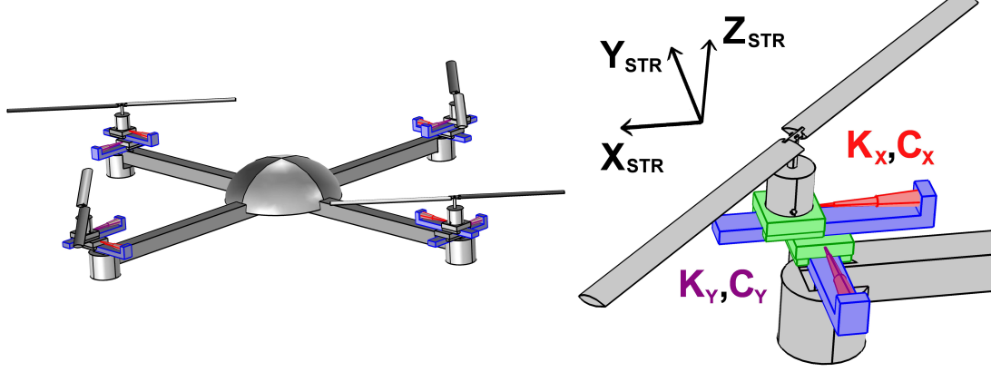
Figure 5.18: Sketch of the isolating control device located between each arm and rotor and detail of the isolating control device located in rotor S_1 , with spring and damper parameters K_{x,y} and C_{x,y} respectively.
