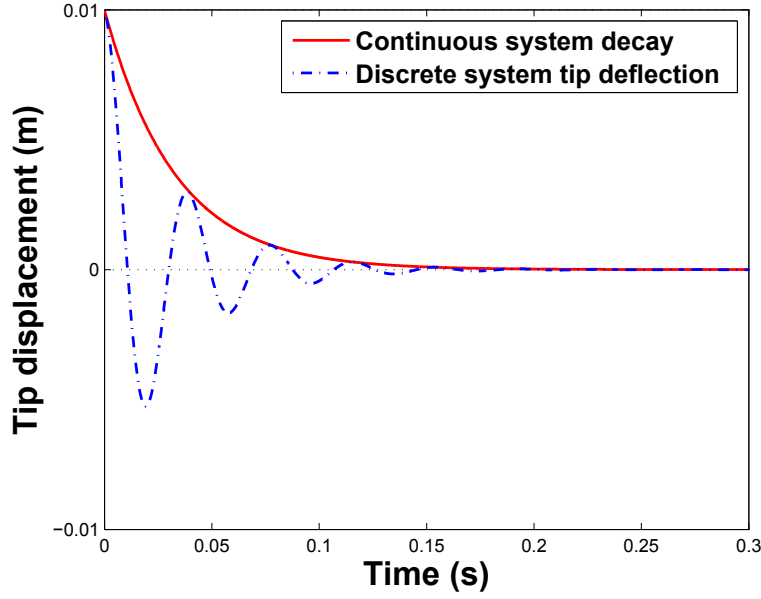
Figure 3.15: Adjusted dynamic displacement of the balsa wood discretized beam tip when initially disturbed (---) and expected decay of the continuous beam oscillations amplitude (—): A_o e^{-2\pi\xi\omega_n t}
