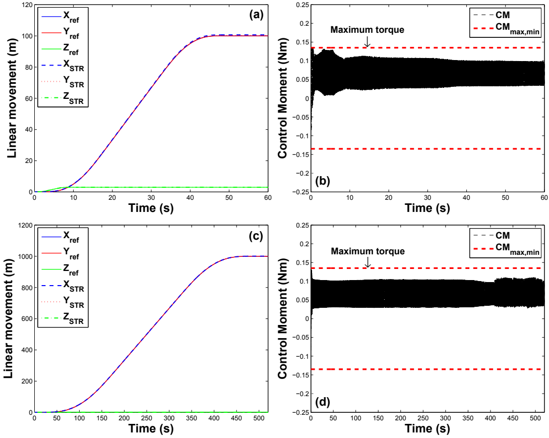
Figure 5.22: Response of the platform with the ICD installed when a complete blade is missing in rotor 1: (a) References ( X_n^{ref} = 100 m, Y_n^{ref} = 100 m, Z_n^{ref} = 3 m) and trajectory tracking. (b) Control action applied to rotor 1 for trajectories shown in (a). (c) References ( X_n^{ref} = 1000 m, Y_n^{ref} = 1000 m, Z_n^{ref} = 3 m) and trajectory tracking. (d) Control action applied to rotor 1 for trajectories shown in (c)
