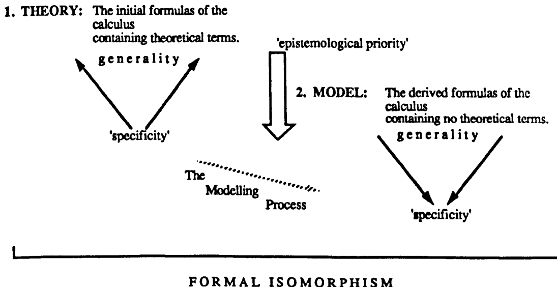
FIGURE 3.3.1b: An Interpretation of the B-N-S Model.
