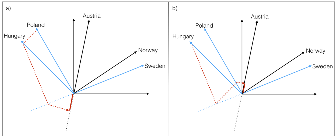
Figure 4: An illustration of how QSM can account for the results from Tversky's(1977) diagnosticity experiment. The order of projection on panel (a) is such that we start from the context elements, Poland (arbitrarily chosen first in the illustration), then Hungary, then Sweden, then Austria. If we were computing a similarity without context, we would just have a projection from Sweden to Austria, to correspond to the similarity of Sweden (first projection) to Austria. Analogously for panel (b). The key aspect of this illustration is that, when the 'grouped' elements (Poland, Hungary) are the context elements, the initial projections are such that not much amplitude is lost across successive projections (of the context elements; panel a). When the context elements are e.g. Hungary and Sweden, so that the similarity comparison concerns Poland and Austria (in the context of Hungary and Sweden), then the initial projections lead to a massive loss of amplitude, with the resulting similarity judgment being lower.
