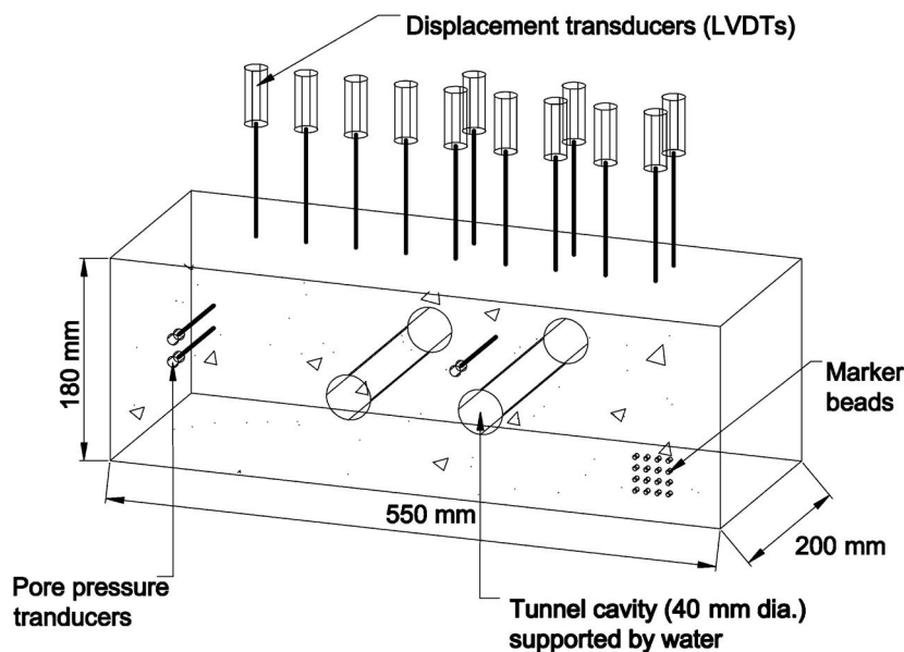
Figure 5: Schematic diagram of a typical plane strain centrifuge twin-tunnel model (not to scale), Divall and Goodey (2012)
