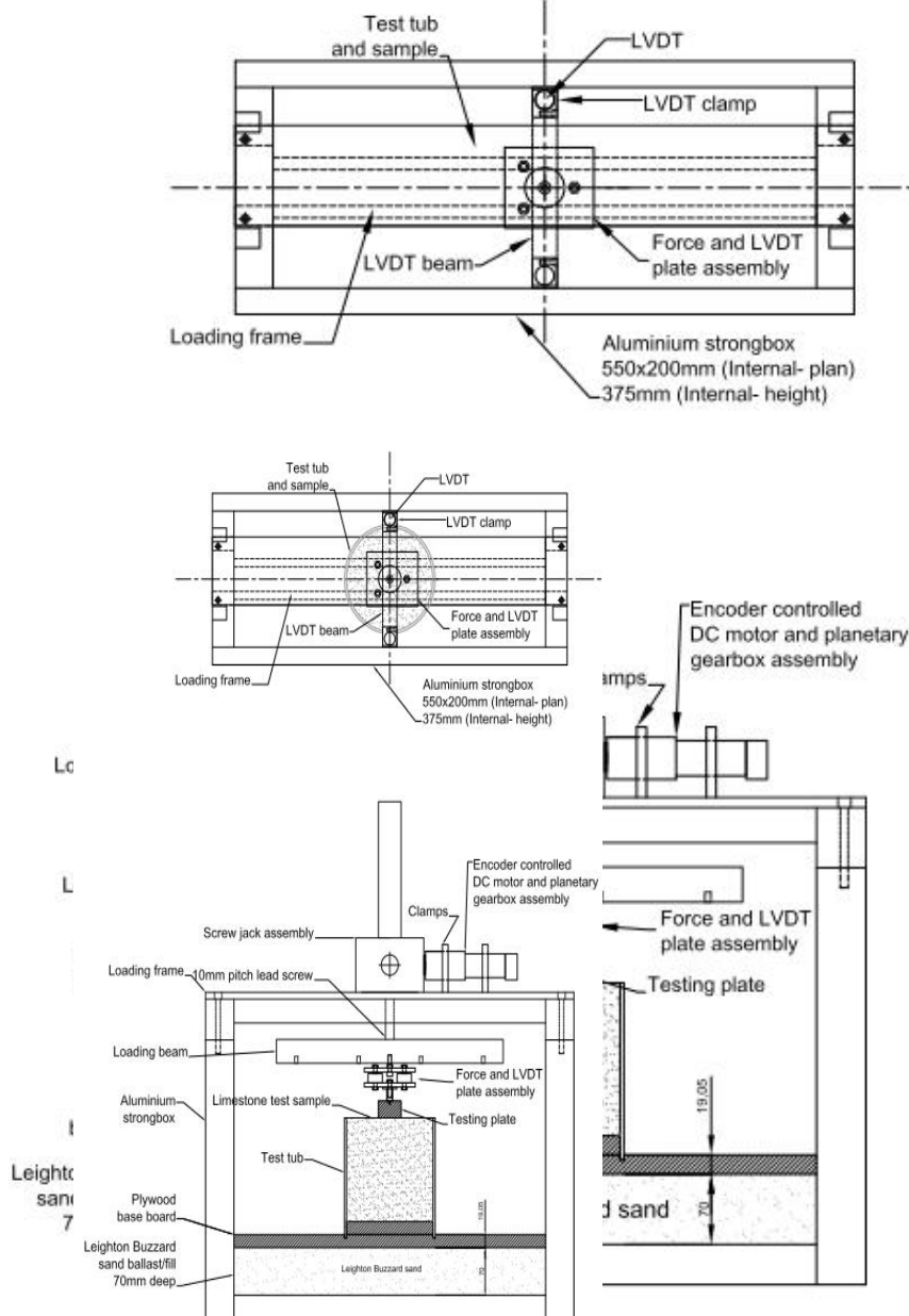
Figure 7. Assembled testing equipment and instrumentation.
