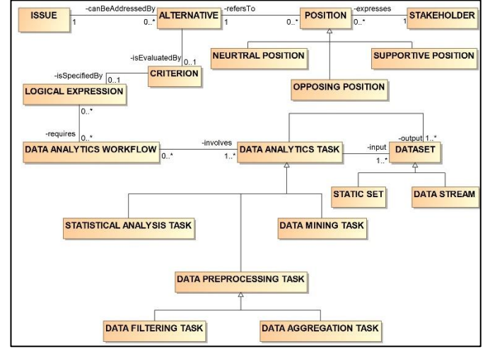
Figure 2 Main Classes of the Ontology Framework
