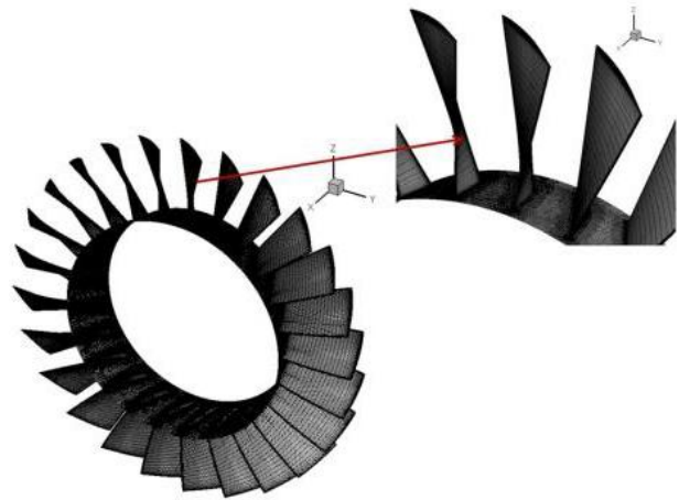
Fig. 3: Partial mesh views for the first rotor
