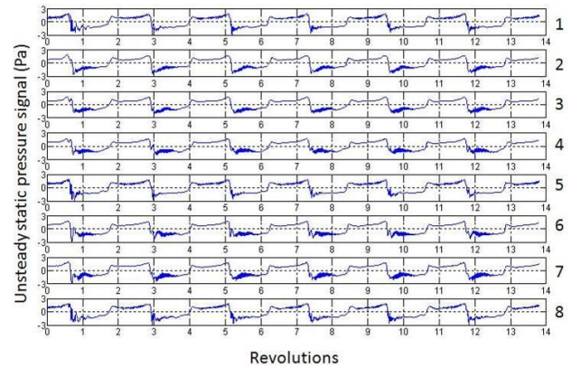
Fig. 6: Unsteady static pressure signal time history from eight numerical sensors on the casing upstream R1 for the nominal case
