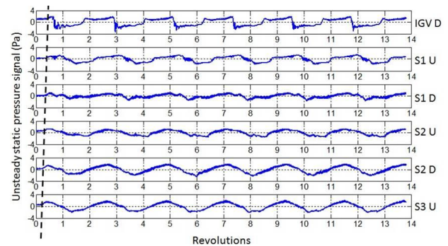
Fig. 8: Unsteady static pressure signal time history from six numerical sensors on the casing in different axial locations for the nominal case (D: Downstream; U: Upstream)
