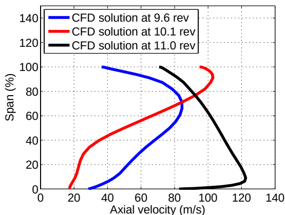
Fig. 9: Instantaneous circumferentially averaged axial velocity radial profile upstream of S3
