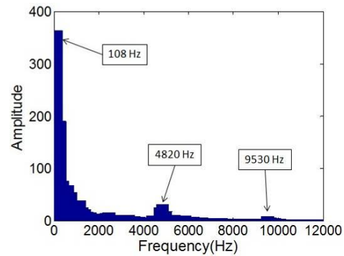
Fig. 7: Fourier transform components from 1 sensor upstream R1
