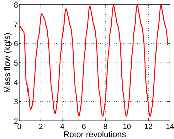
Fig. 5: Mass flow time history for the nominal case
