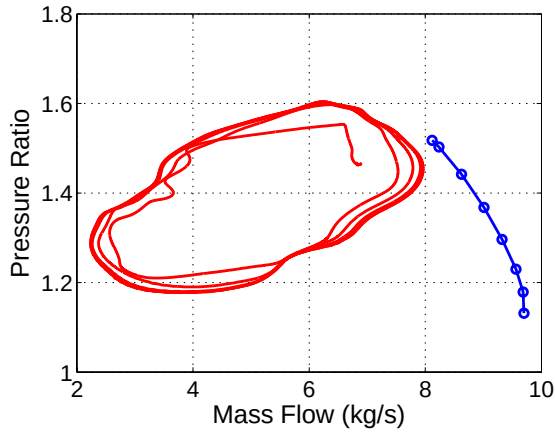
Fig. 4: Overall compressor performance during surge with steady state solution added
