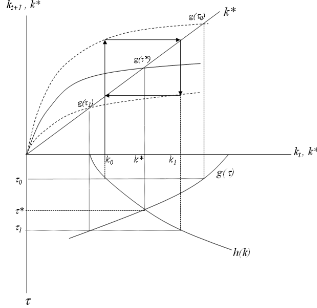
Figure 7: Oscillations around a neoclassical steady state.
