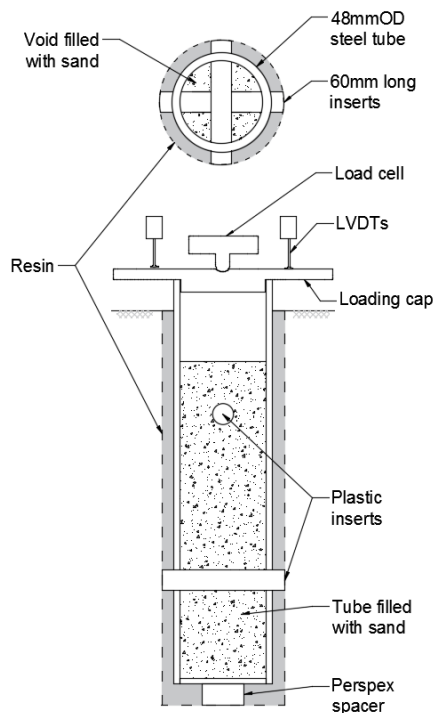
Figure 3. Rough pile geometry and set up
