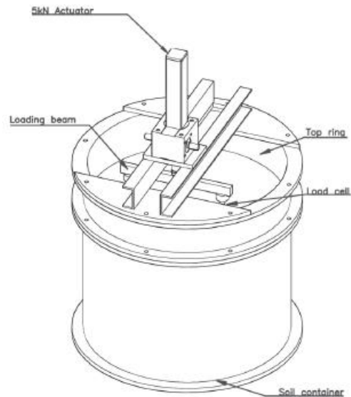
Figure 1. Apparatus set up (Gorasia, 2013)
