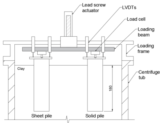
Figure 4. Centrifuge test set up
