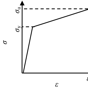
Fig. 13 Linear hardening model for steel material
