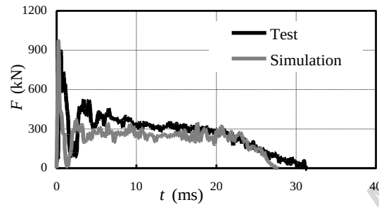
(c) Specimen HW11-56
