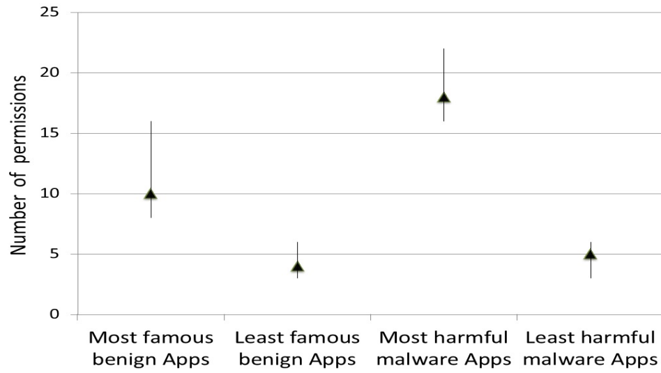
Figure 2: Number of permissions used by malware and benign applications
