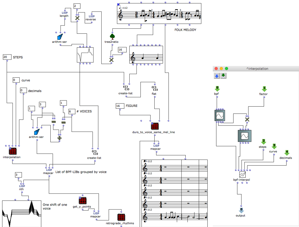
Figure IV.4-13 – Algorithm for rhythm-focusing. The BPFs show the durational contours of melodies. The graph on the lower left corner shows the progressive augmentation for the durations of a given voice. The patch window on the right is the interpolation abstraction.
