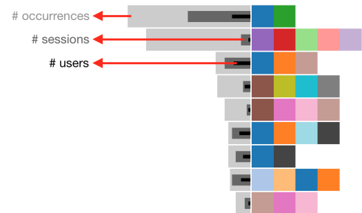
Figure 4: Frequent activities. Each row represents an activity. The right part indicates its sequence of actions with colour-coded squares representing action types. The left part shows three statistic values of the activity: the number of times it appears, the number of sessions it appears in, and the number of users performing it.
