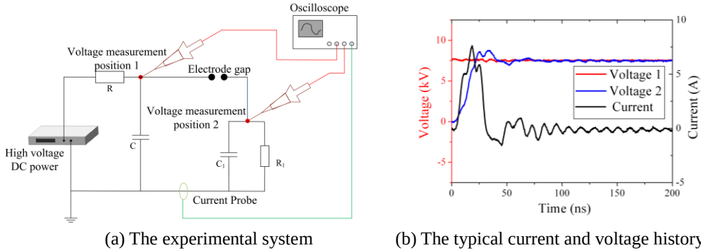
Figure 3. The special discharge circuit experiment
