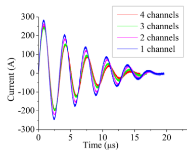
Figure 15. The discharge current waveform
