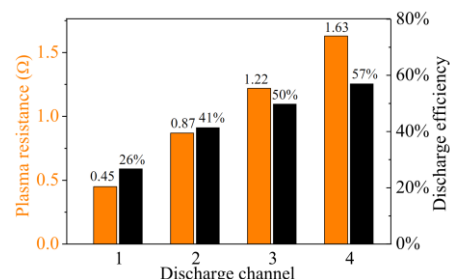
Figure 16. The plasma resistance and discharge efficiency for discharge with different channel number
