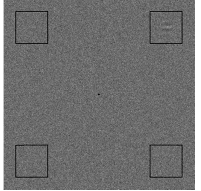
Fig. 3. Stimulus geometry used in the experiment. Gabor and noise contrasts have been adjusted for illustrative purposes.
