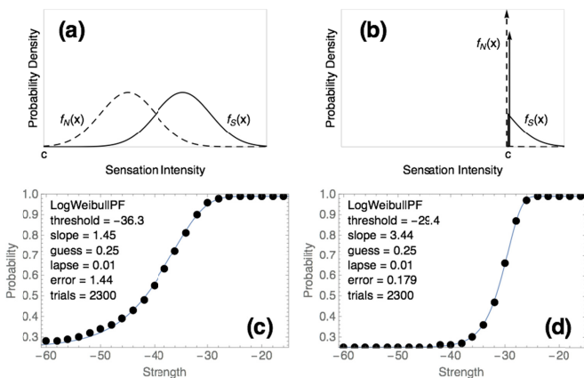
Fig. 1. Representative densities (with \mu_S = \mu_N + 2\sigma_N ) for 4AFC detection target S and non-target N (a, b) and corresponding psychometric functions (c, d) with a high sensory threshold ( c = \mu_N + 3\sigma_N ; b, d) and a low sensory threshold ( c = \mu_N - 3\sigma_N ; a, c). Arrows in (b) represent delta functions, indicating high probability density at the sensory threshold c . Insets in panels (c) and (d) describe best-fitting Weibull distributions (smooth curves) to the model-derived accuracies (filled circles).
