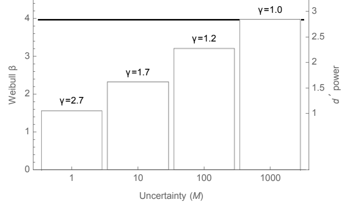
Fig. 6. Model performances with best-fitting values of \gamma (indicated on the figure), b , and N_a for various fixed values of uncertainty M . All other model parameters were fixed at the baseline values, described in Section 3. The solid horizontal line shows the median values for Weibull \beta obtained in detection experiments. (In noise, the median was 4.2; in the absence of noise, it was 3.9. Geometric means were greater: 5.3 and 5.0, respectively. Arithmetic means were even greater.)
