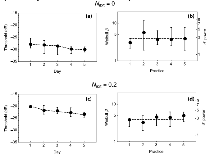
Fig. 5. Values for threshold (a, c) and slope (b, d) from Weibull fits to empirical data from detection (a, b) and detection-in-noise (c, d) conditions. Each symbol illustrates the median value, across 9 observers, \pm 1 quartile. Dashed curves illustrate a model fit. Parameter values were: \delta = 0.01, K = 1, M = 870
