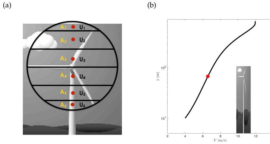
Figure 4. (a) Schematic to represent the calculation of the equivalent rotor wind speed, (b) mean wind profile computed using the values of y_0 and d for a given rough surface assuming a reference speed of 4 m/s at a height of 10m above ground. The red dot marks the hub velocity (at the hub height) in the profile.
