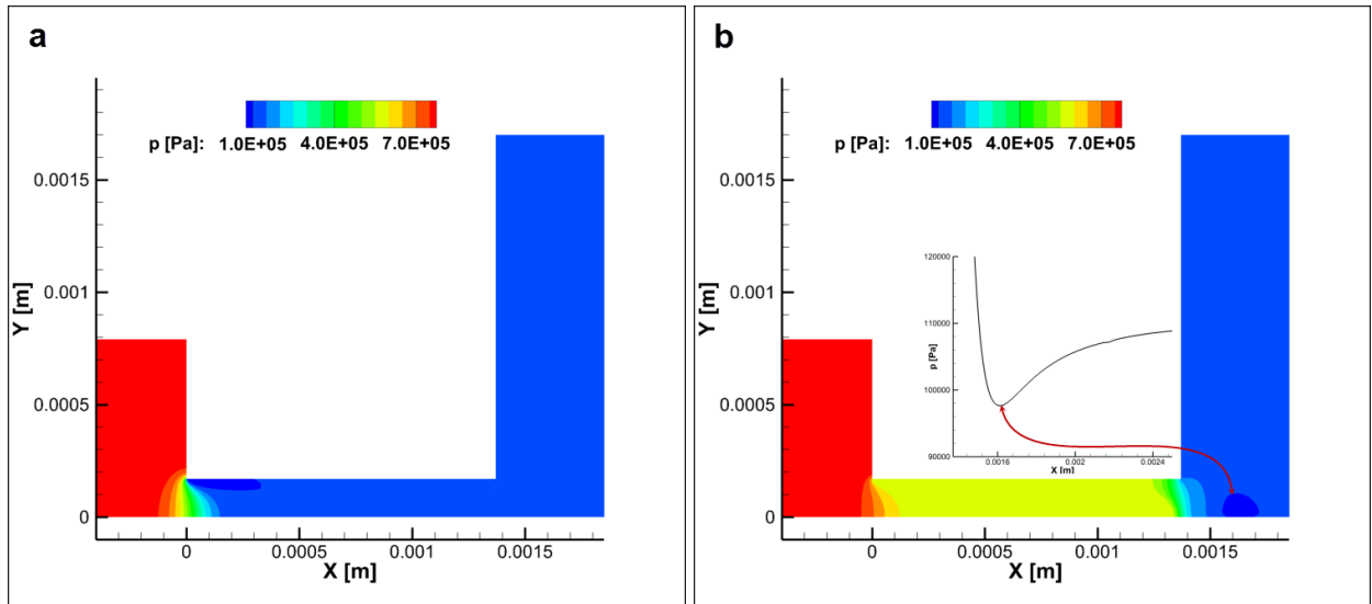
Fig. 9 Pressure distribution (ZGB model, R_b=1.0 \cdot 10^{-6} \text{ m} ): (a) T=370\text{K} ( p_{\text{sat}}=90540\text{Pa} ) and (b) T=430\text{K} ( p_{\text{sat}}=570260\text{Pa} ).
