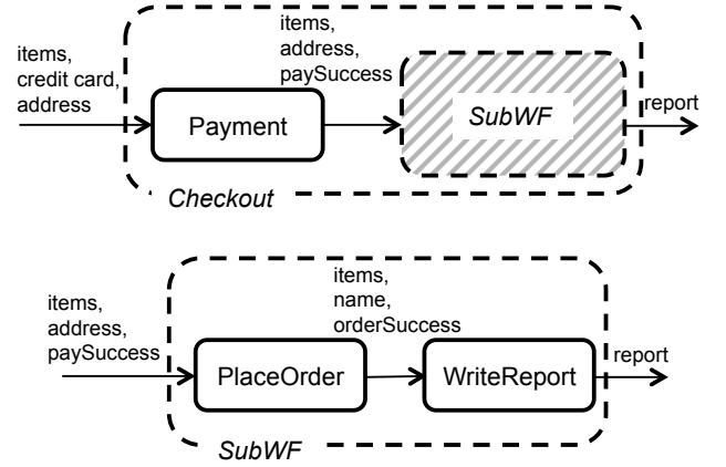
Fig. 4. The inference process on the sub-workflows of Checkout SBS process workflow.
