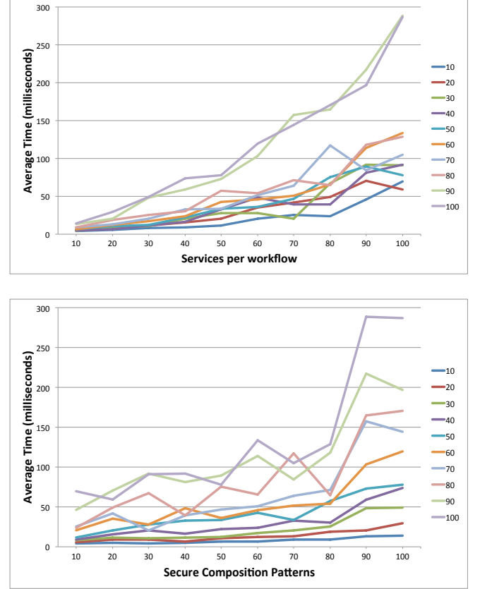
Fig. 7. Average VT_s for different workflow and SCO pattern set sizes
