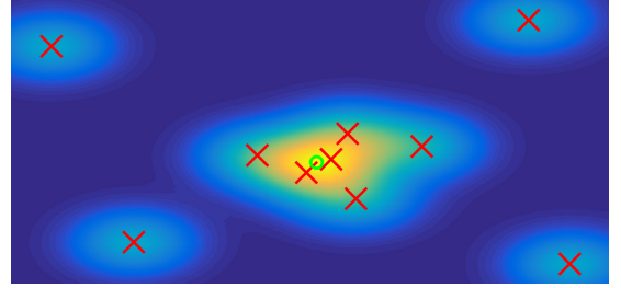
Figure 8: KDE: The heat map denotes the confidence of the aggregated probability distribution p(\mathbf{d}_{1_{out}}) . Red crosses indicates the positions of the input \mathbf{d}_{1_{in}} vector and green circle represents the maxima of p(\mathbf{d}_{1_{out}}) and output vector \mathbf{d}_{1_{out}} .
