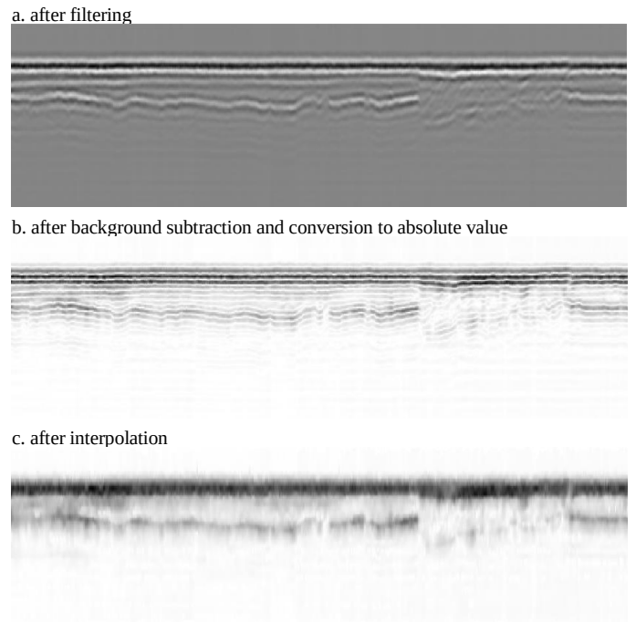
Figure 4. GPR processing example: pre-processing stage (B-scan)
