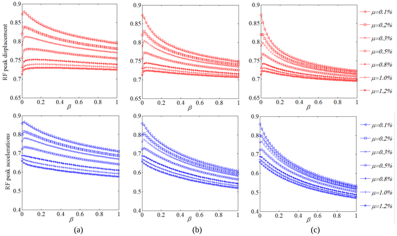
Fig. 4. Peak top floor displacement (upper panels) and acceleration (bottom panels) of TMDI equipped primary structure for different inertia ratio, \beta , and attached mass ratio, \mu , values normalised by the corresponding peak values of the uncontrolled structure for TMDI topologies (a) “-1”, (b) “-2”, and (c) “-3”.
