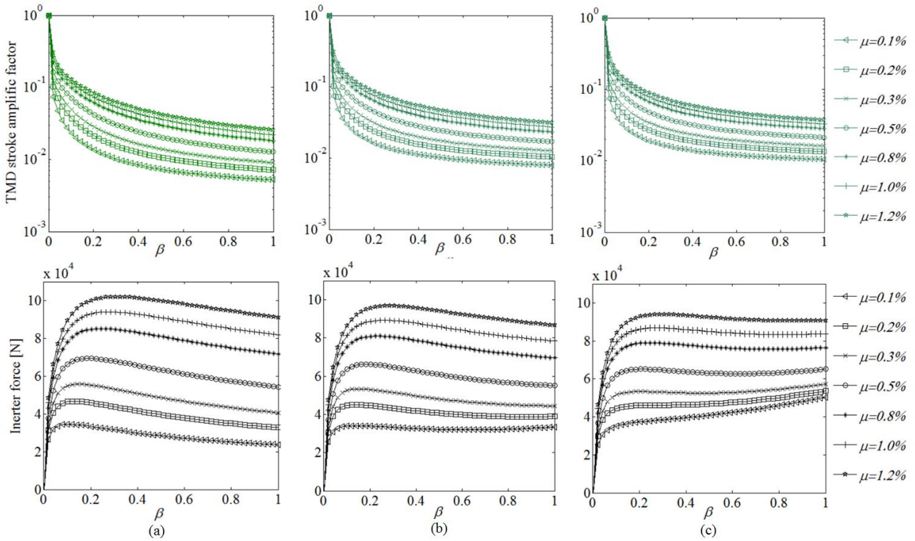
Fig. 5. Peak TMDI attached mass displacement over peak TMD attached mass displacement (upper panels), and peak inerter resisting force (lower panels) for different values of inertia ratio \beta and attached mass ratio \mu for TMDI topologies (a) “-1”, (b) “-2”, and (c) “-3”.
