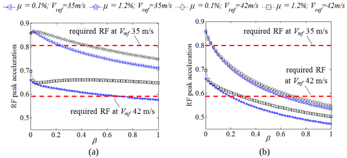
Fig. 7. Peak top floor acceleration of TMDI-equipped primary structure for different inertance ratio, \beta , and attached mass ratio, \mu , values normalised by the corresponding peak values of the uncontrolled structure for two different design V_{ref} values and for TMDI topologies (a) “-1” and (b) “-3”.
